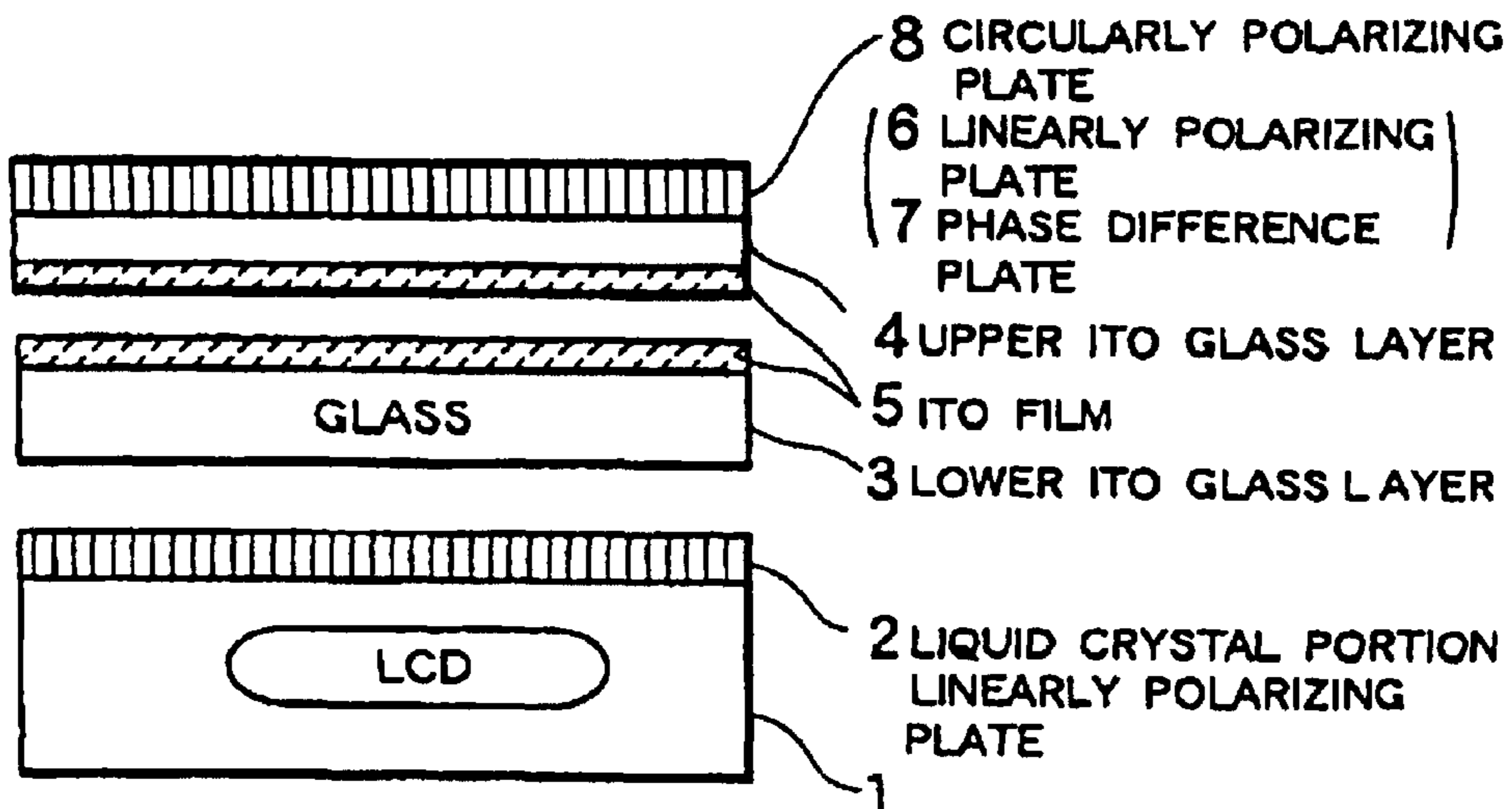
FIG.12 PRIOR ART
