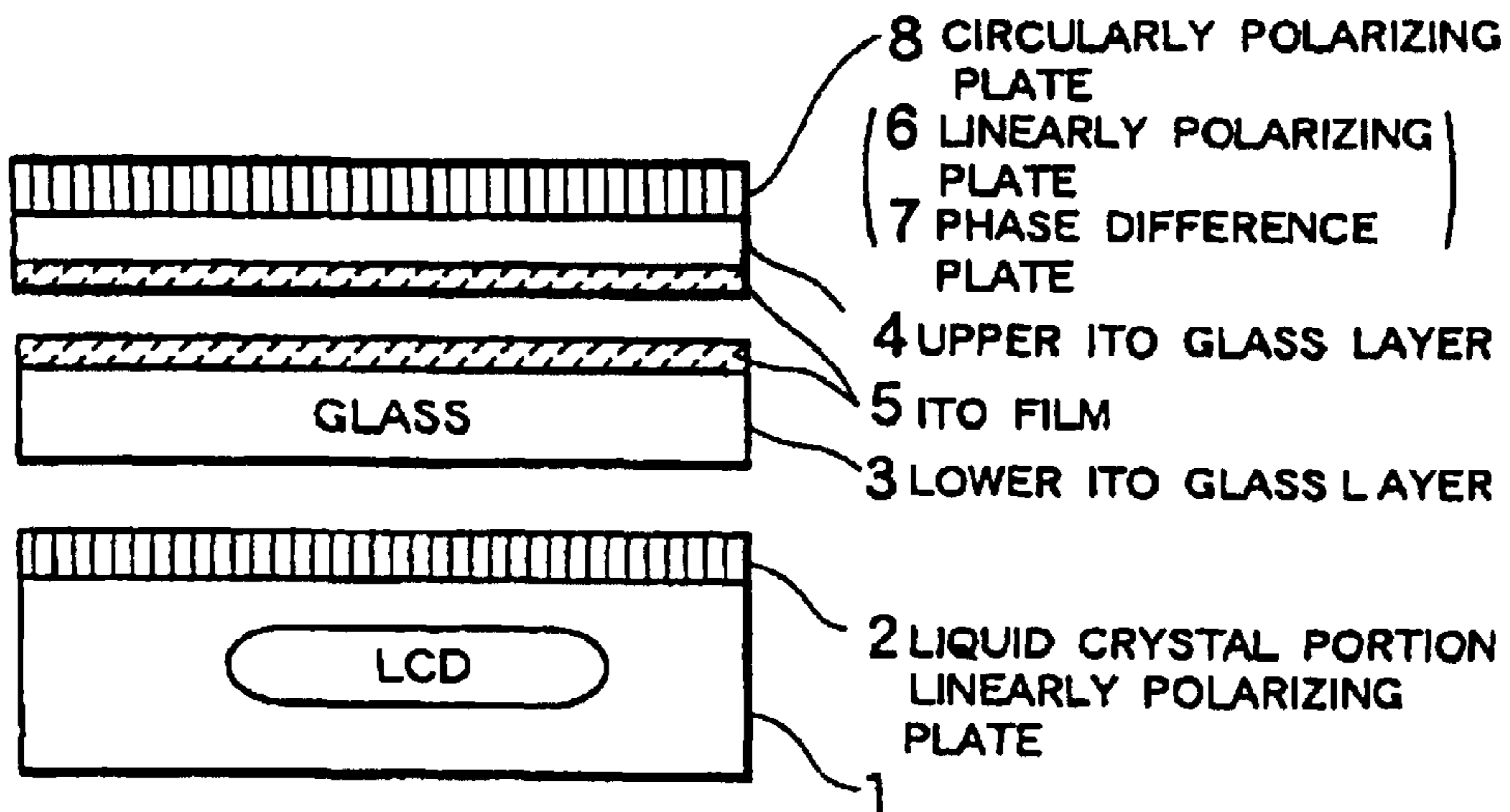
FIG.12 PRIOR ART
