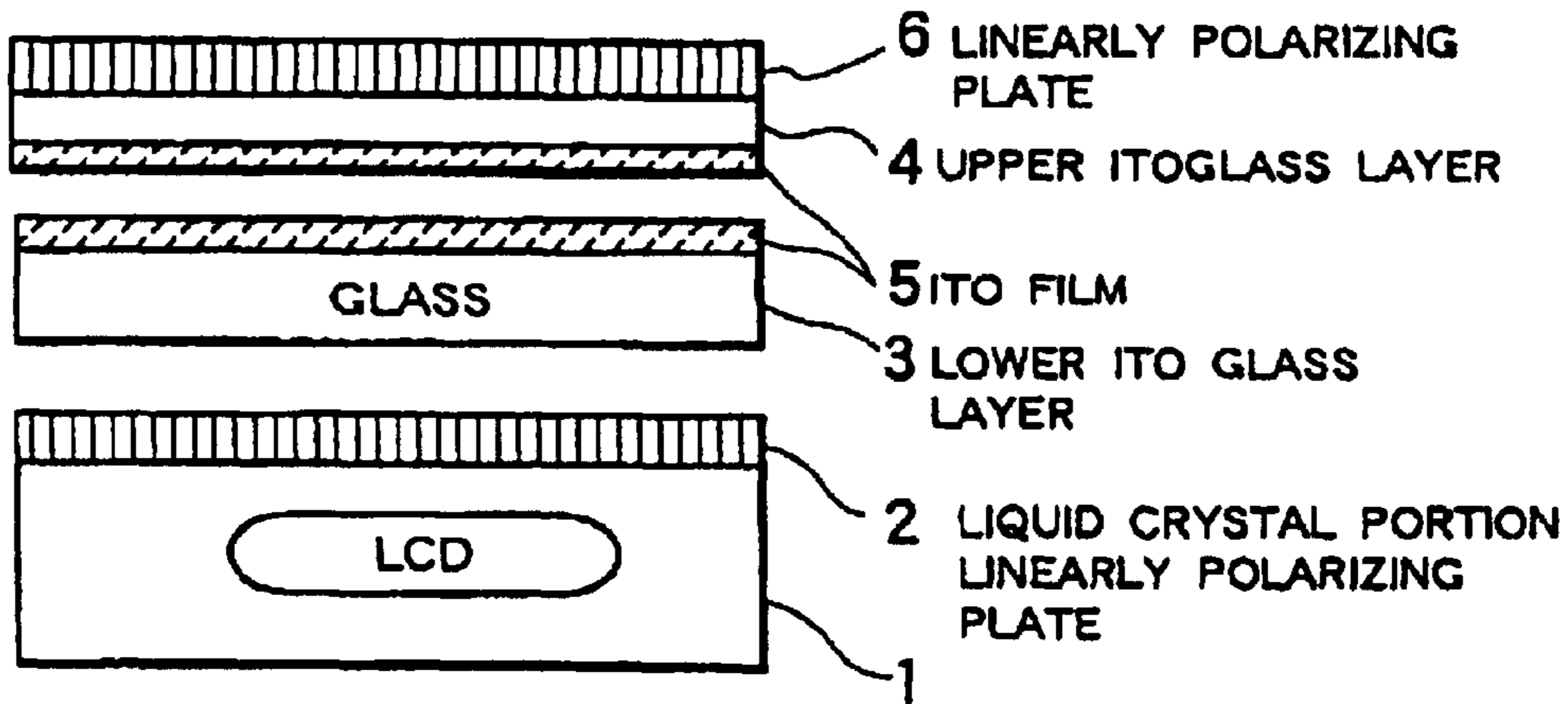
FIG.12 PRIOR ART
