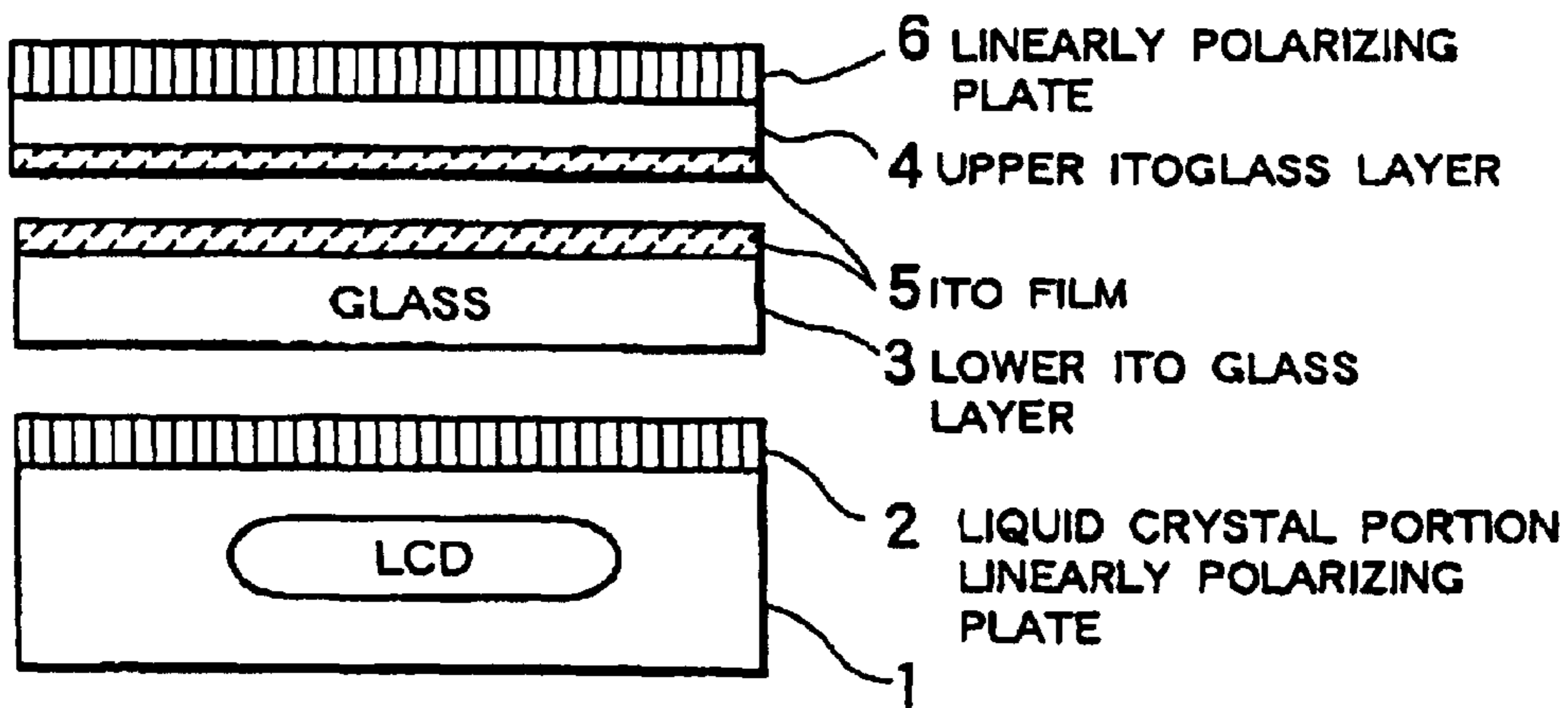
FIG.12 PRIOR ART
