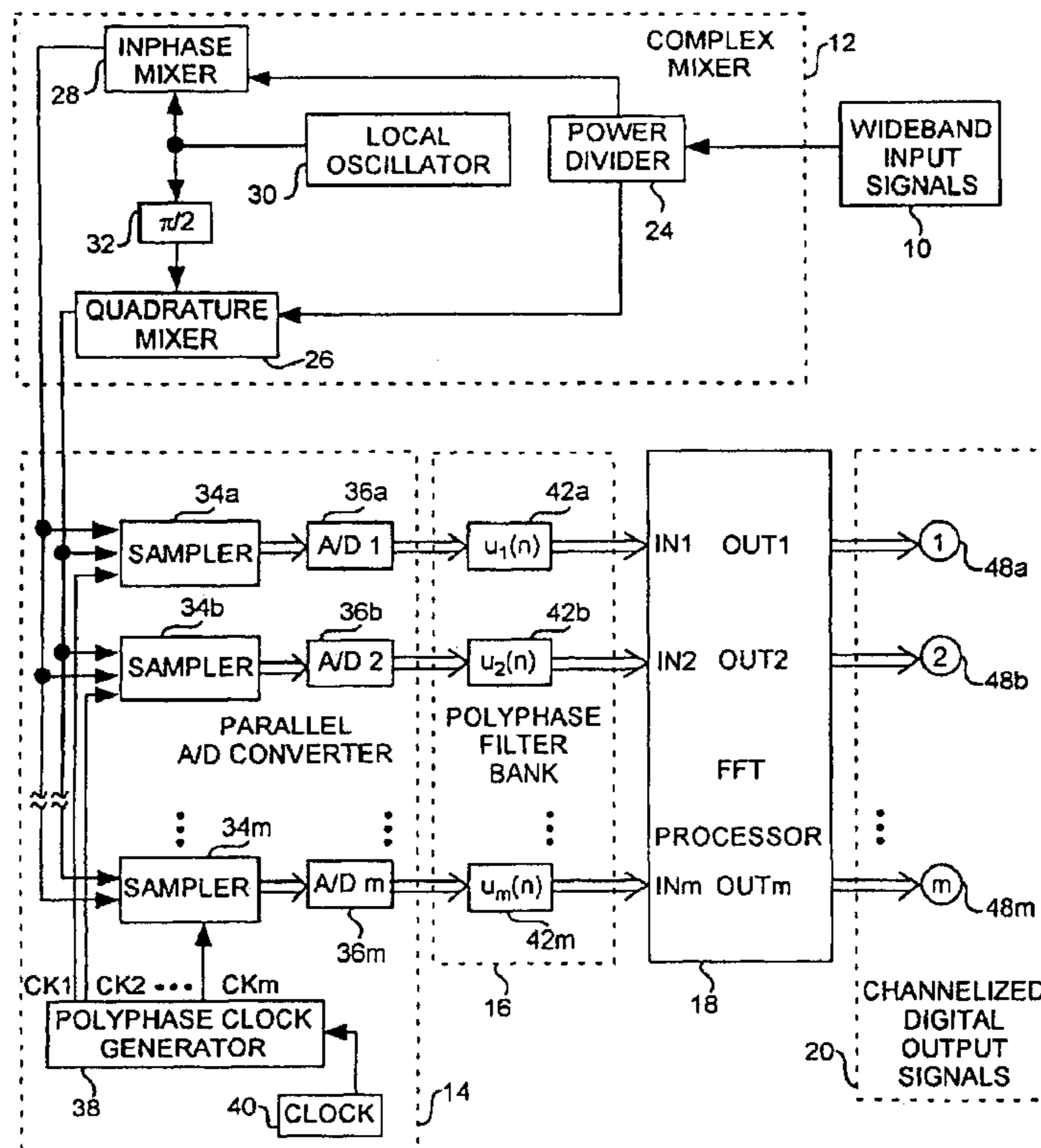
POLYPHASE CHANNELIZER
