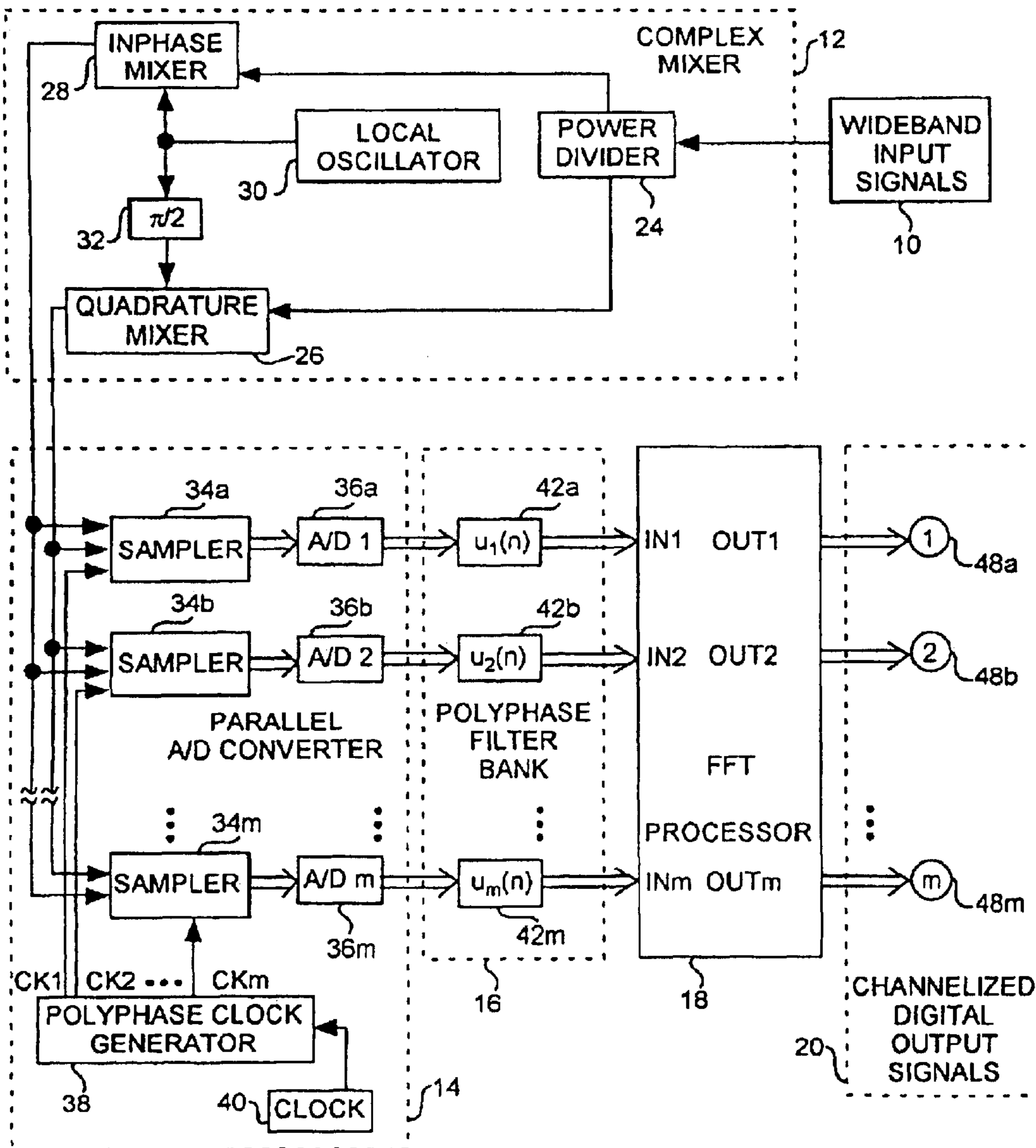
POLYPHASE CHANNELIZER
