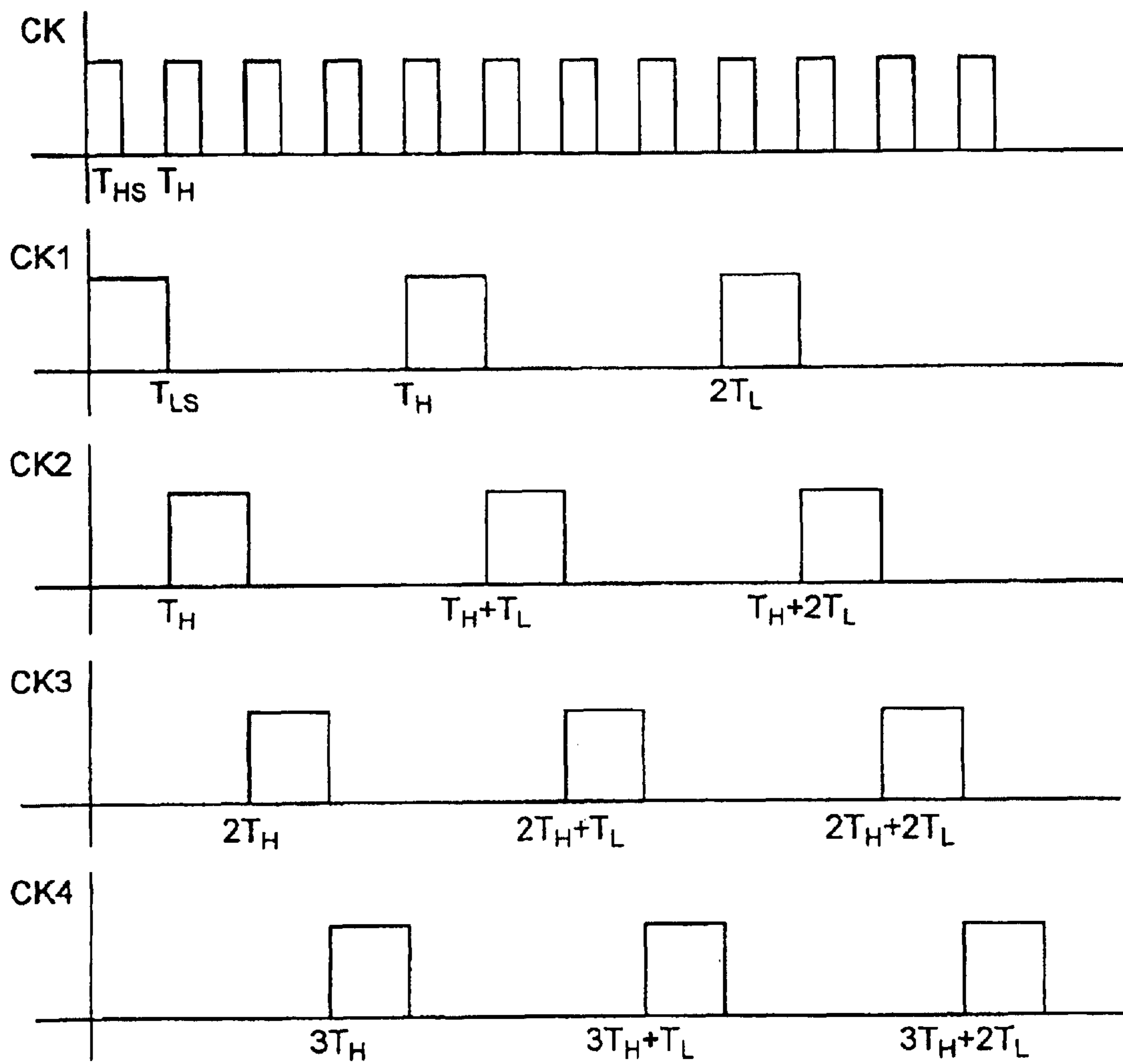
POLYPHASE CLOCK TIMING DIAGRAM ( m = 4 )
