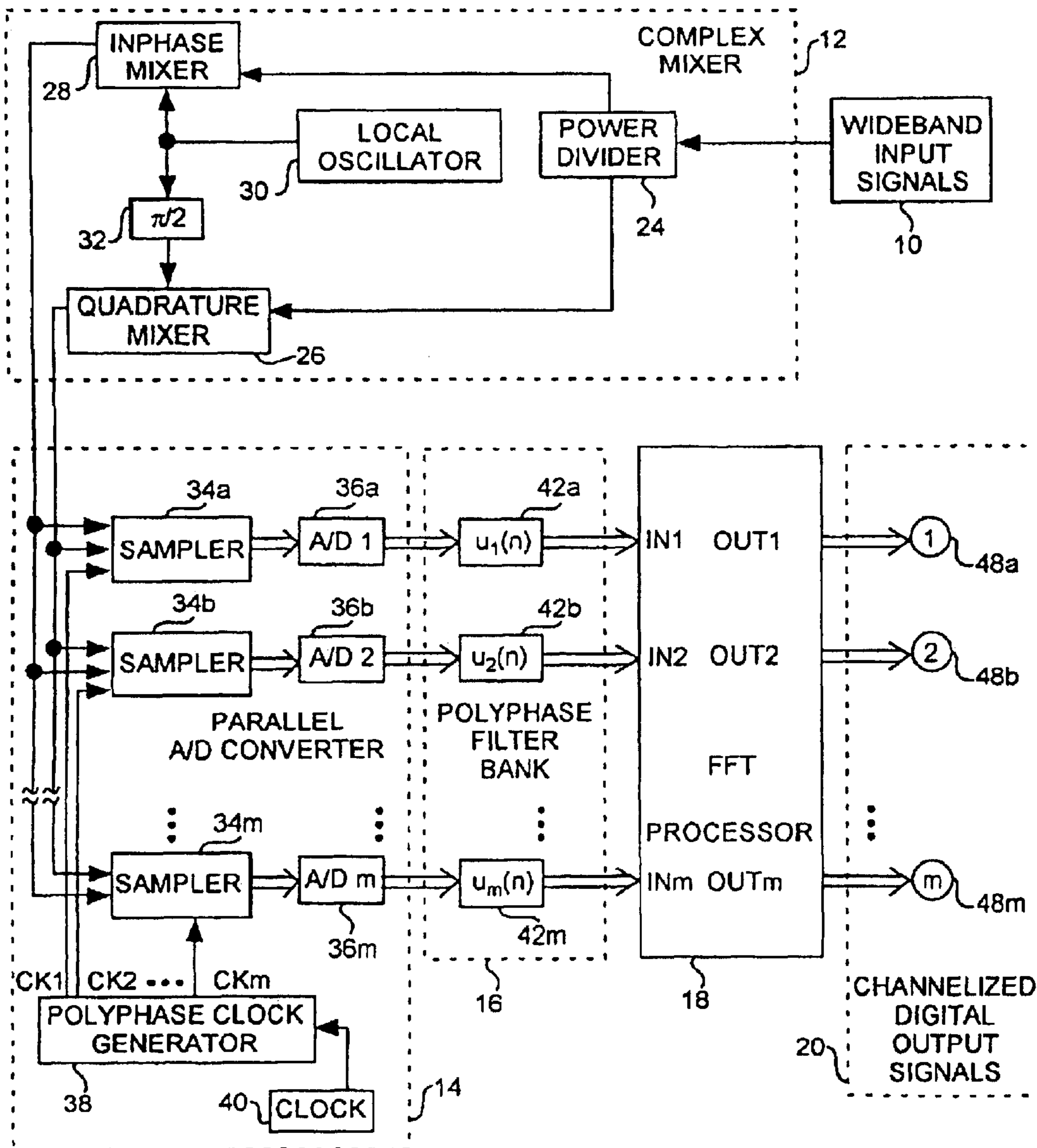
POLYPHASE CHANNELIZER
