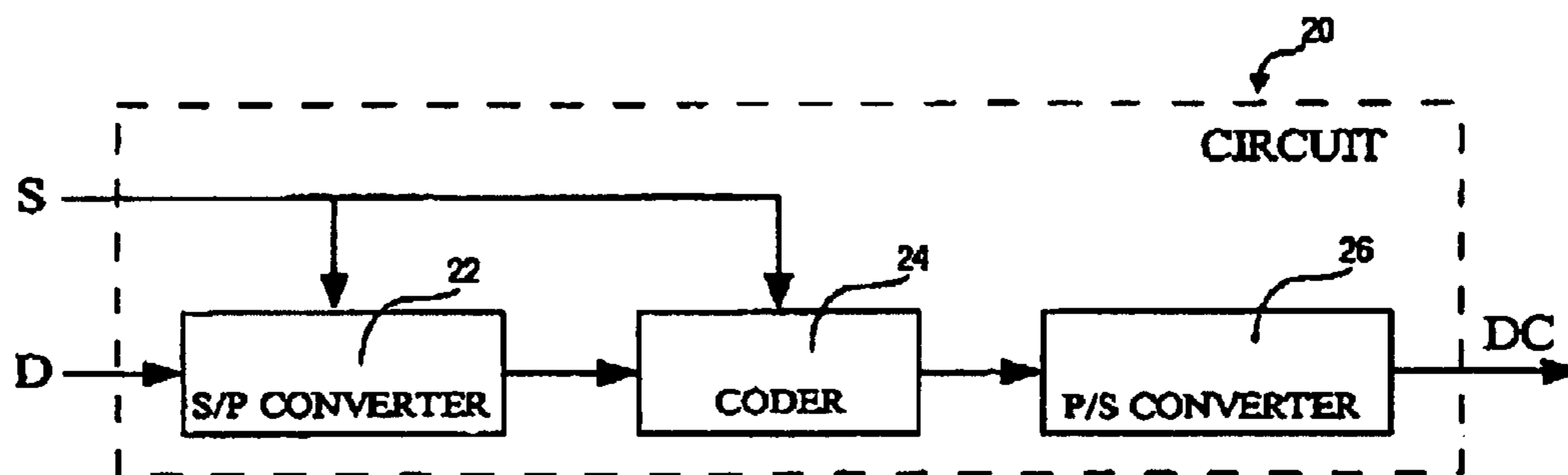
FIG. 2 PRIOR ART
