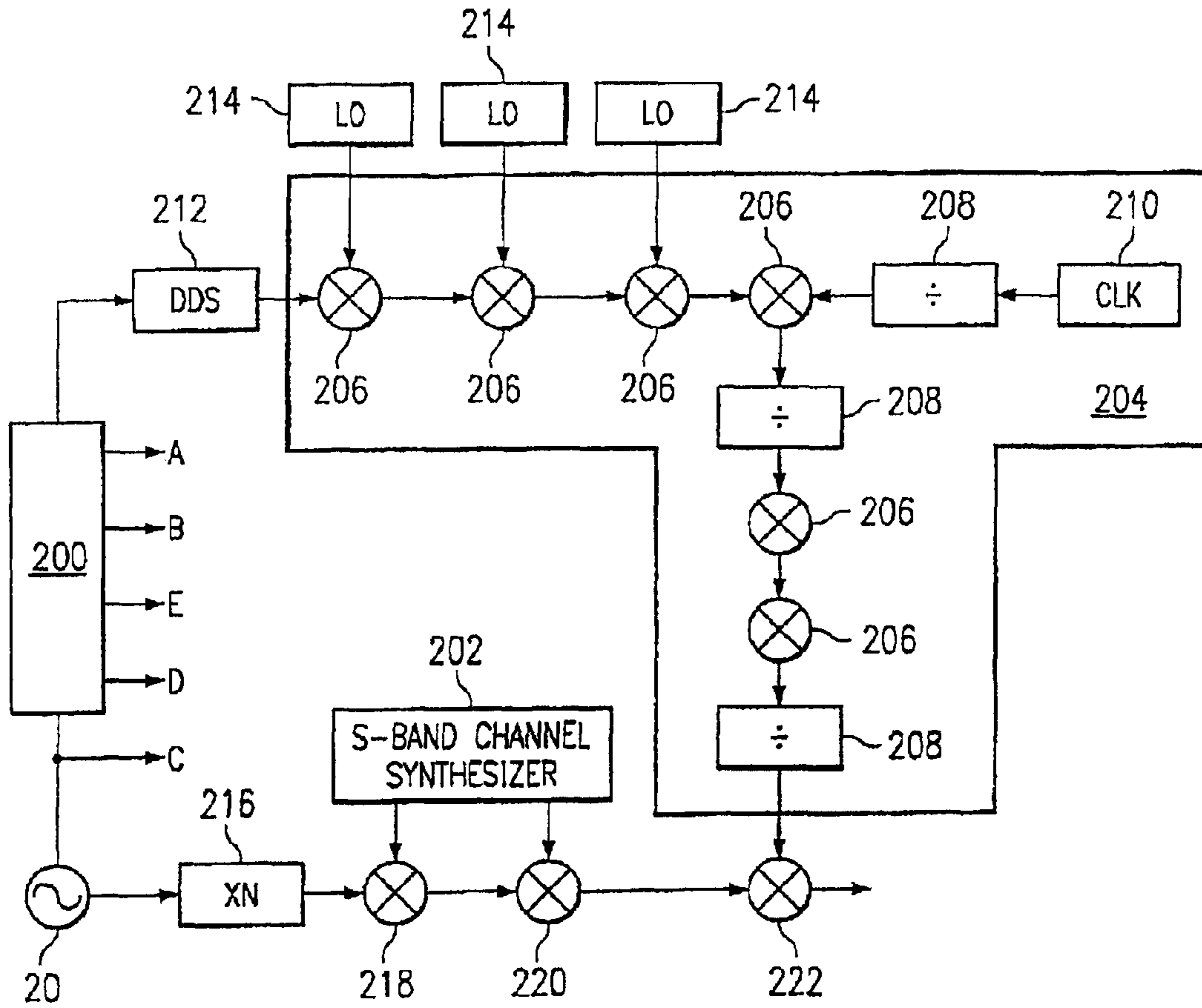
FIG. 5 (PRIOR ART)
