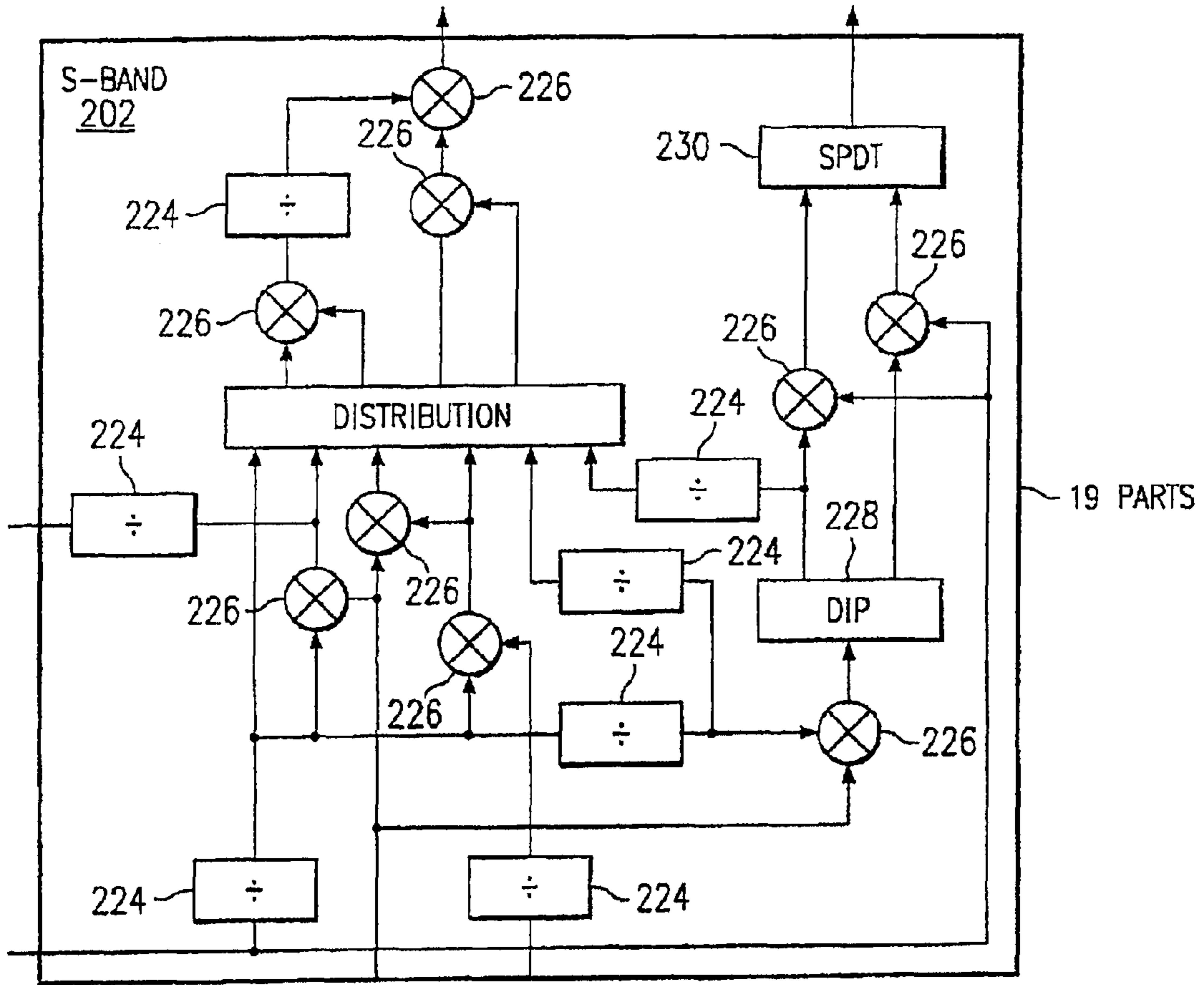
FIG. 6 (PRIOR ART)
