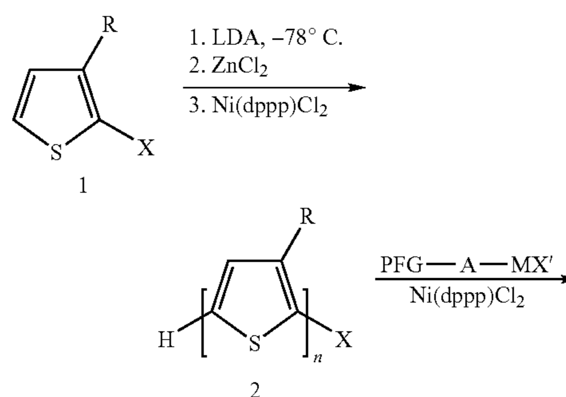
Scheme 1. Synthesis of regioregular head-to-tail poly(3-[alkylthiophenes] alkylthiophenes with one functional end group.
