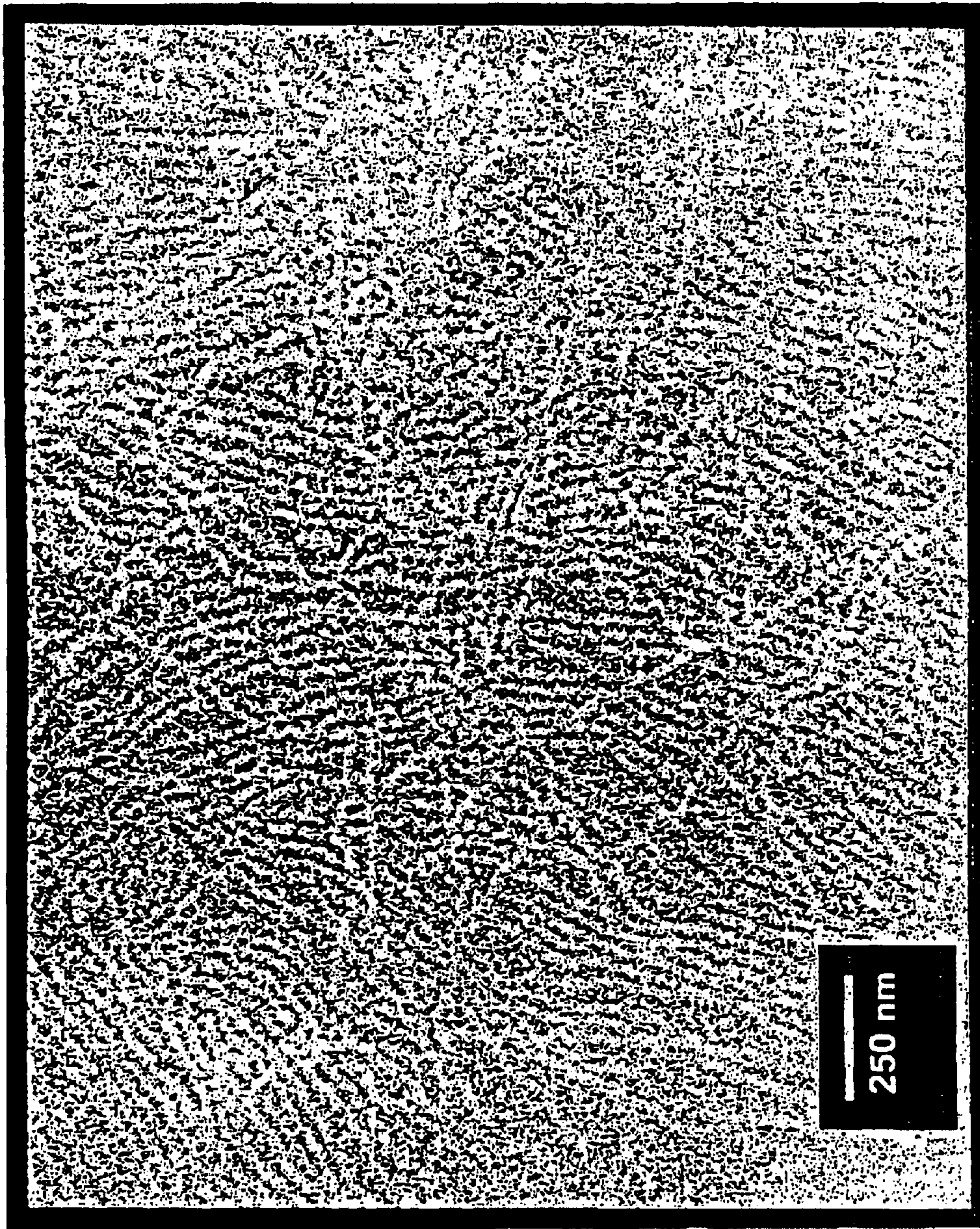
FIG. 6 TEM confirms the present of "nano-wire" network in the solid film of a HT-PHT-block-PMA diblock copolymer
