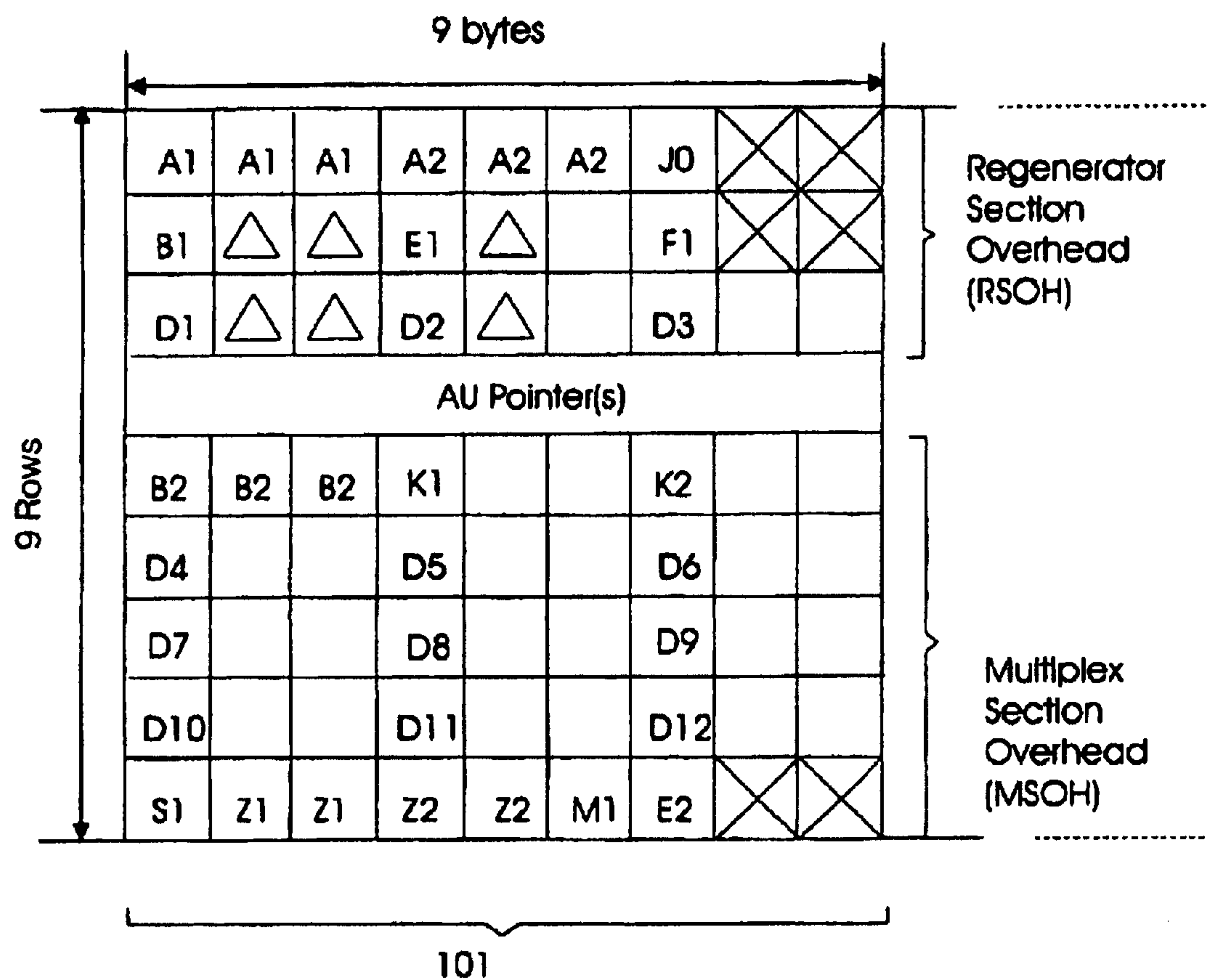
Fig. 3 (Prior Art)
