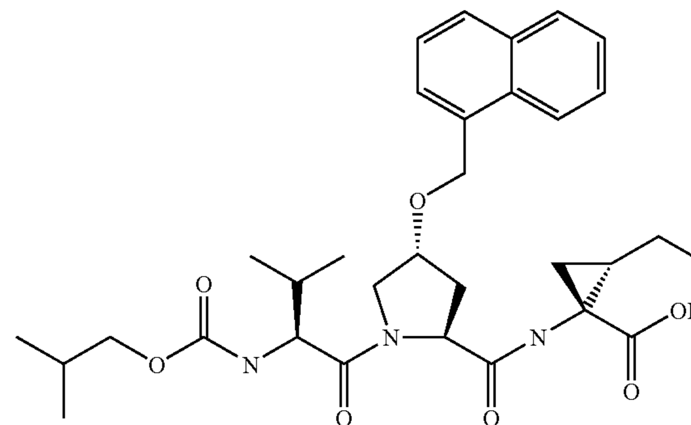
Synthesis of compound 302
