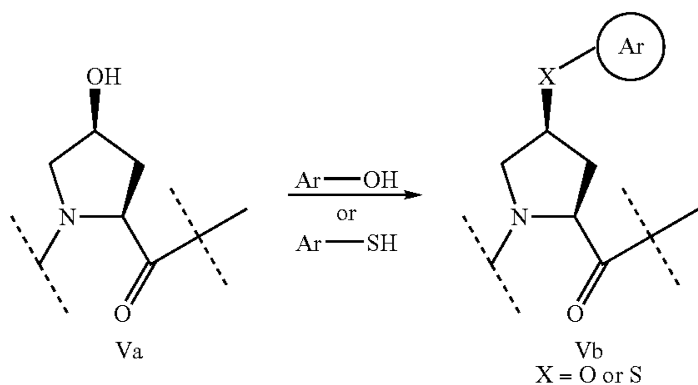
SCHEME V
