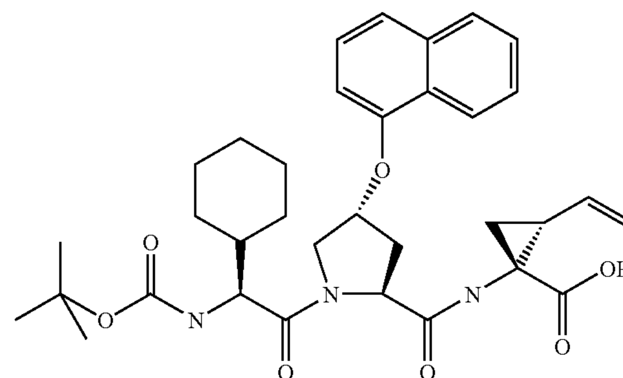
Synthesis of compound 308
