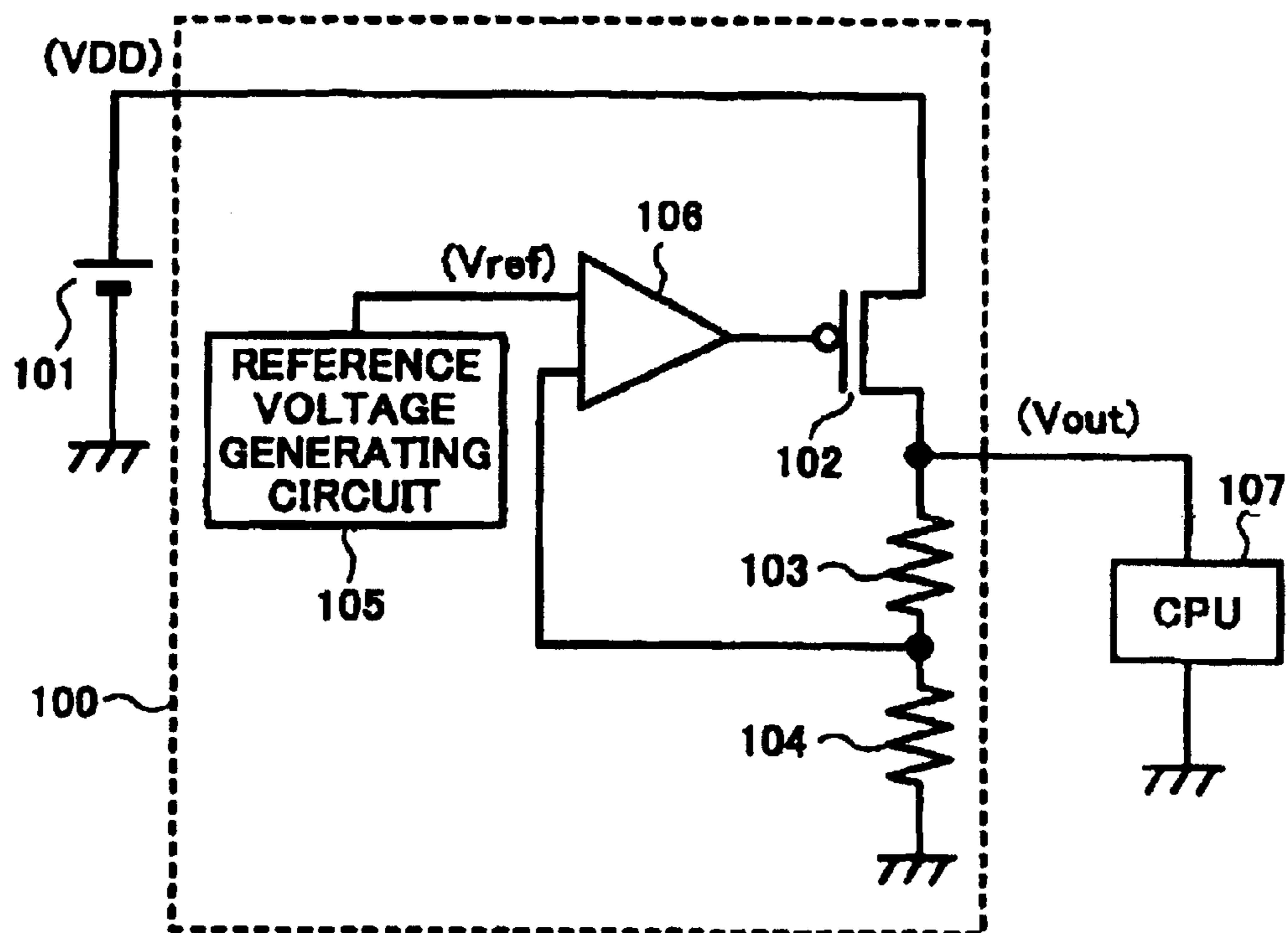
FIG. 1 PRIOR ART
