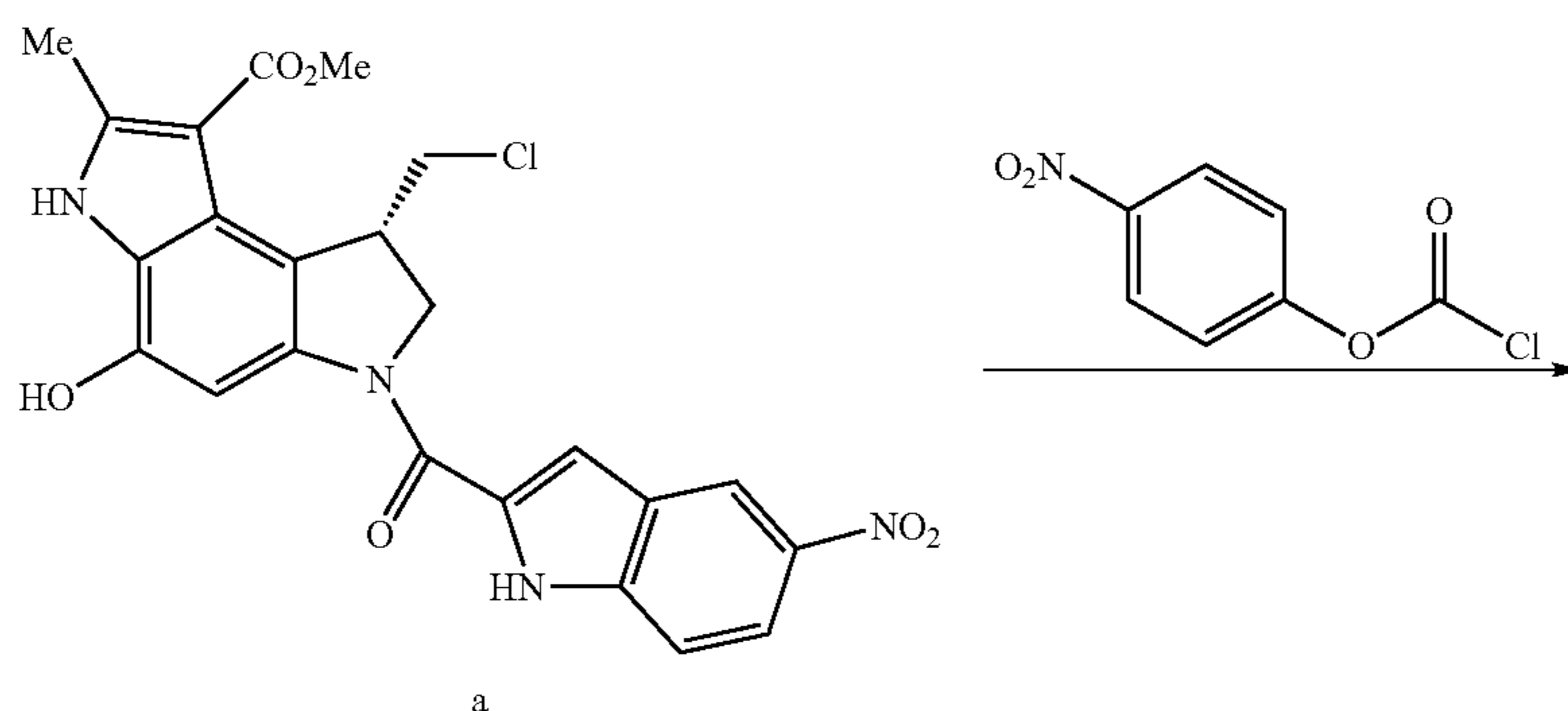
Scheme 7
