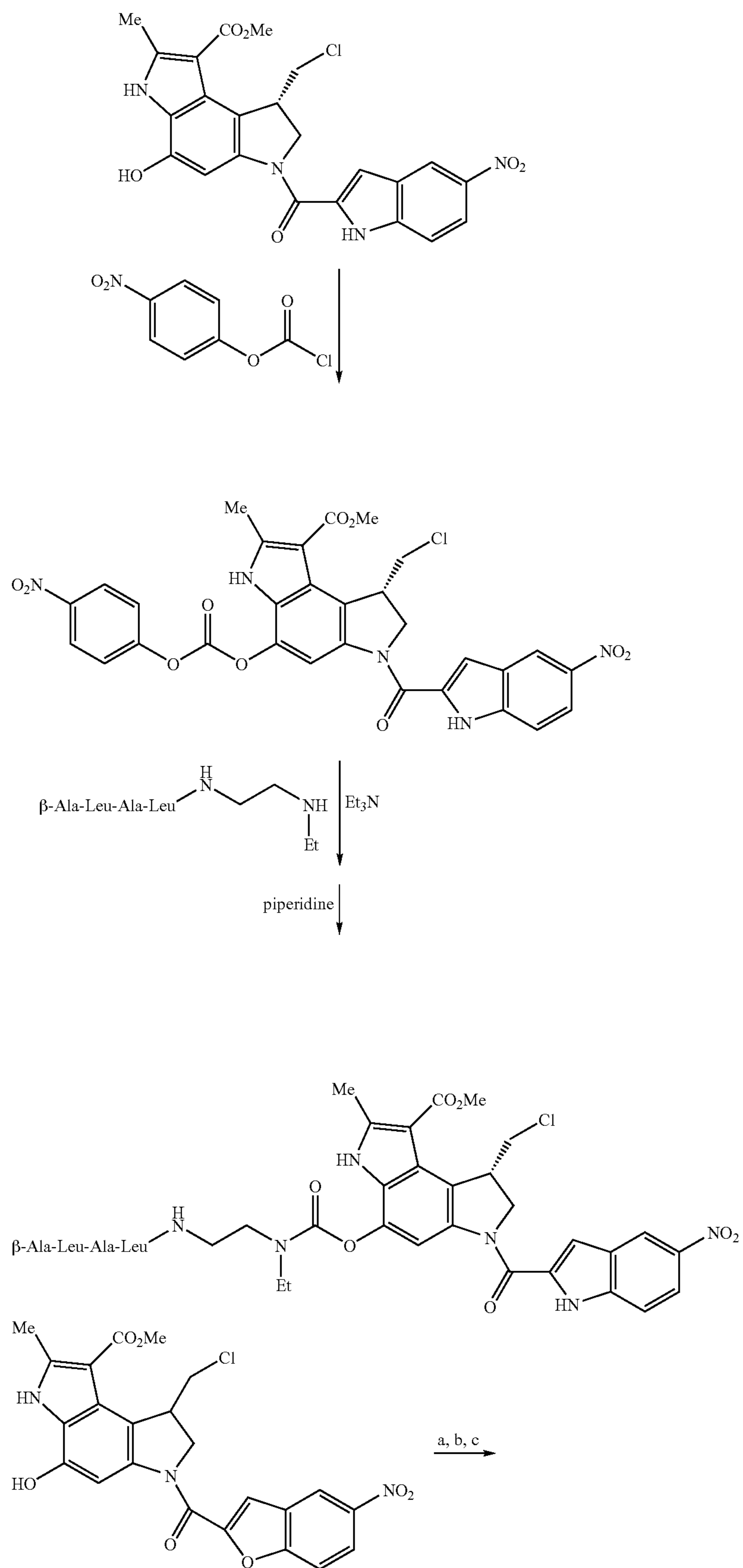
Scheme 4
