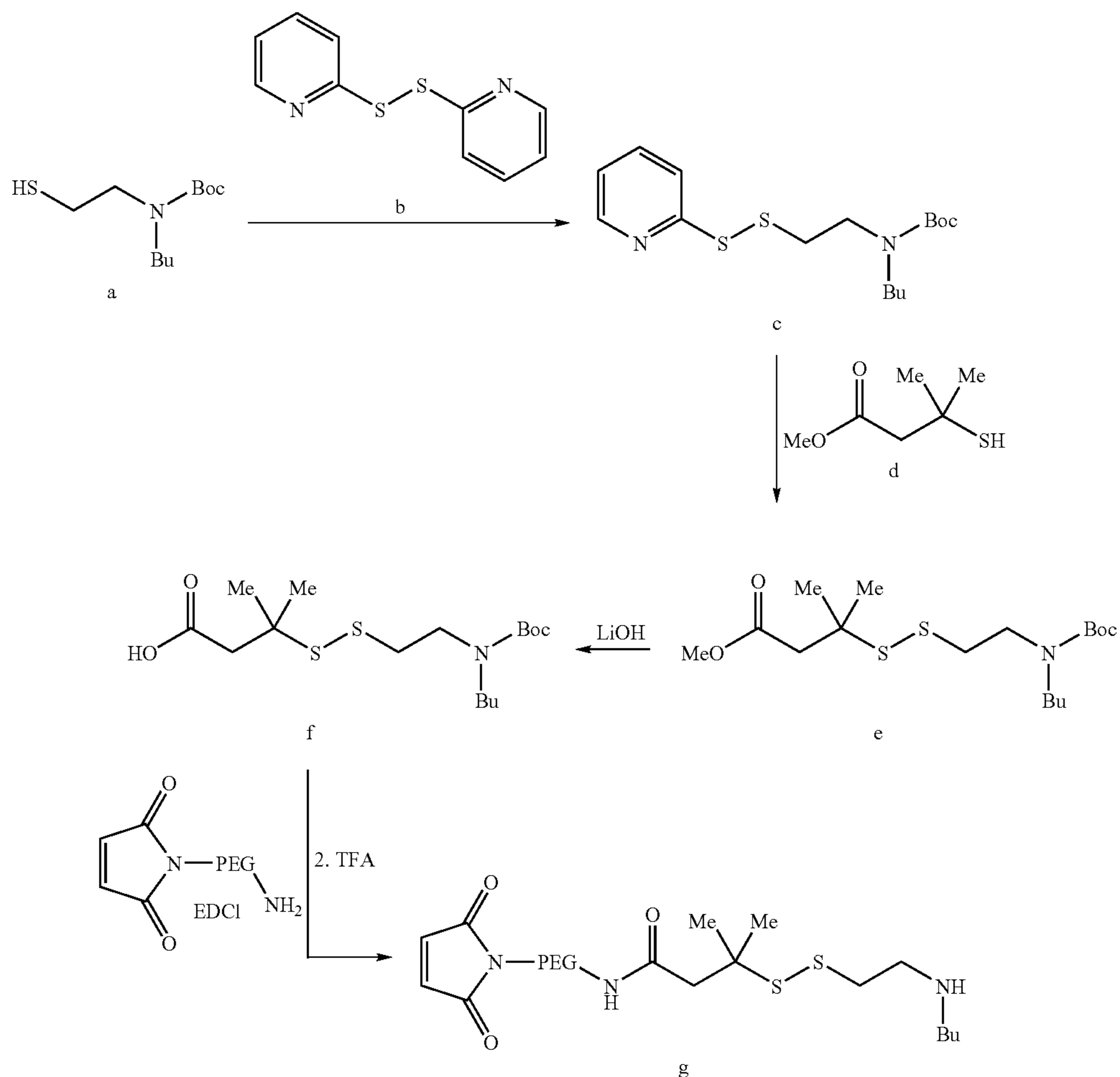
Scheme 5
