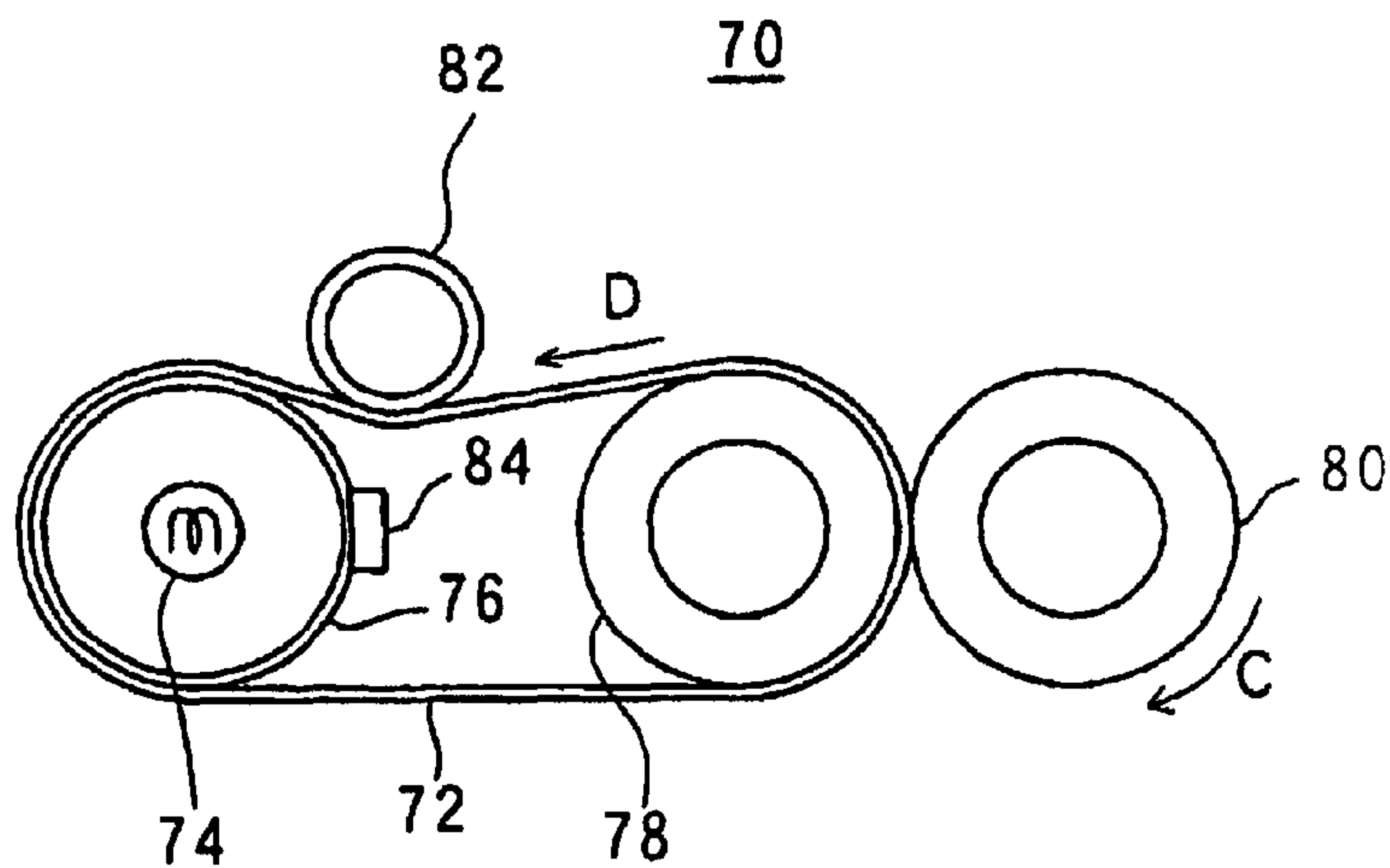
Fig.4 PRIOR ART
