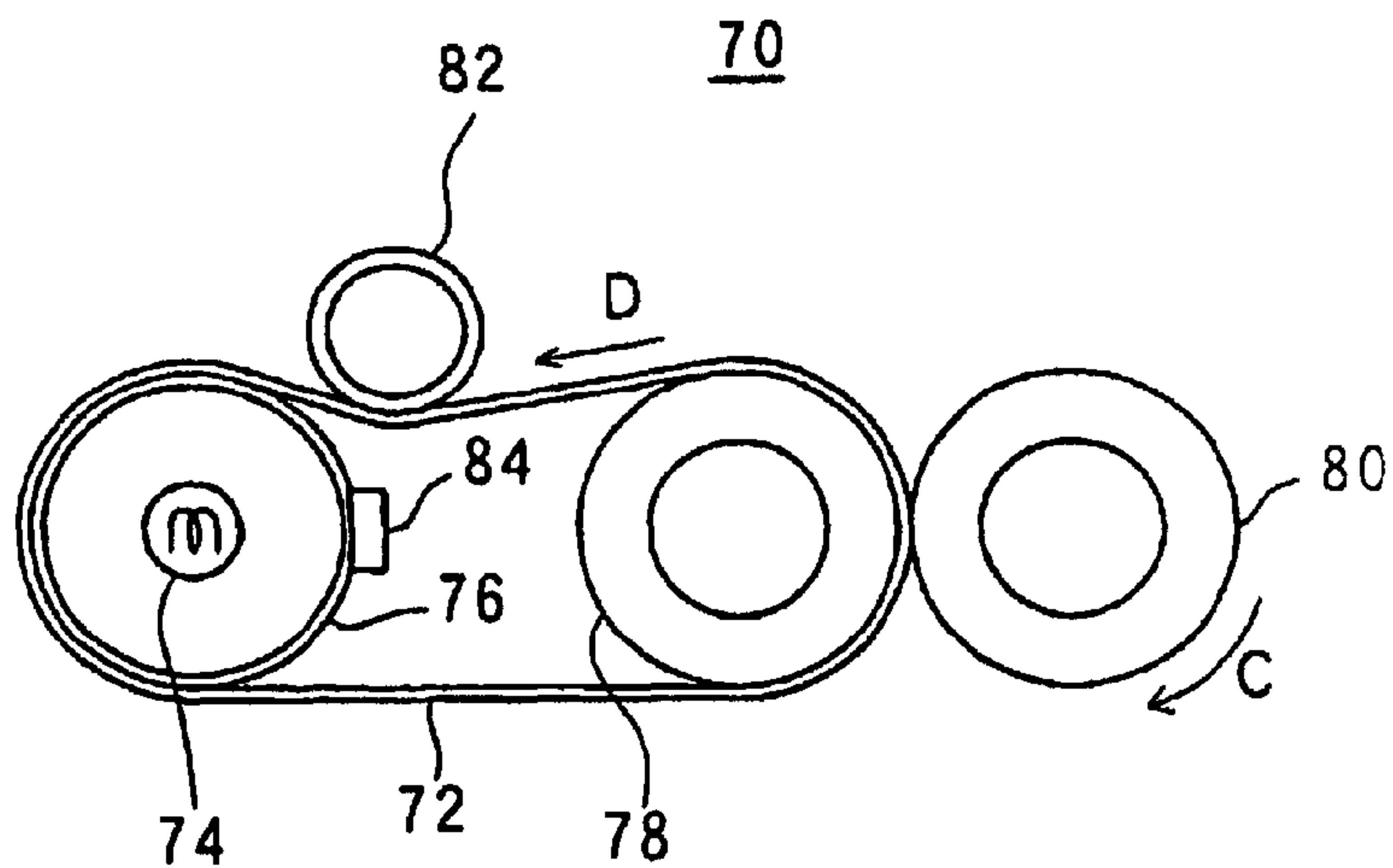
Fig.4 PRIOR ART
