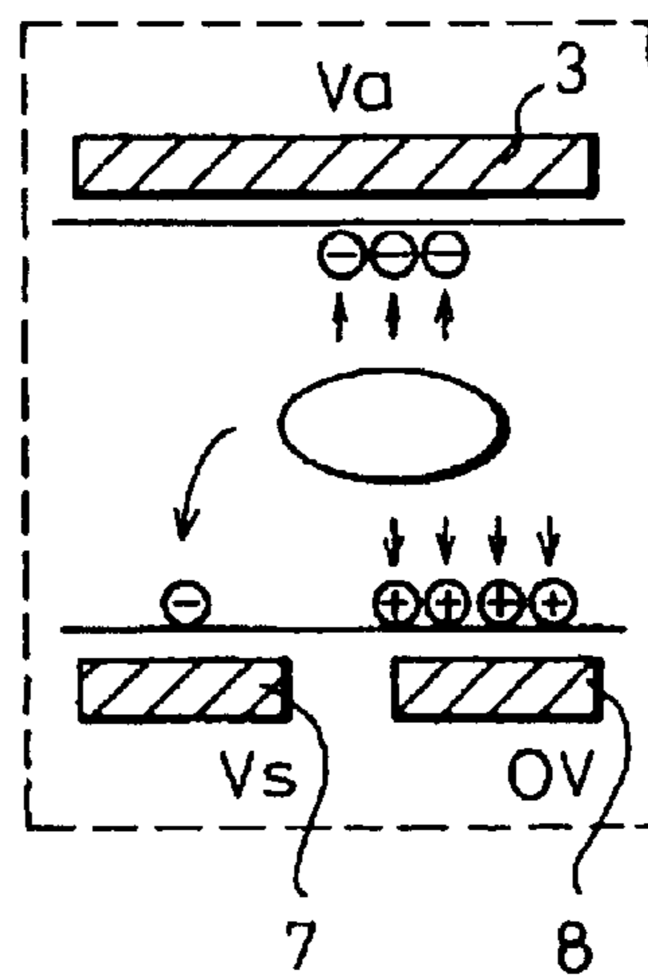
Fig.5D (PRIOR ART)
