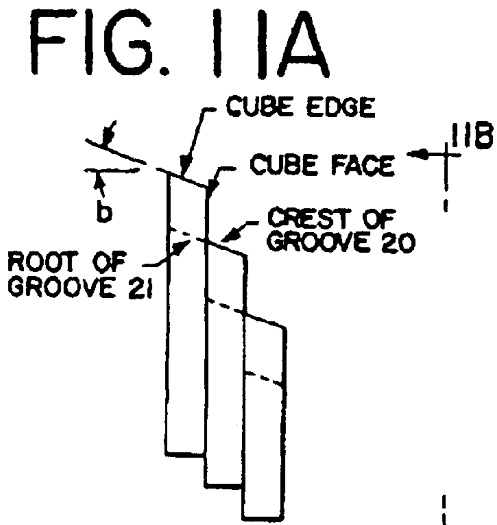
FIG. 11 PLATE ANGLE HIGHLY EXAGGERATED
