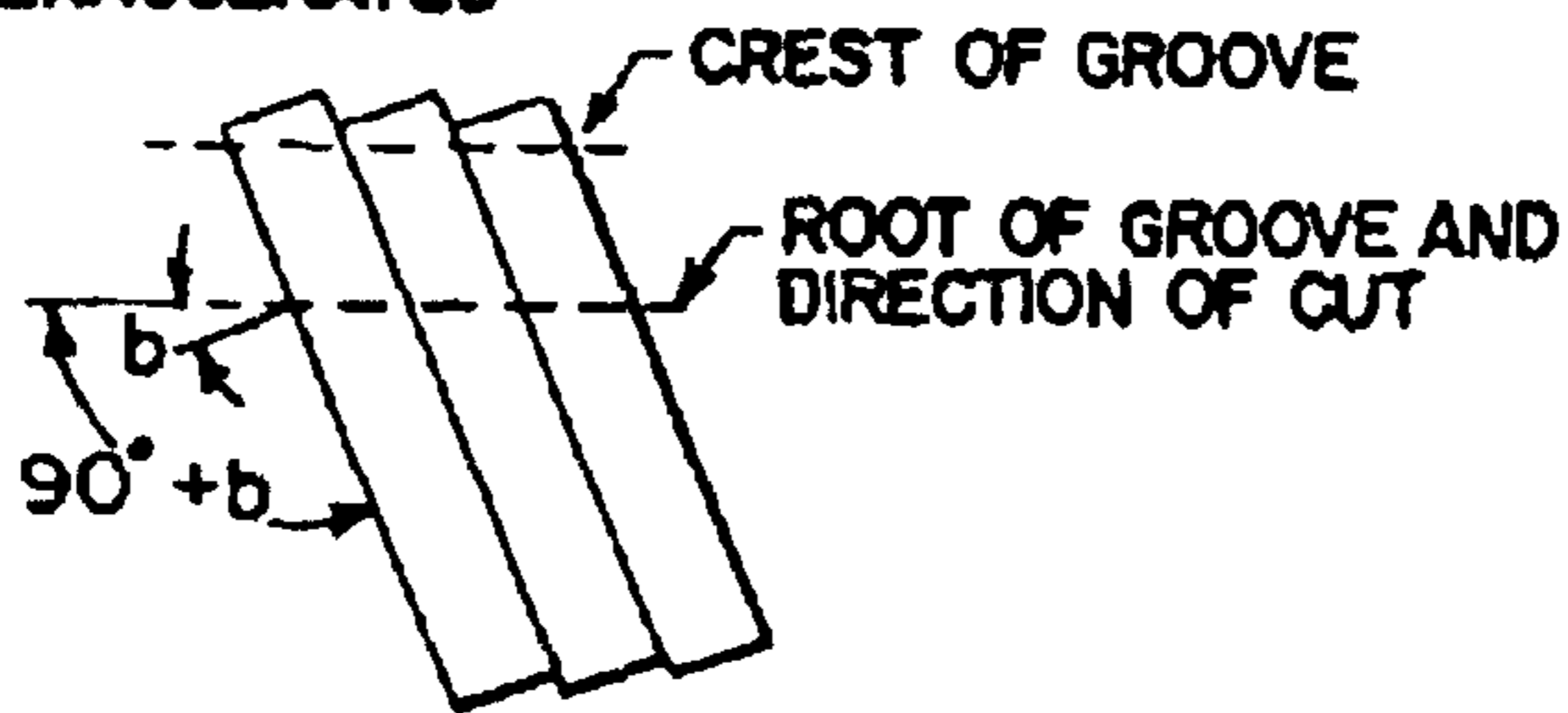
FIG. 11 PLATE ANGLE HIGHLY EXAGGERATED
