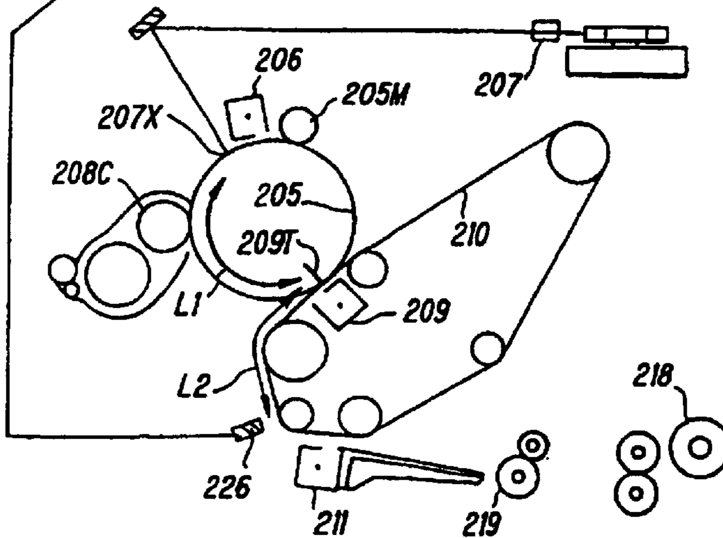
OPERATION OF IMAGE FORMING SECTION
