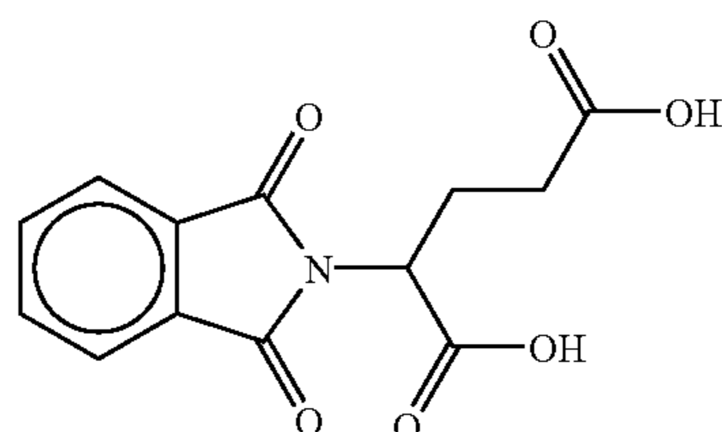
phthaloyl glutamic acid (PG Acid)
