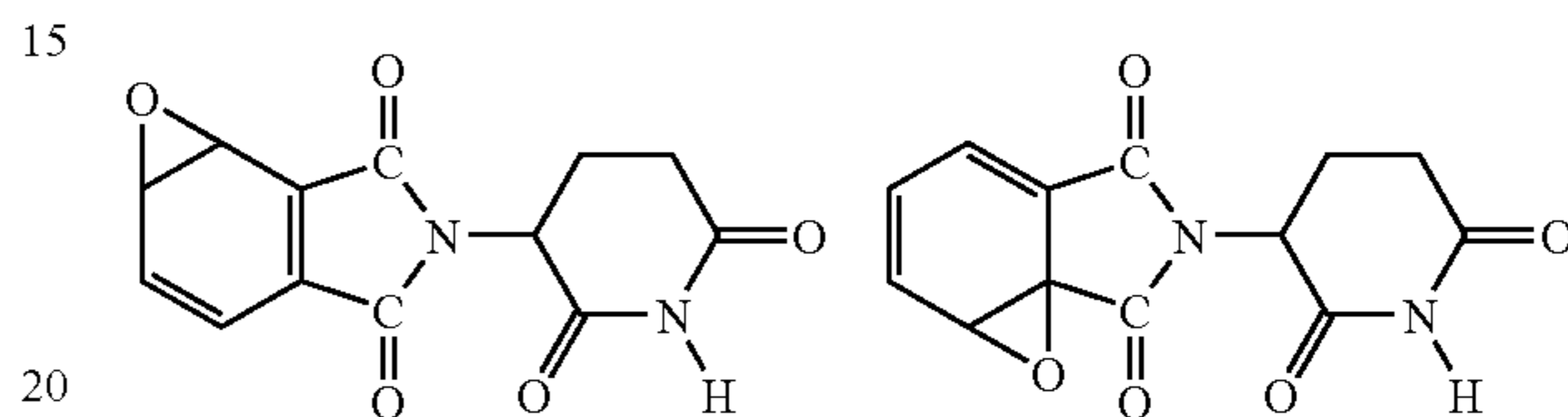
Epoxides of thalidomide
