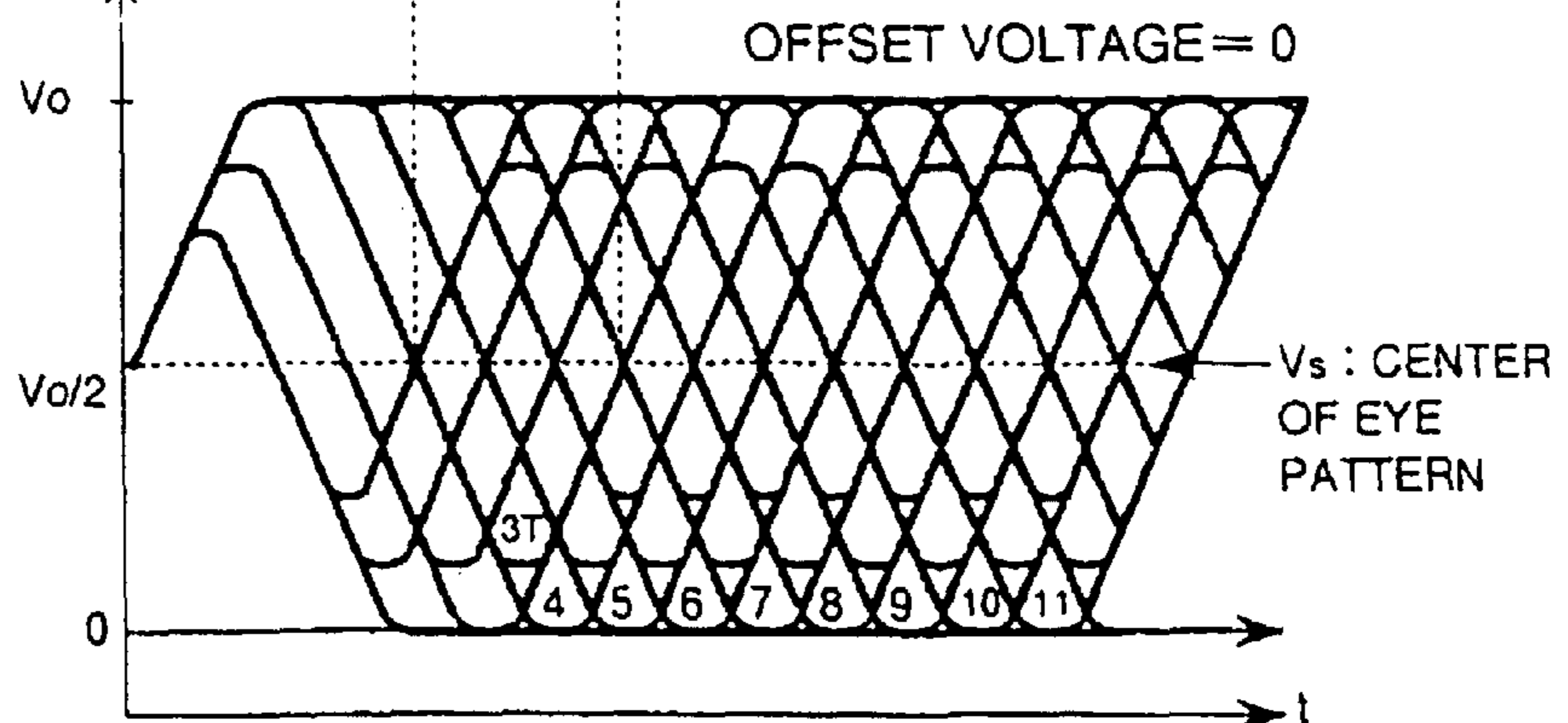
WAVEFORM (9) EYE PATTERN
