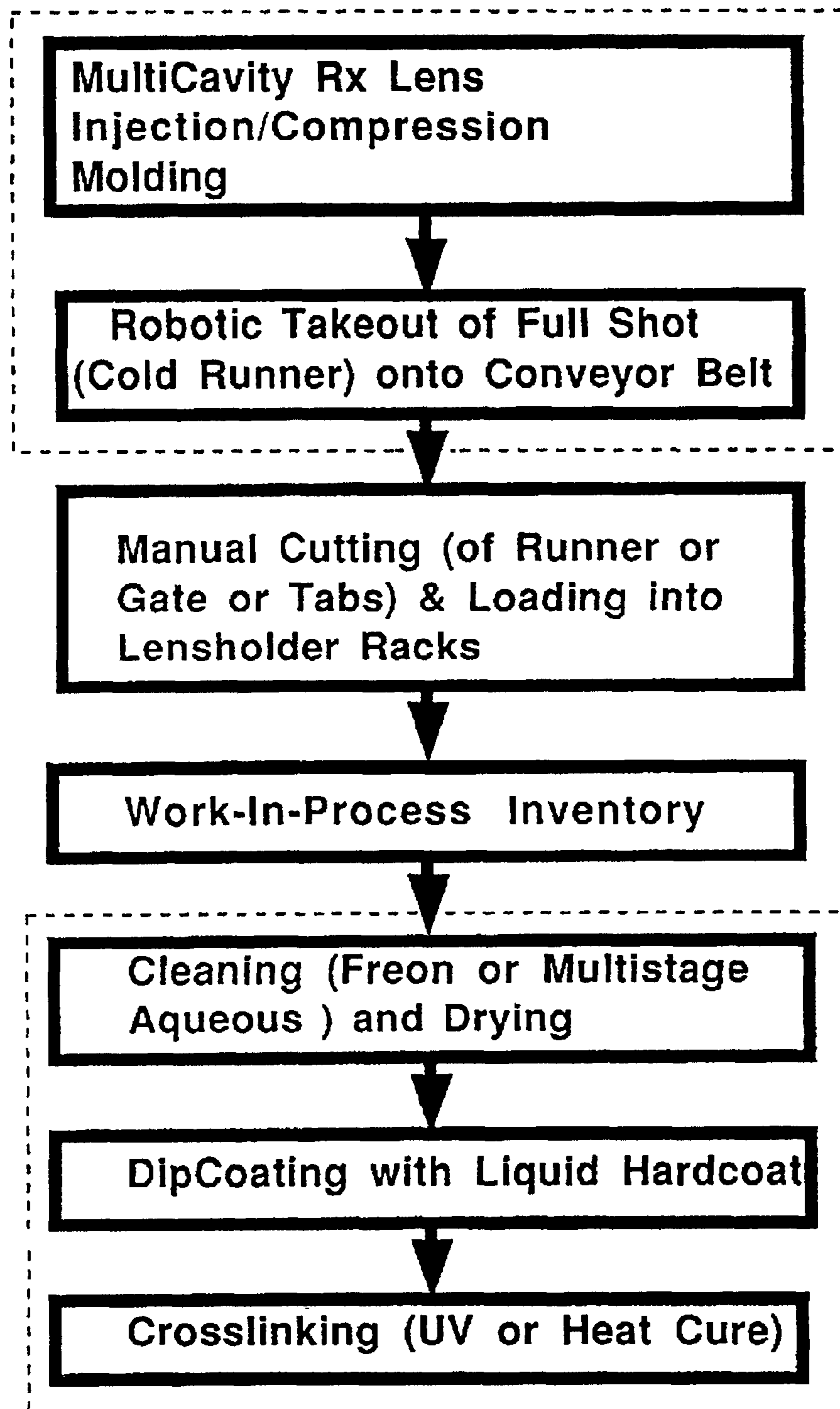
FIG. 4A: Comparative Example ("Batch Process")
