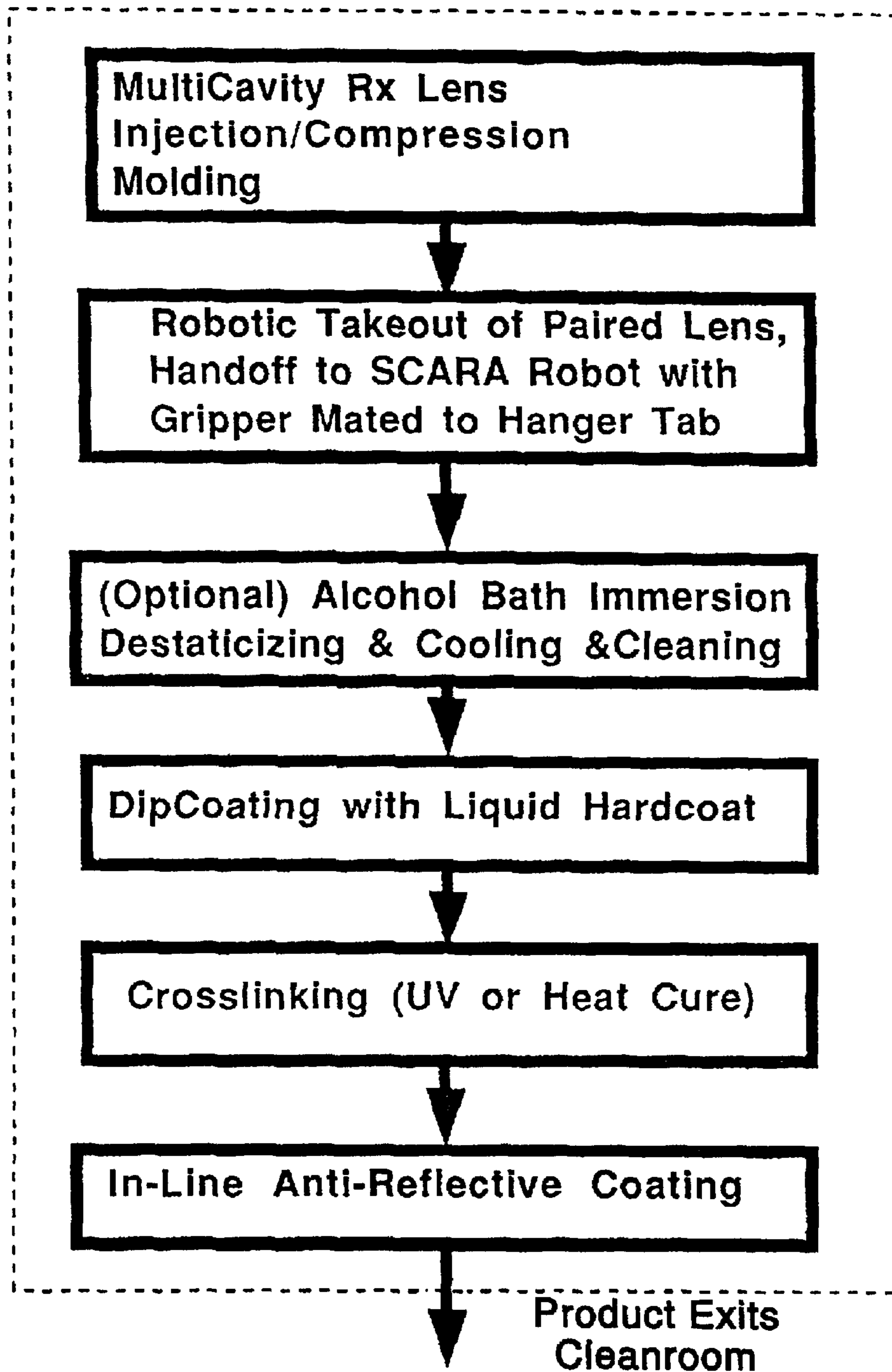
FIG. 4D: In-Line Automated AR Vacuum Coat of "Mold and Dipcoat" ("Continuous Process")
