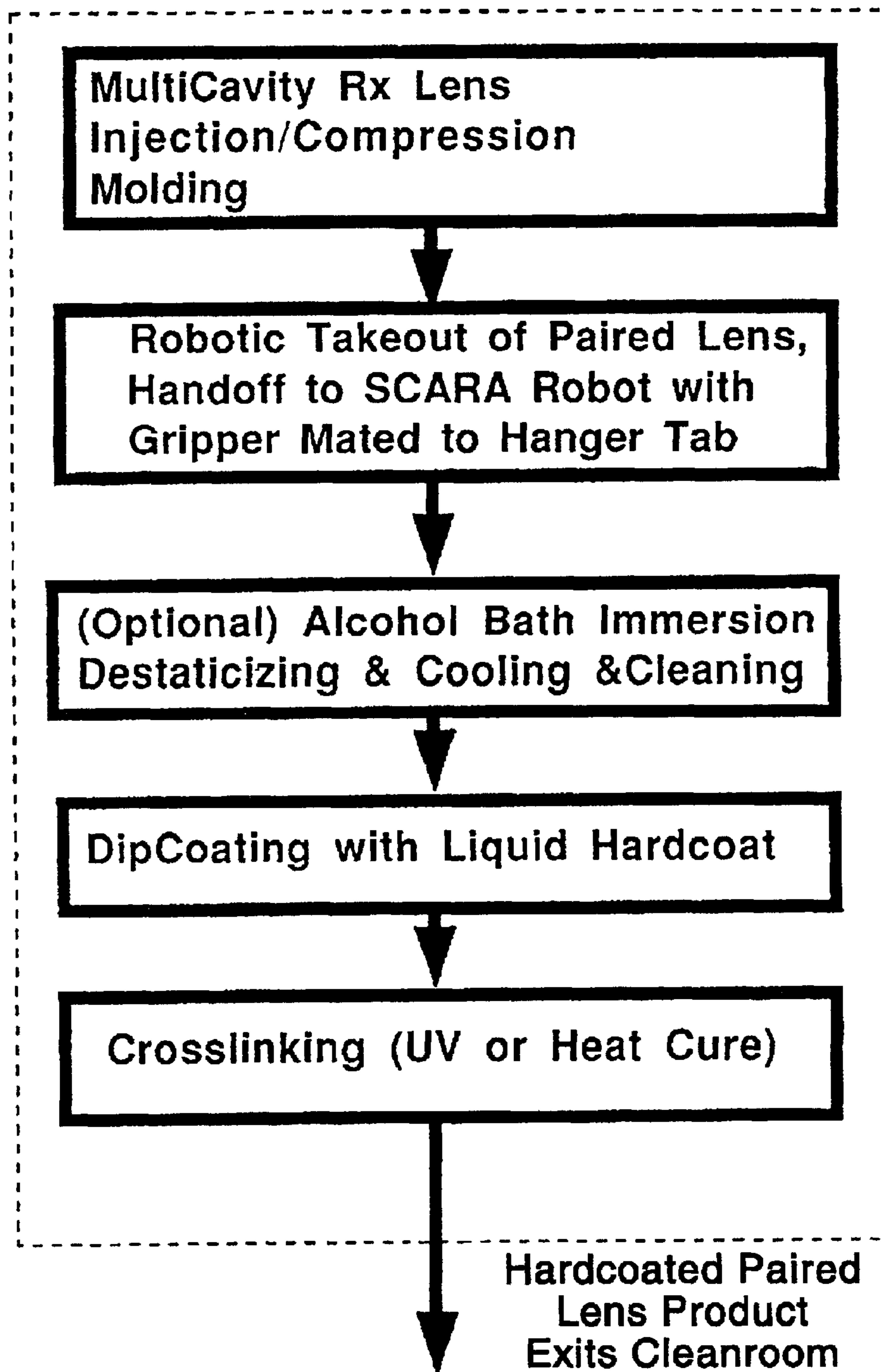
FIG. 4B: Automated "Mold And Dipcoat" ("Continuous Process")
