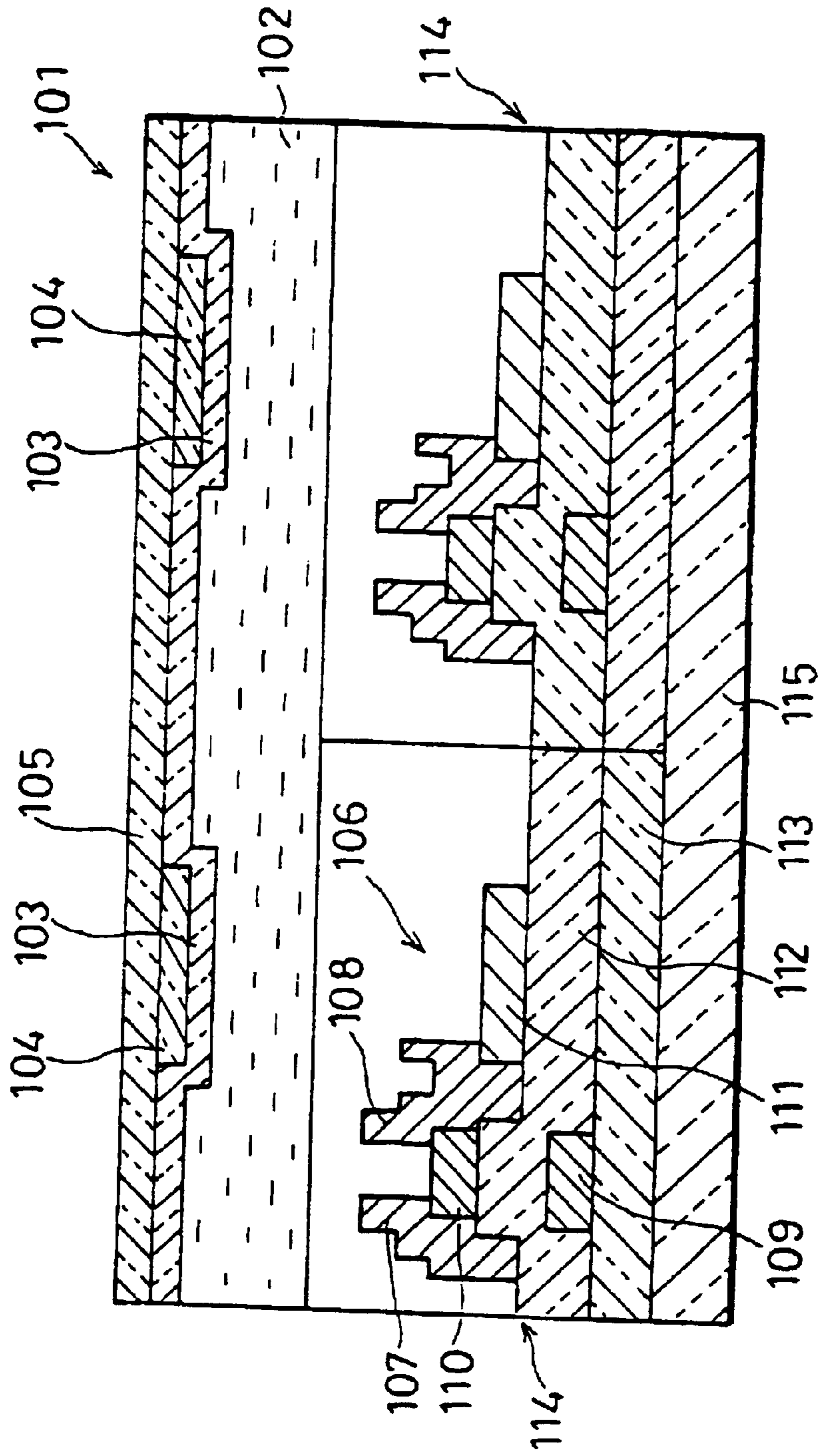
FIG. 15 (PRIOR ART)
