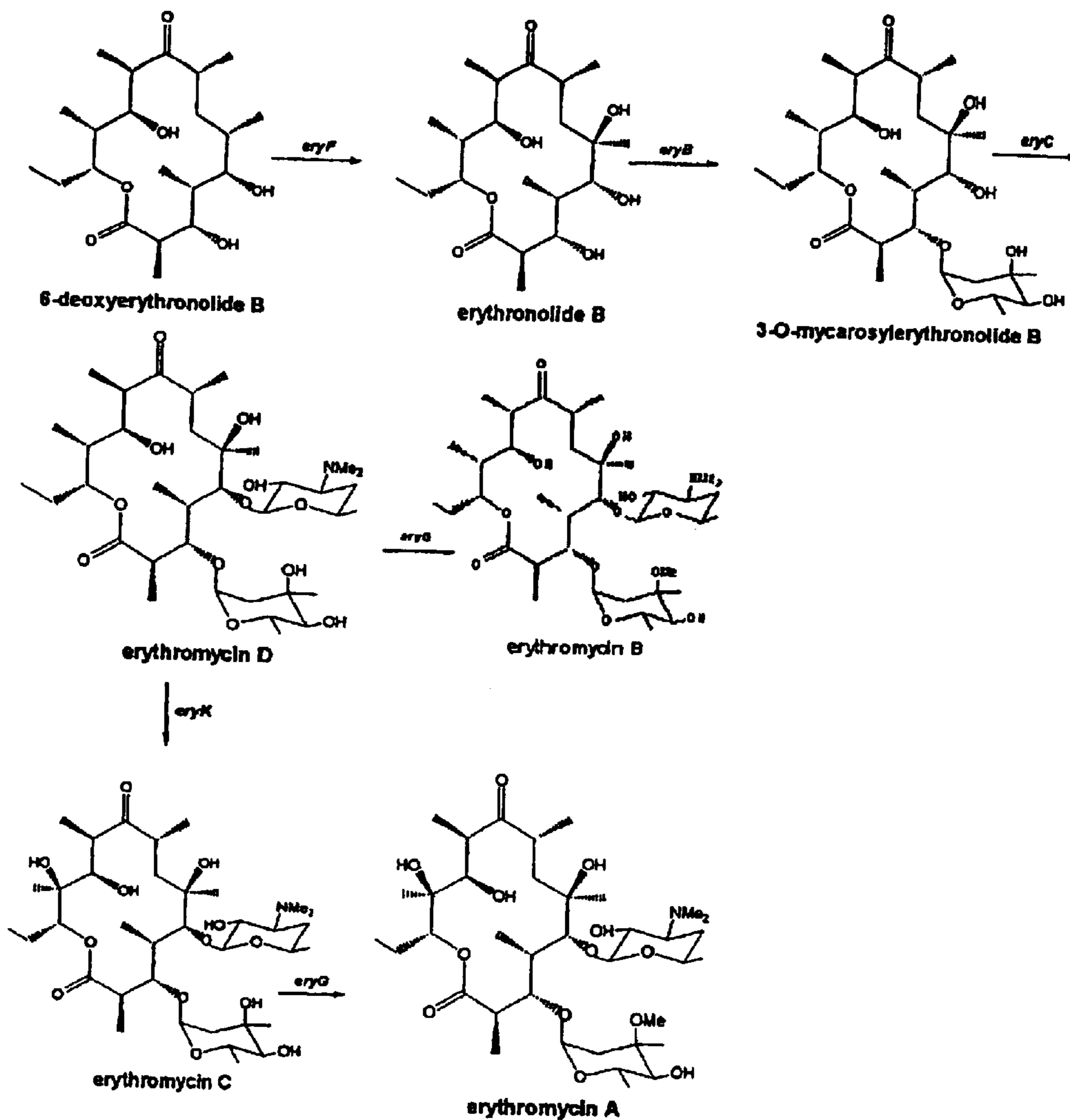
Post-PKS Biosynthesis of Erythromycins
