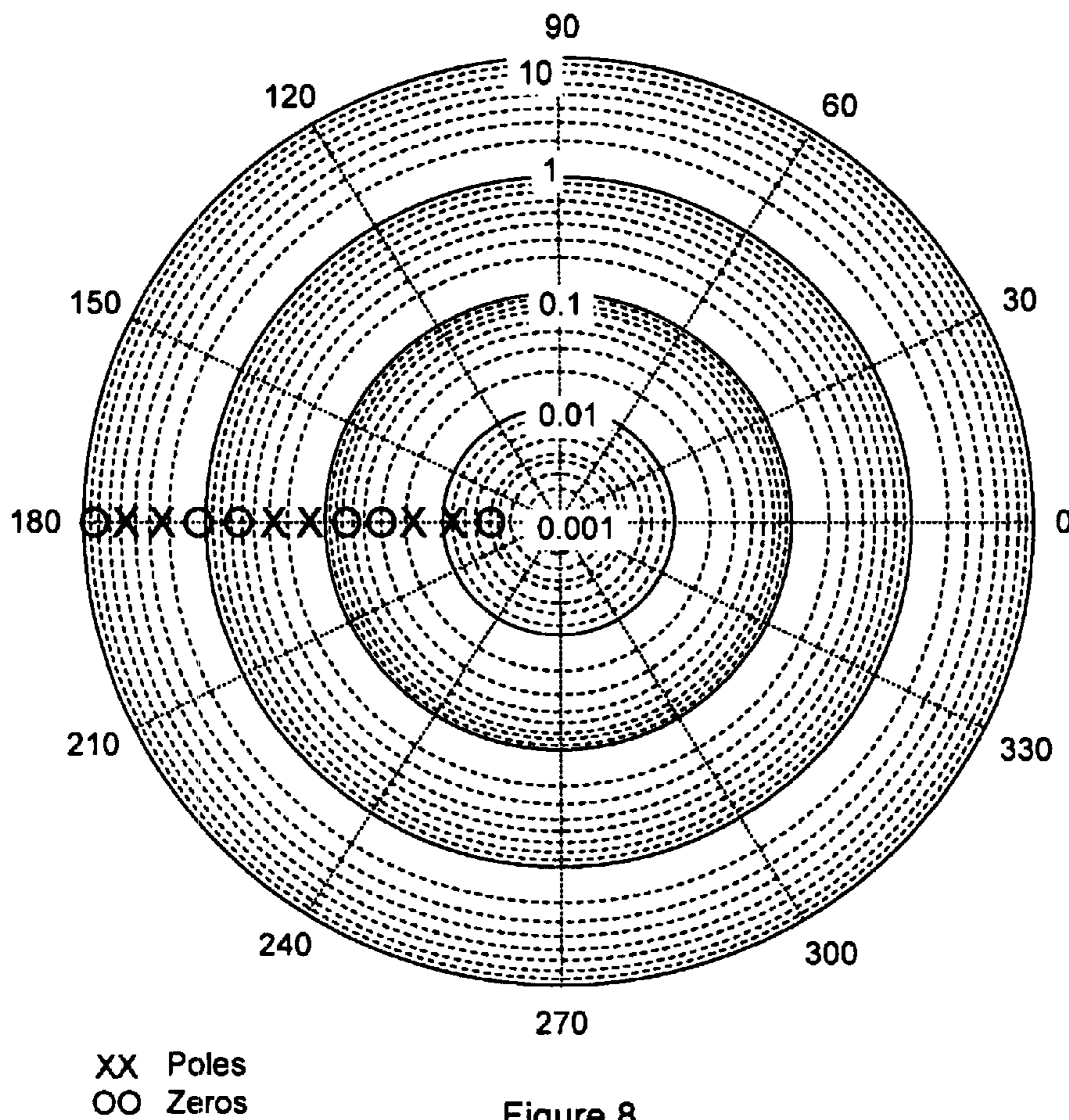
Poles and Zeros of Initial Filter Guess
