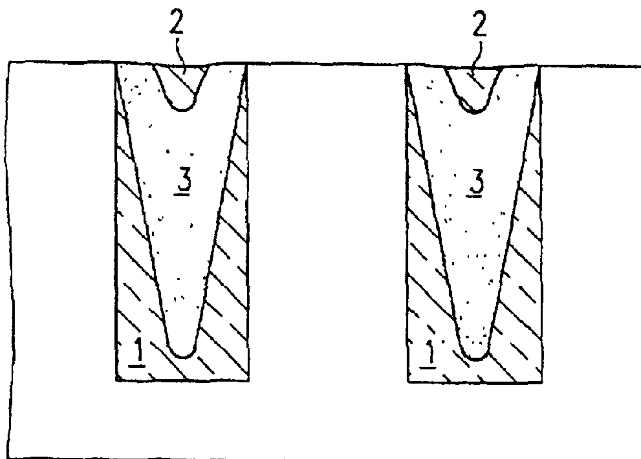
FIG. 3C SOG/LTO etchback
