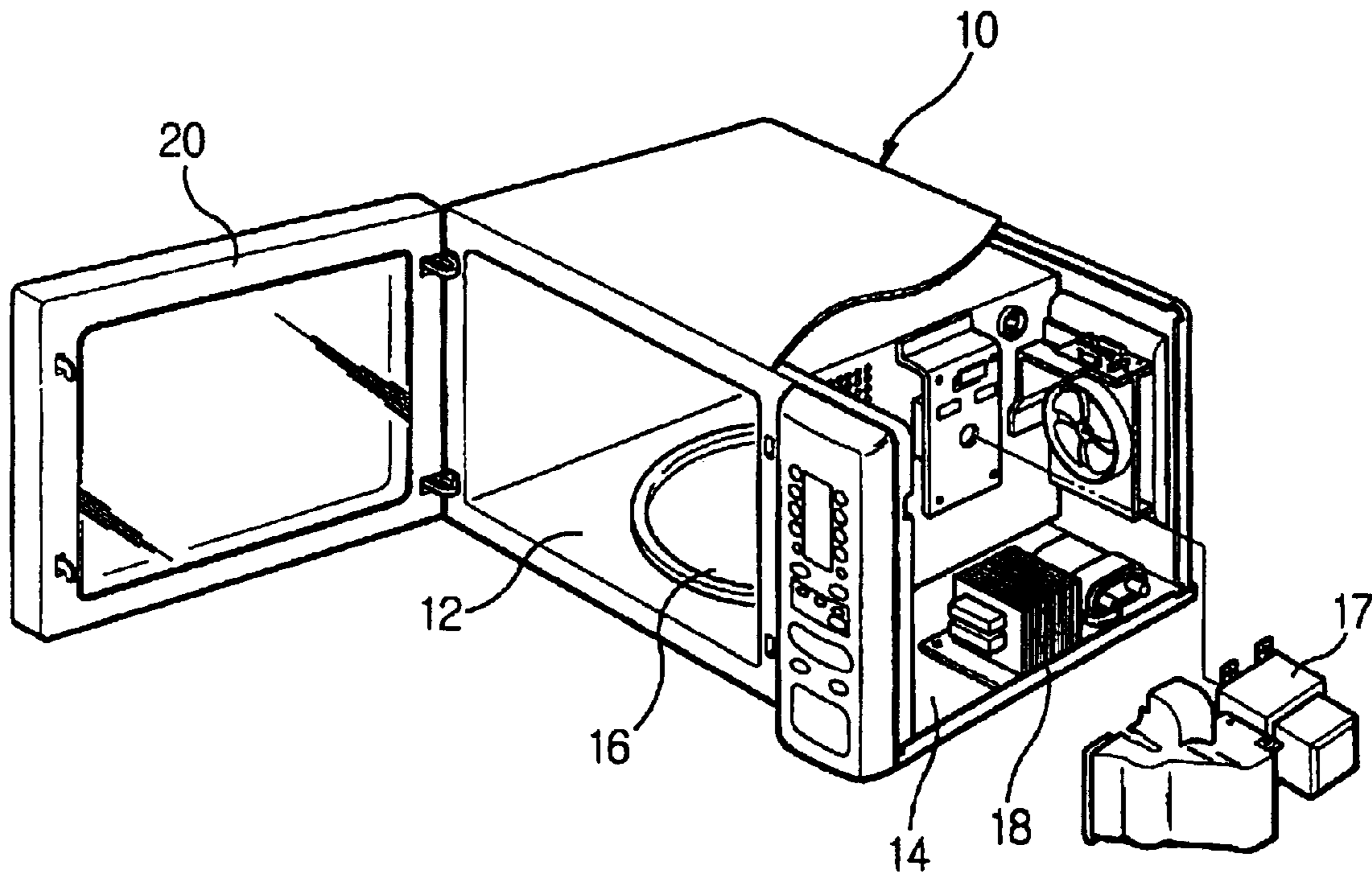
FIG. 1 (PRIOR ART)
