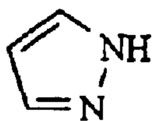
pyrazole
