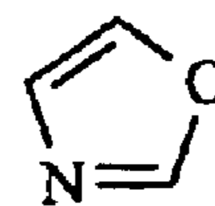
oxazole
