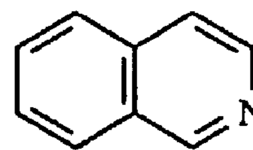
isoquinoline
