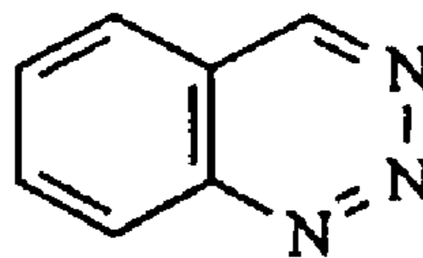
benzotriazine
