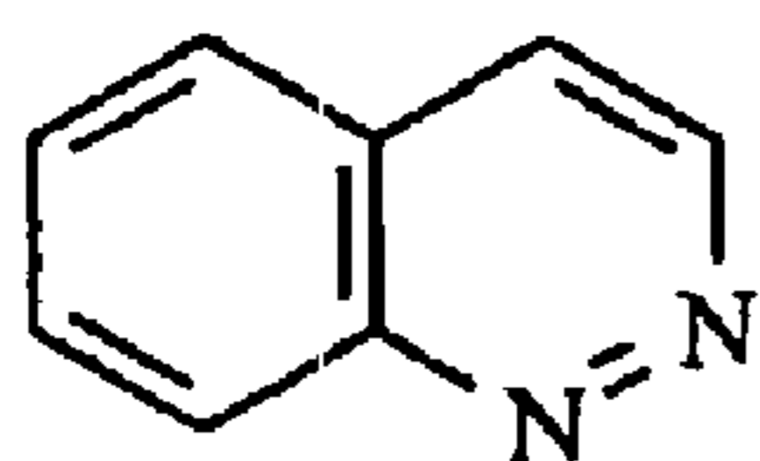
cinnoline
