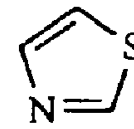
thiazole
