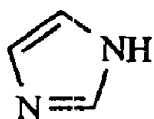
imidazole
