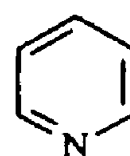
pyridine
