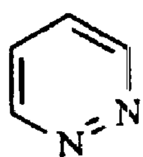
pyridazine
