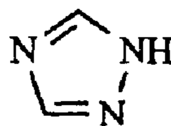
1,2,4-triazole
