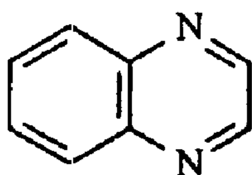
quinoxaline
