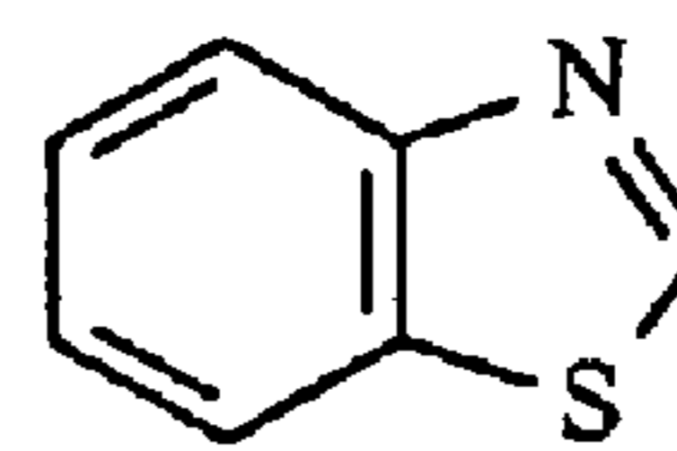
benzothiazole
