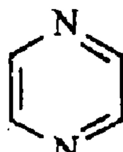
pyrazine
