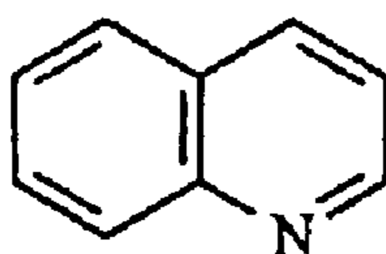
quinoline
