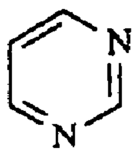
pyrimidine
