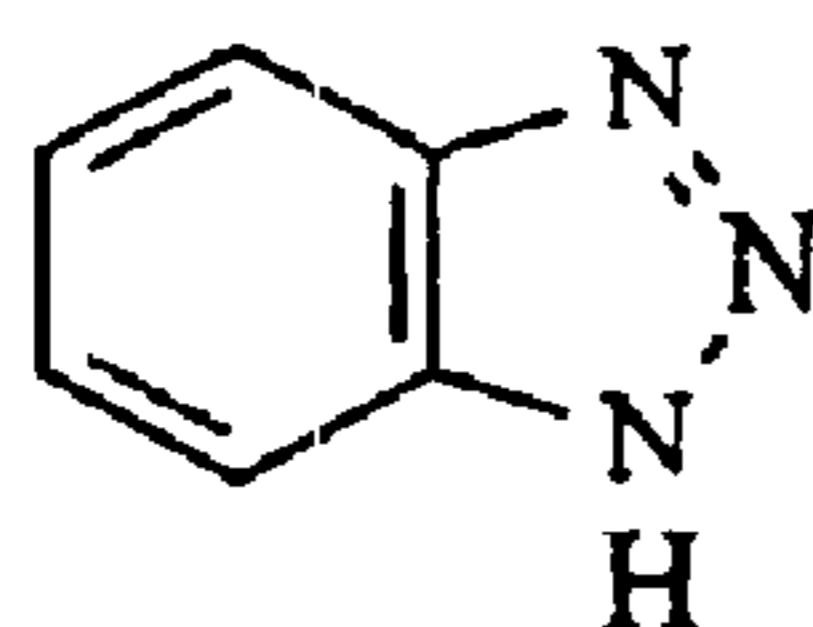
benzotriazole
