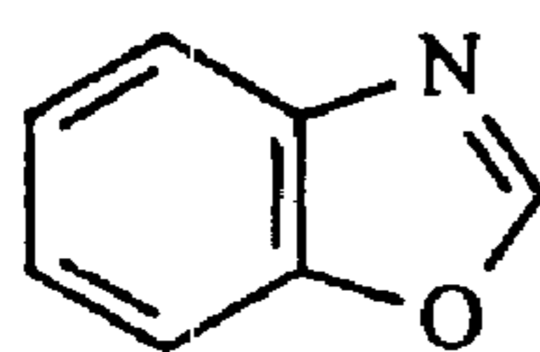
benzoxazole
