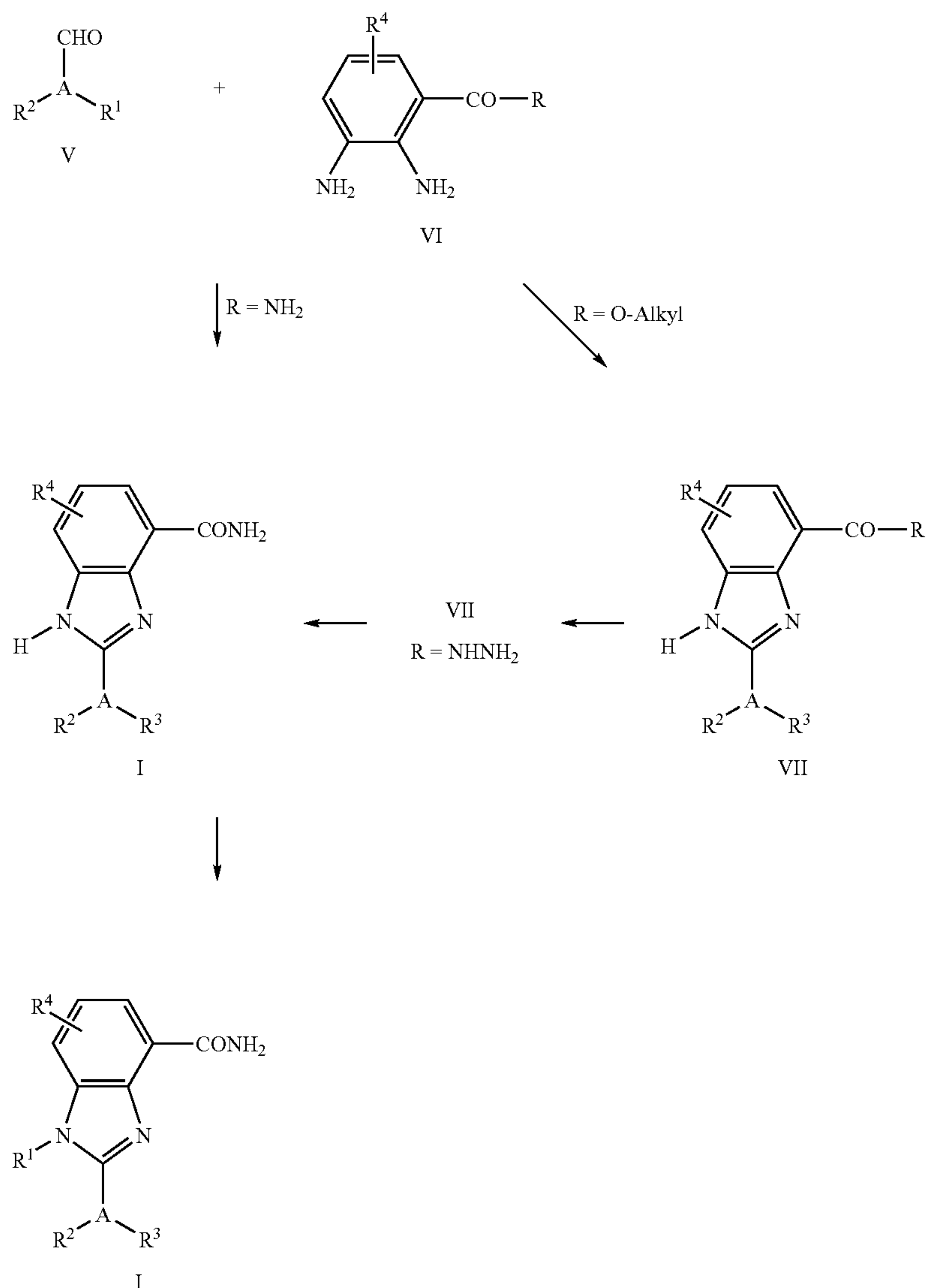
Synthesis Scheme 1
