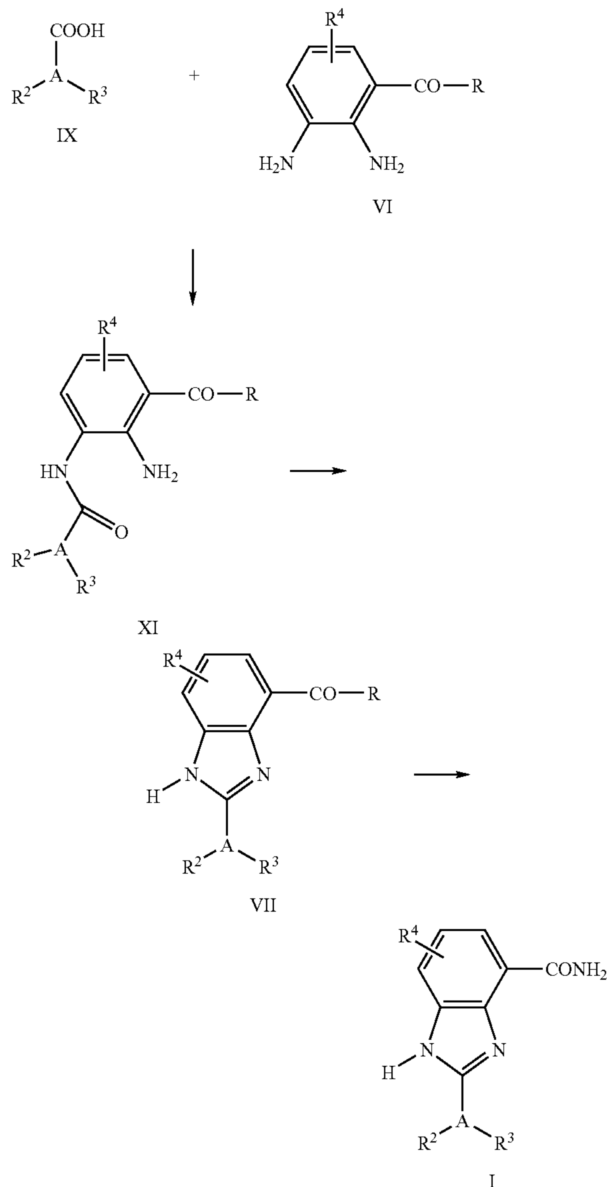
Synthesis Scheme 2
