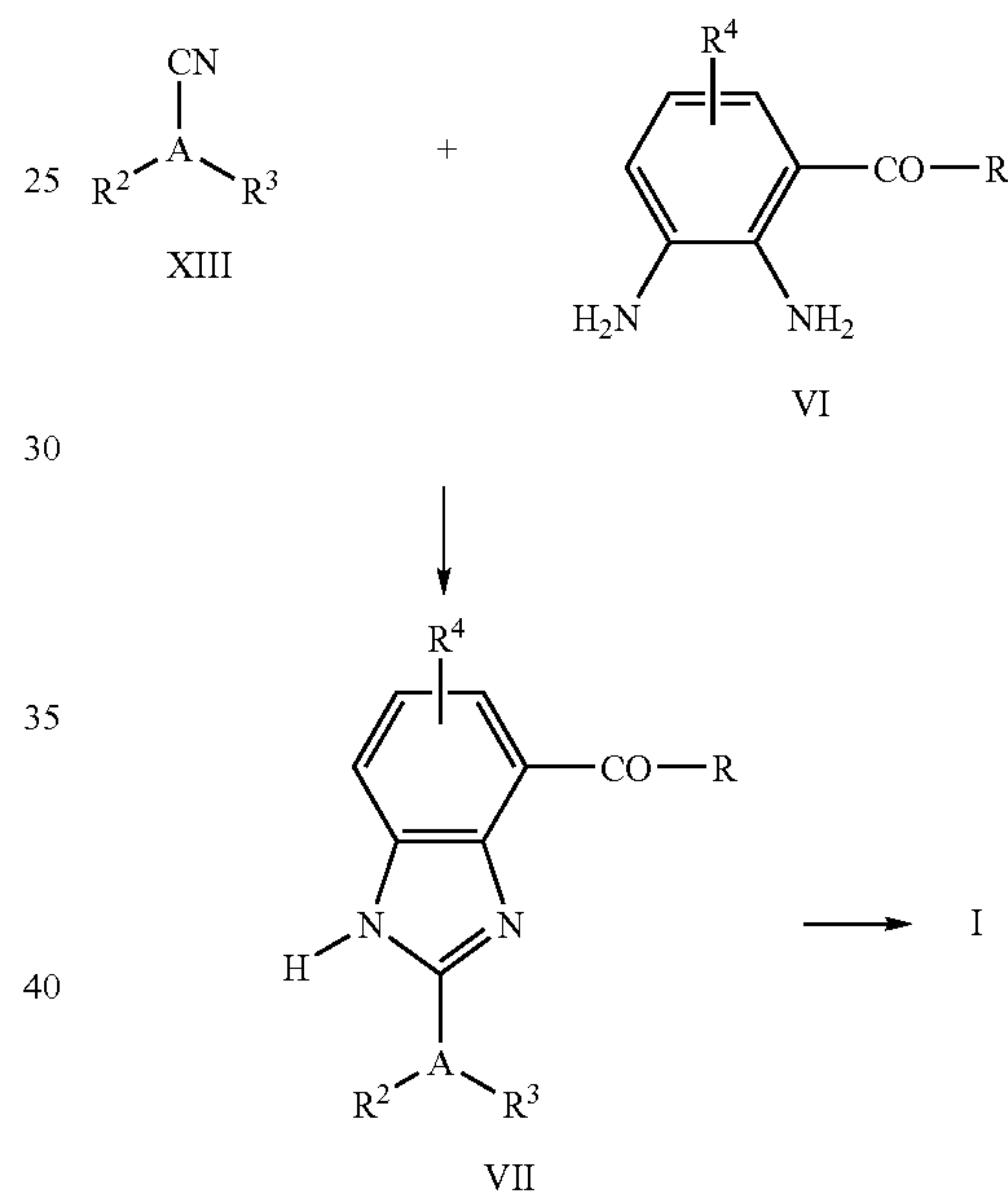
Synthesis Scheme 3
