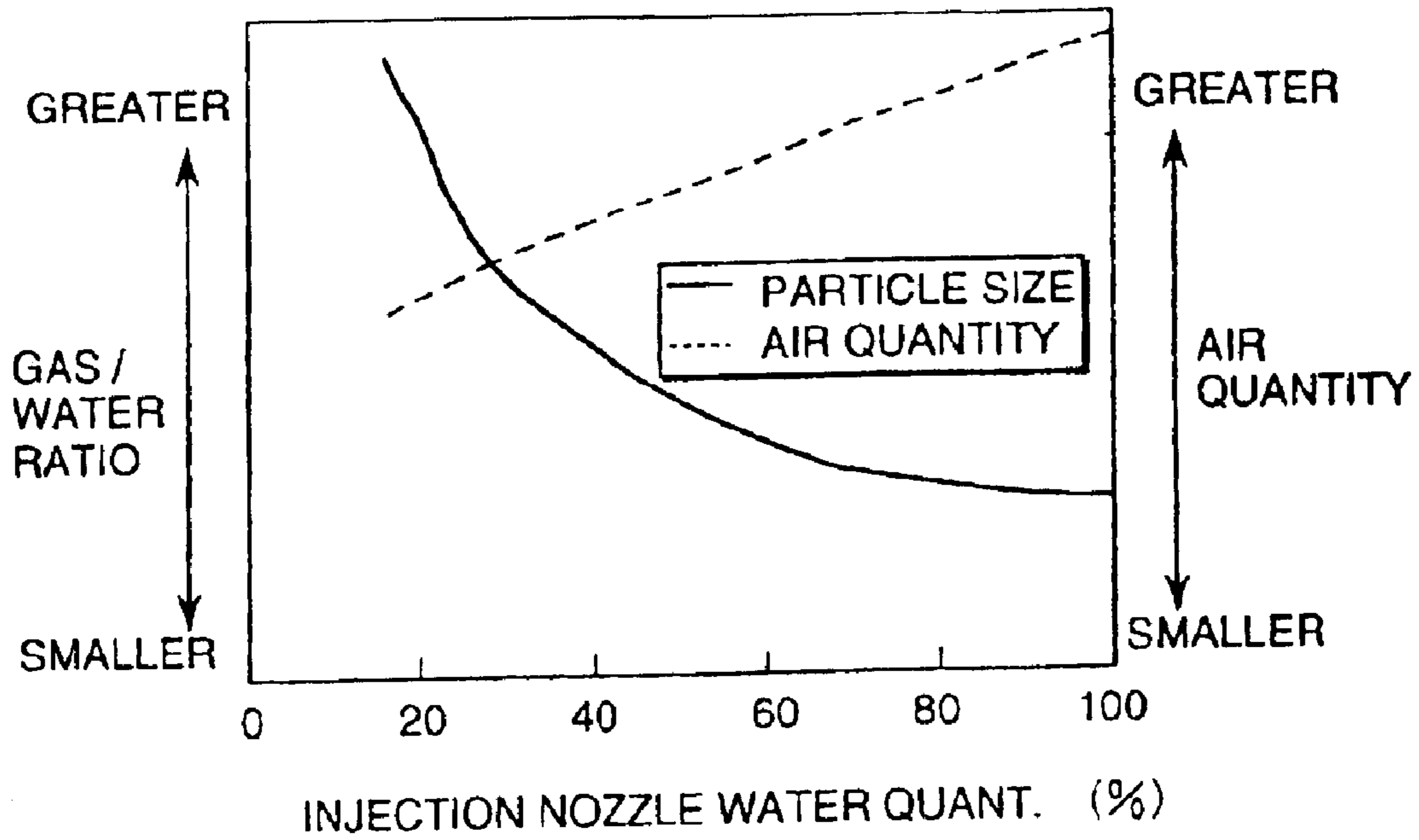
RELATION OF WATER QUANT. VS GAS / WATER RATIO, AIR QUANT. UNDER A CONSTANT PARTICLE SIZE
