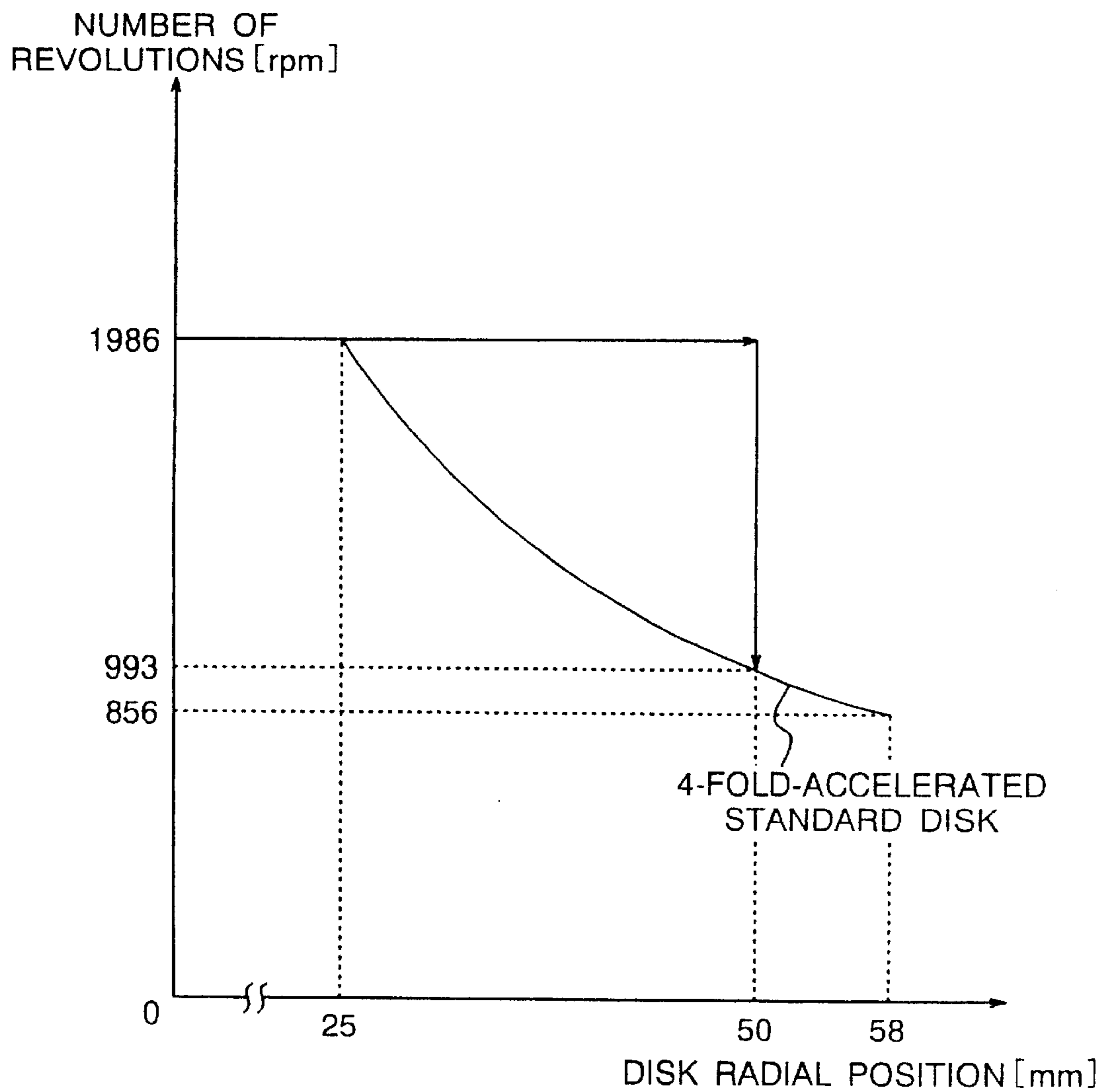
FIG. 19 PRIOR ART
