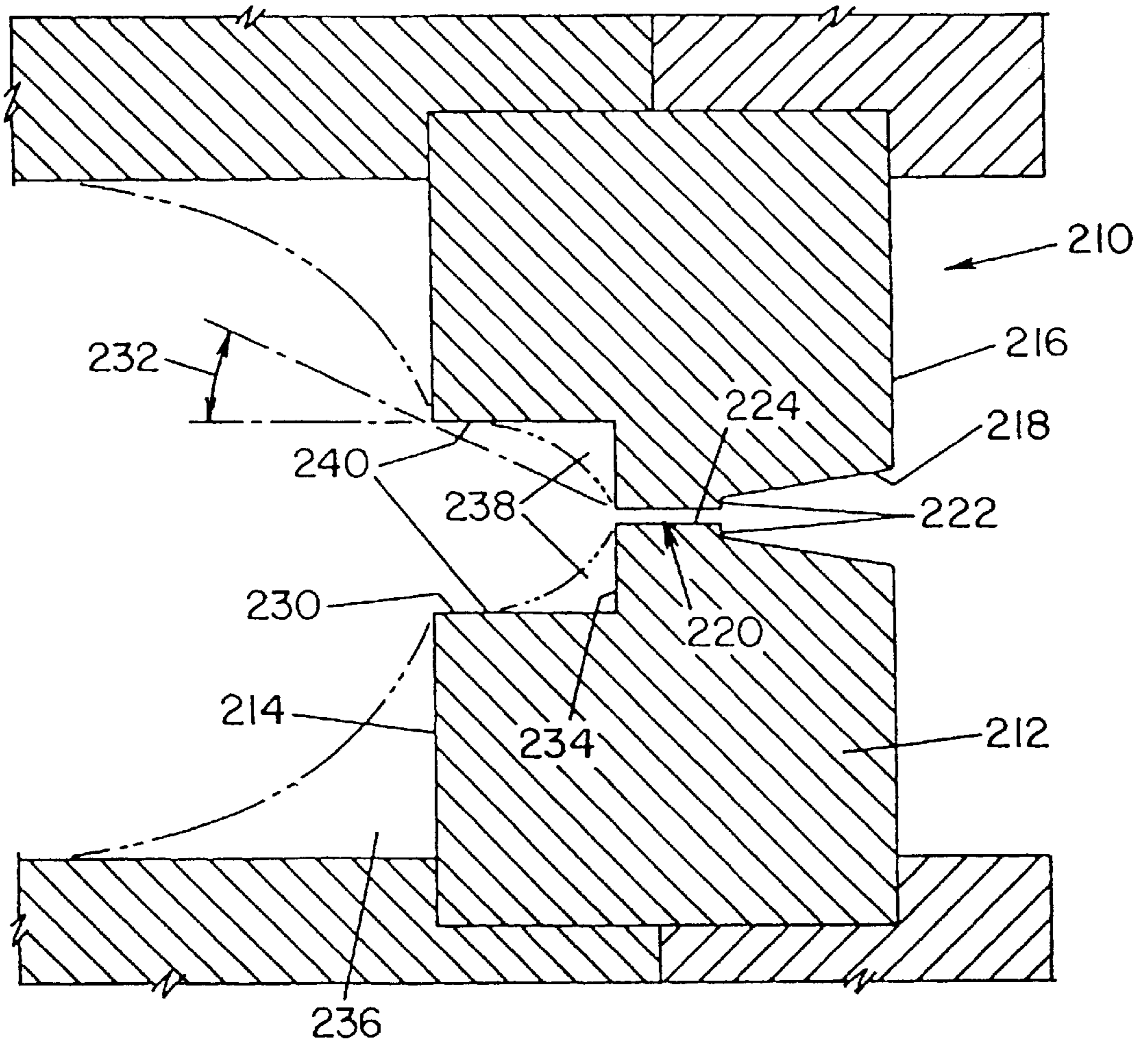
FIG. 1 (PRIOR ART)
