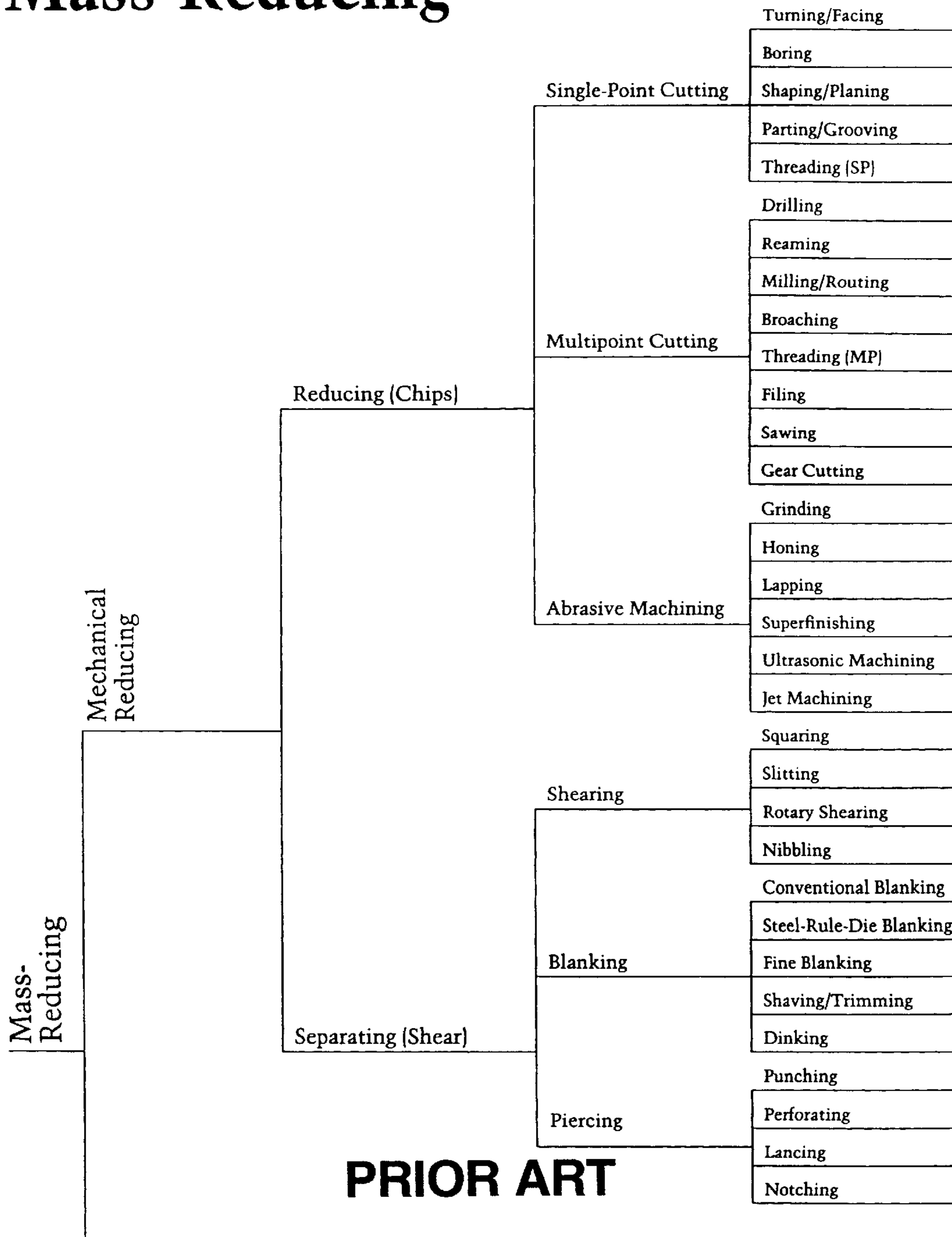
Taxonomy of Manufacturing Processes: Mass-Reducing
