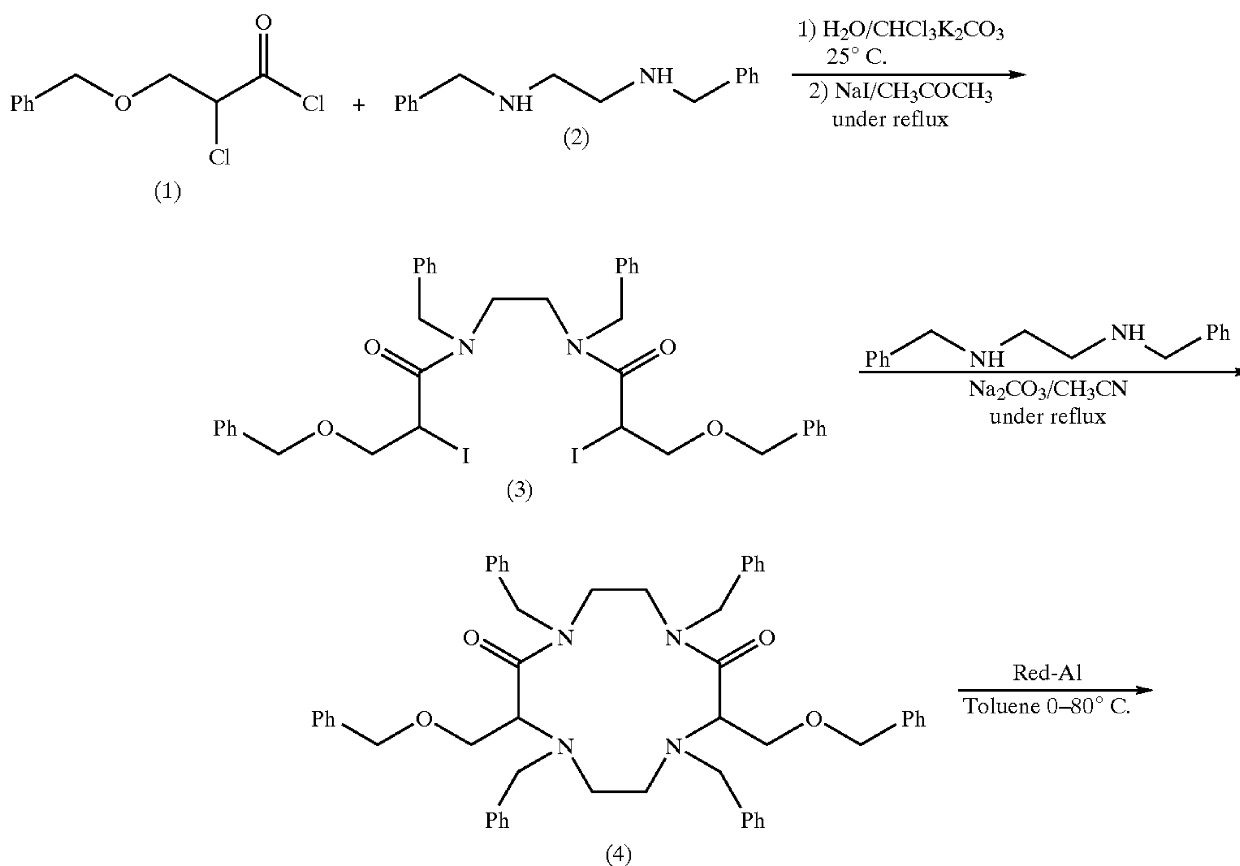
SCHEME 2
