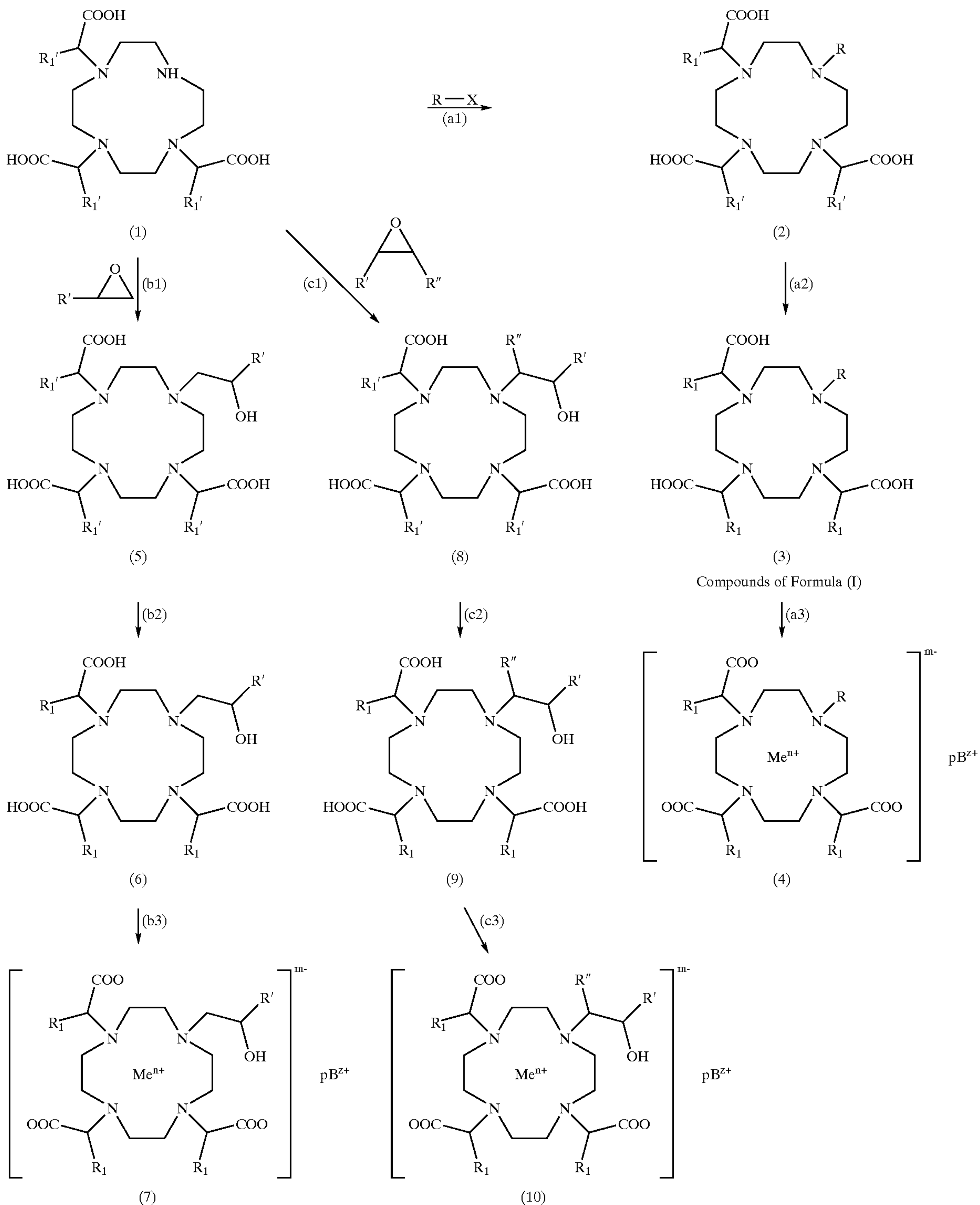
SCHEME 1
