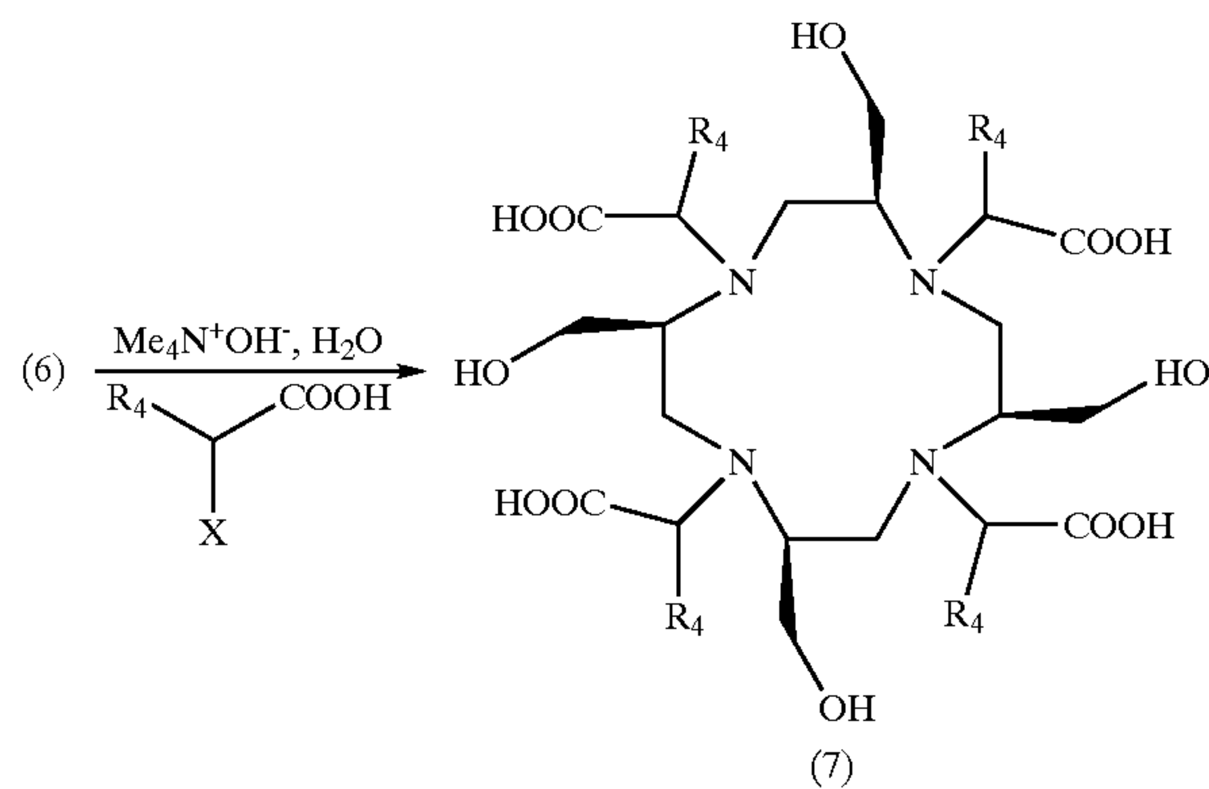
SCHEME 5
