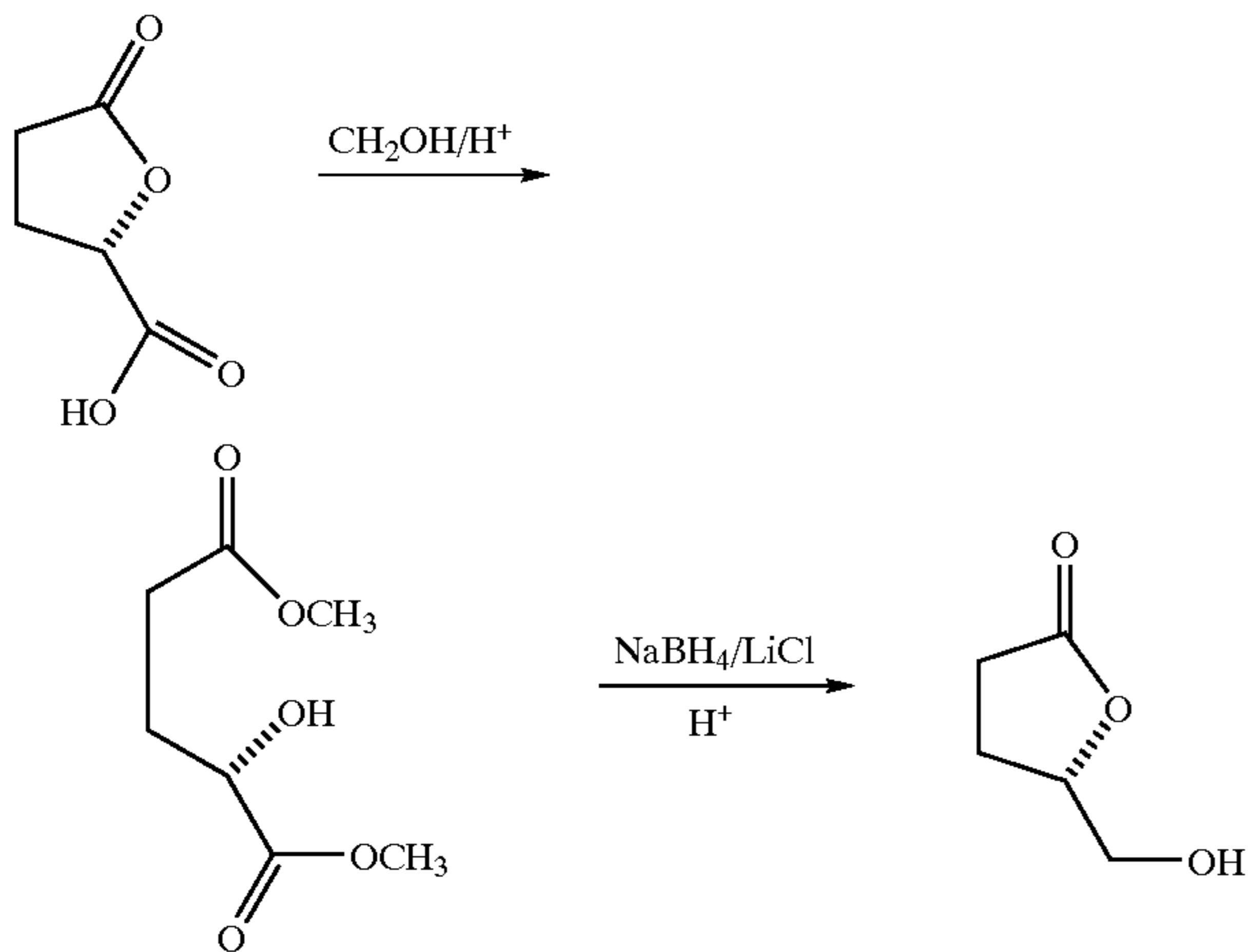
Scheme III
