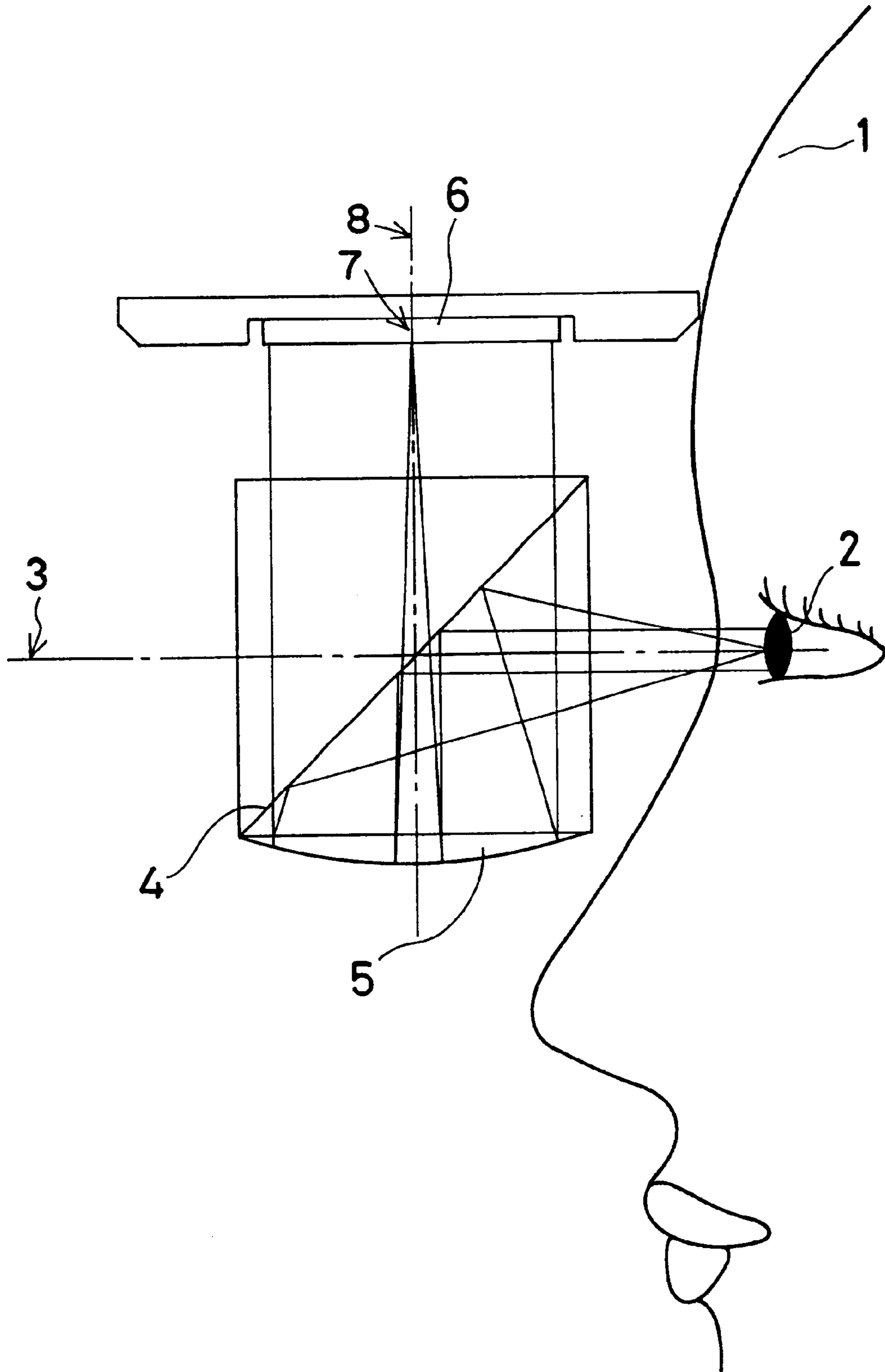
FIG. 18 (PRIOR ART)
