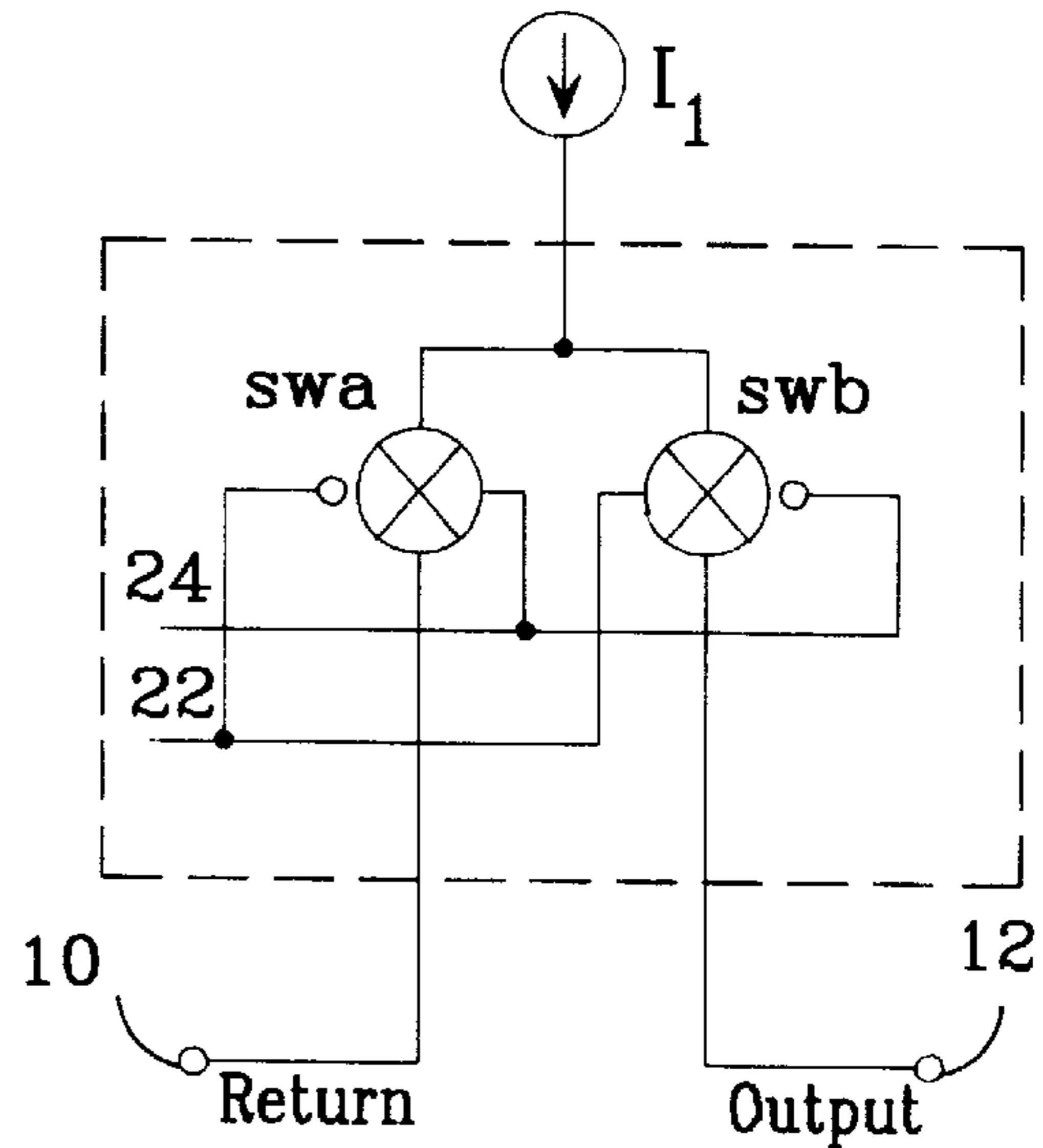
FIG. 2C (Prior Art)
