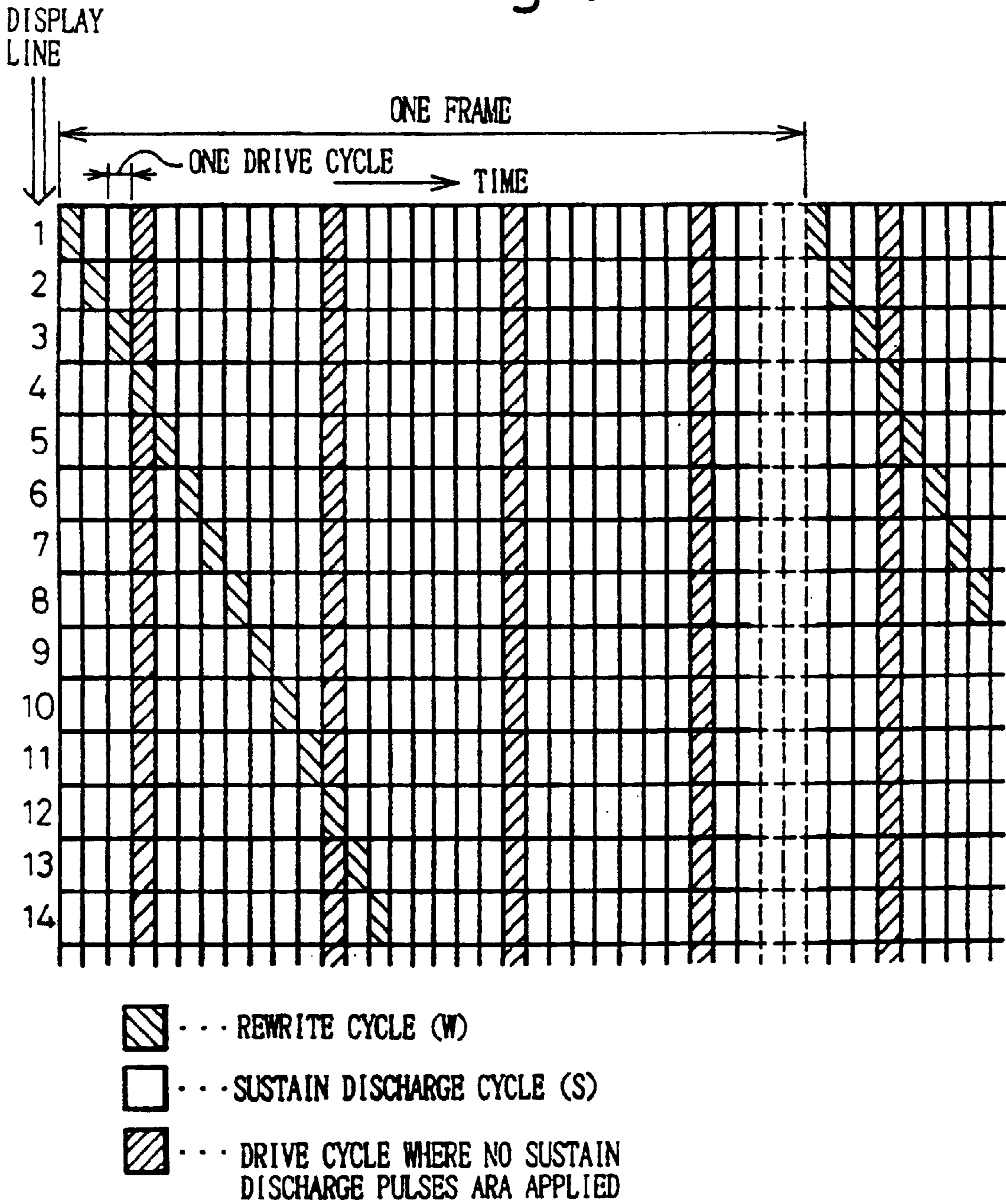
Fig. 57 PRIOR ART
