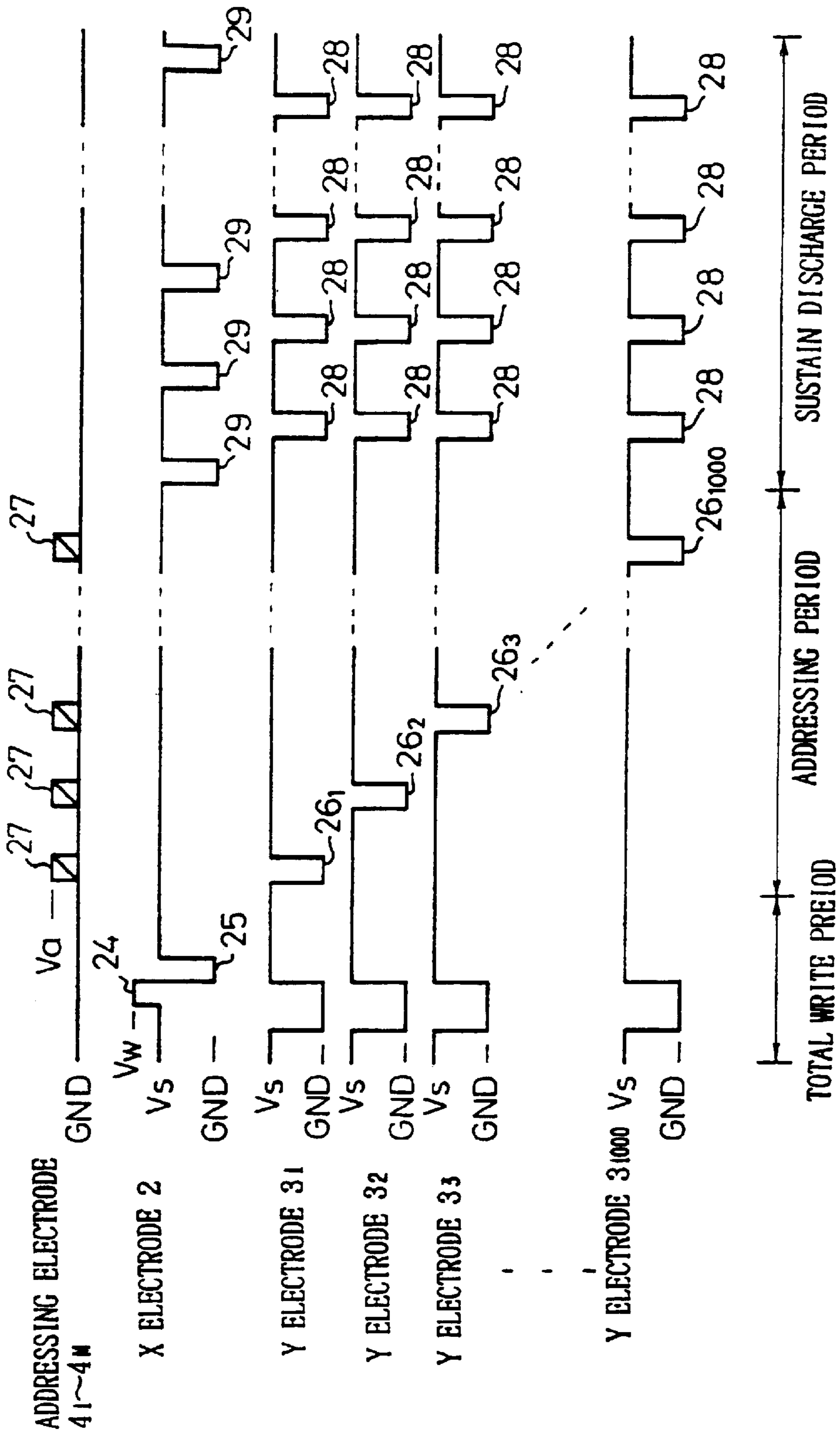
Fig. 6 PRIOR ART
