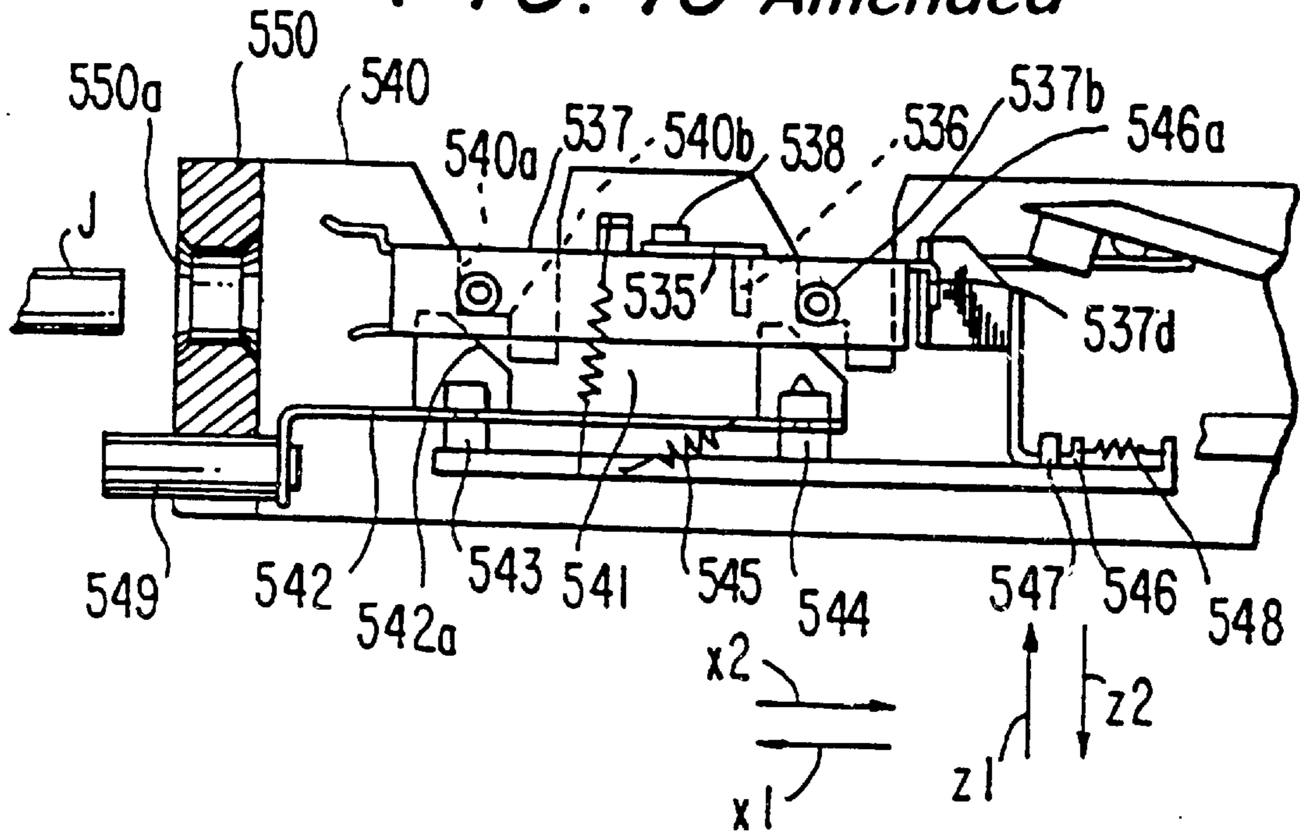
PRIOR ART FIG. 46 Amended
