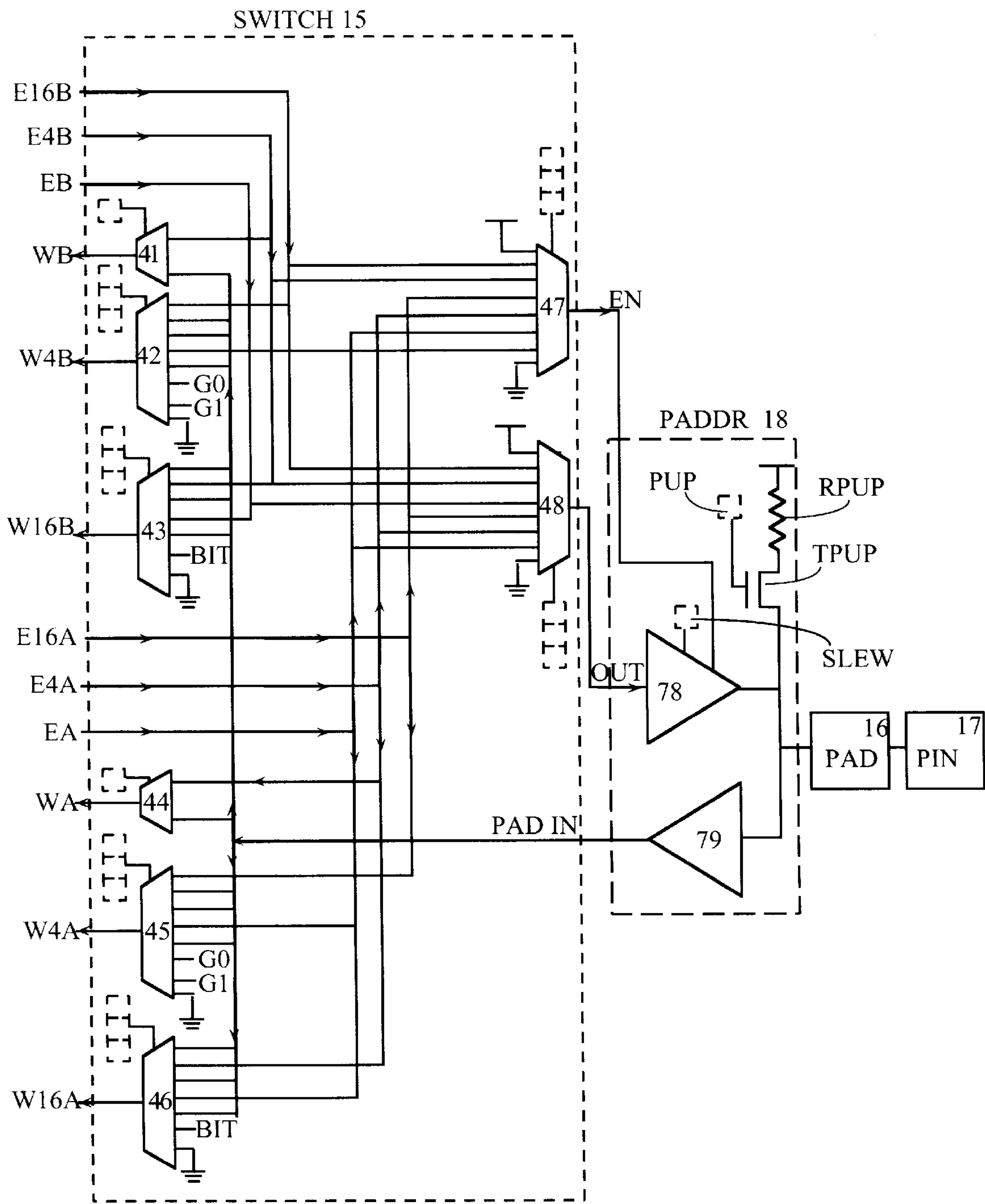
FIG. 4 PRIOR ART
