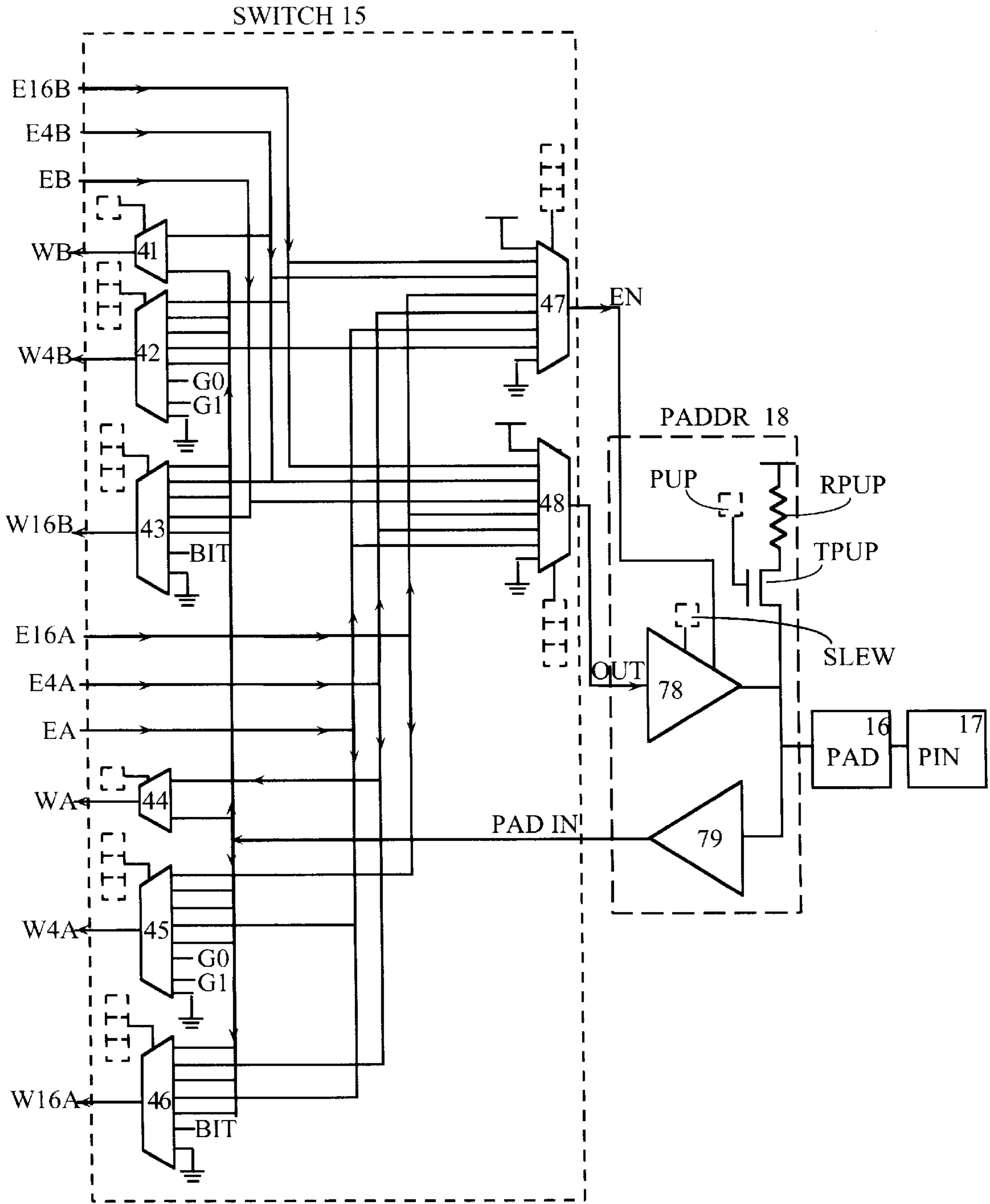
FIG. 4 PRIOR ART
