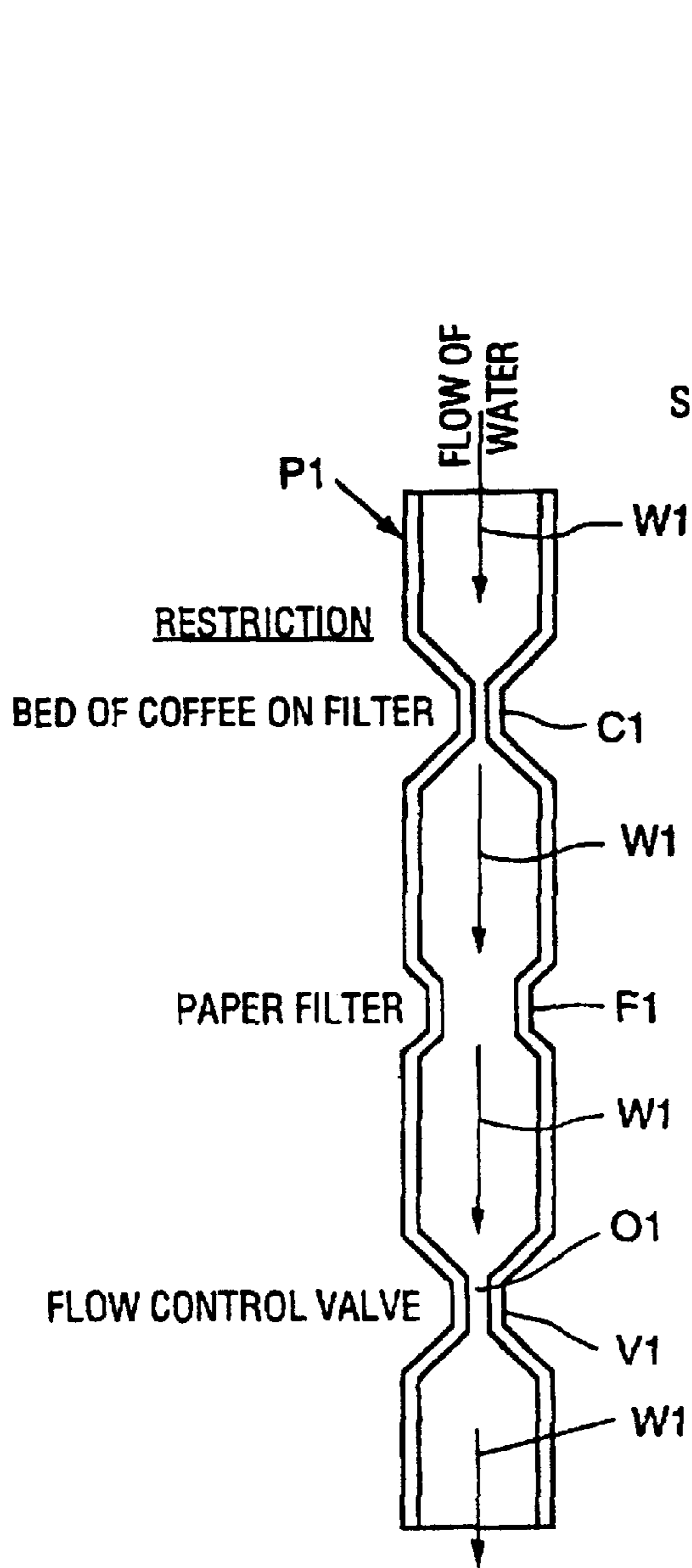
(PRIOR ART) FIG. 5A
