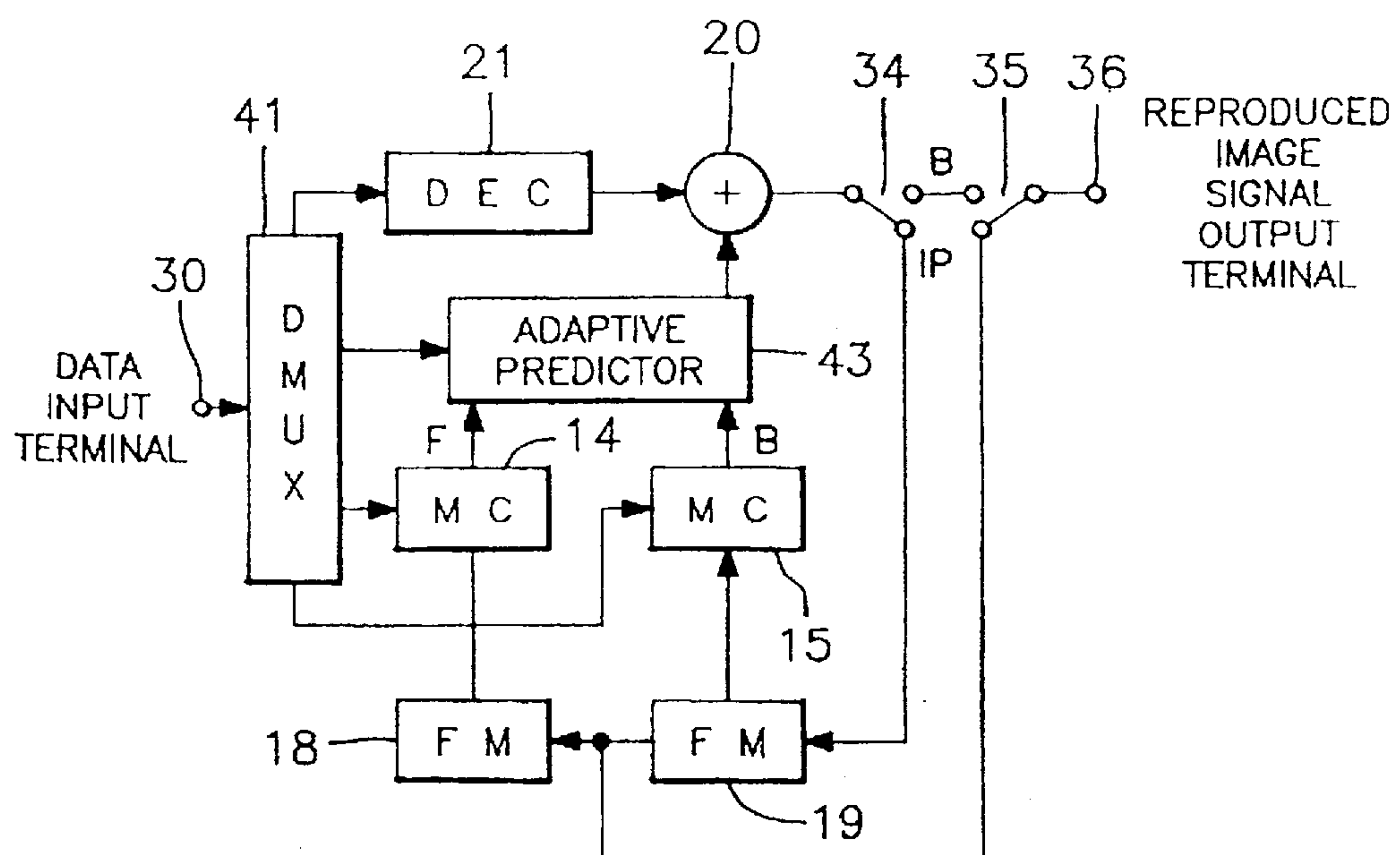
FIG. 2 (PRIOR ART)
