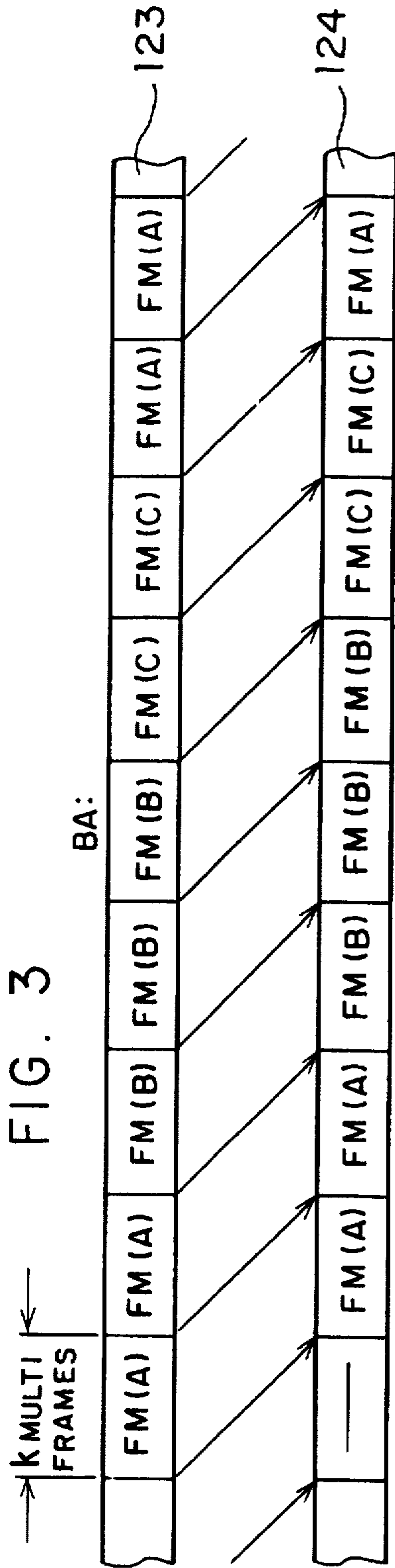
TRANSMISSION FRAME FM: FRAME FORMAT TYPE
