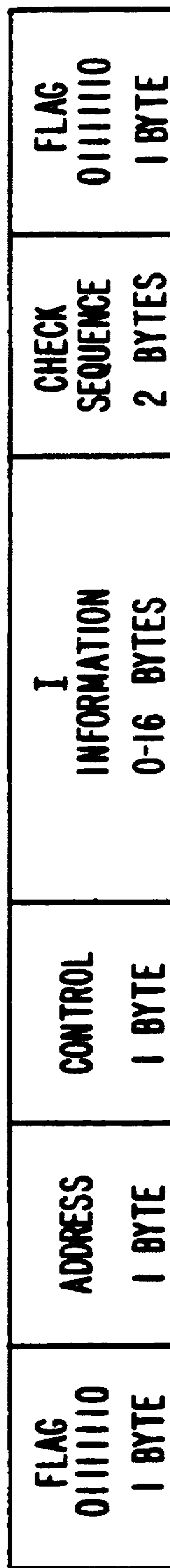
HDLC FRAME FORMAT
