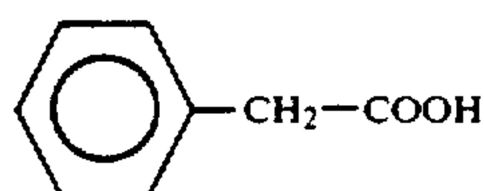
phenylacetic acid
