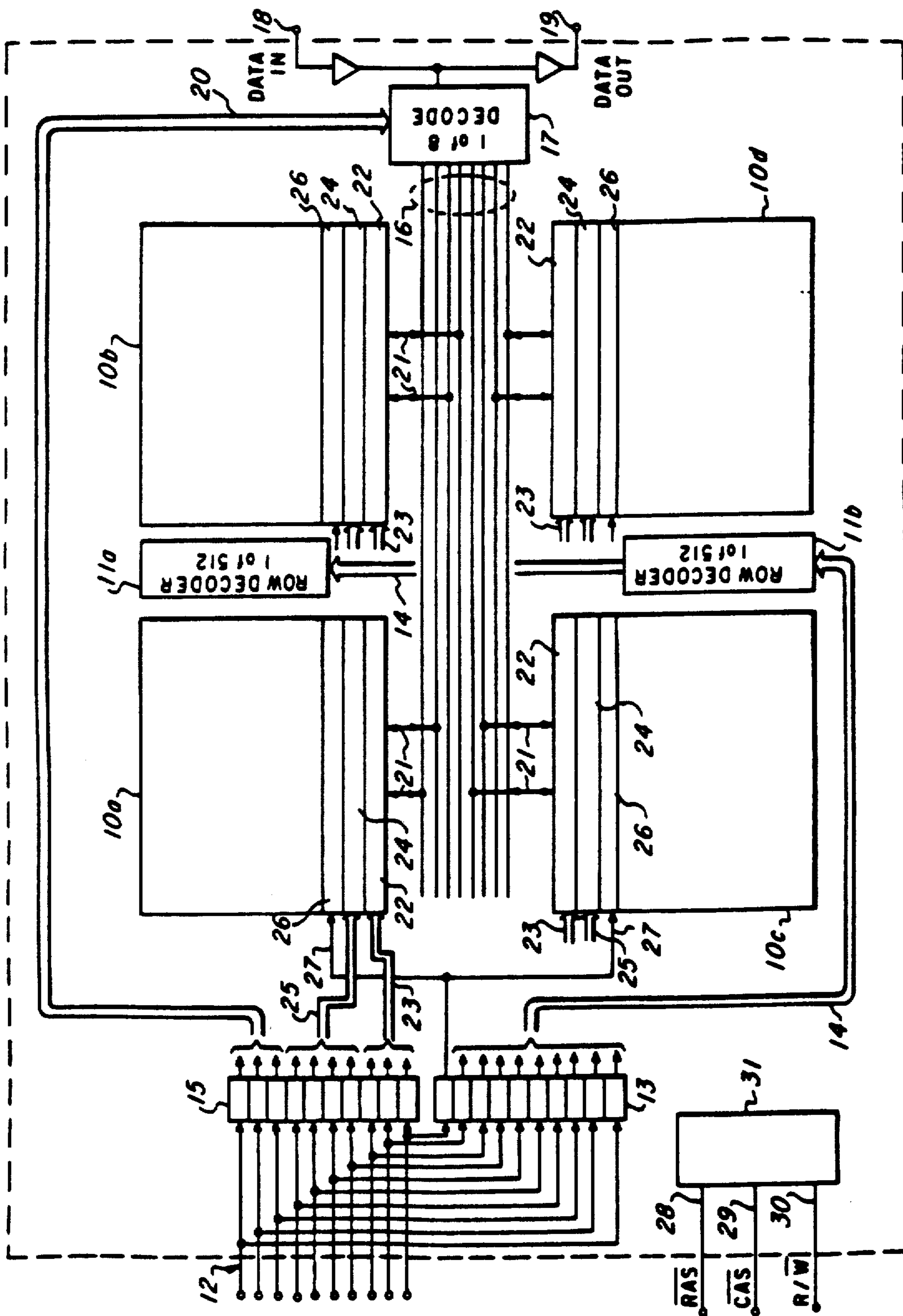
SEMICONDUCTOR CHIP Fig. 3
