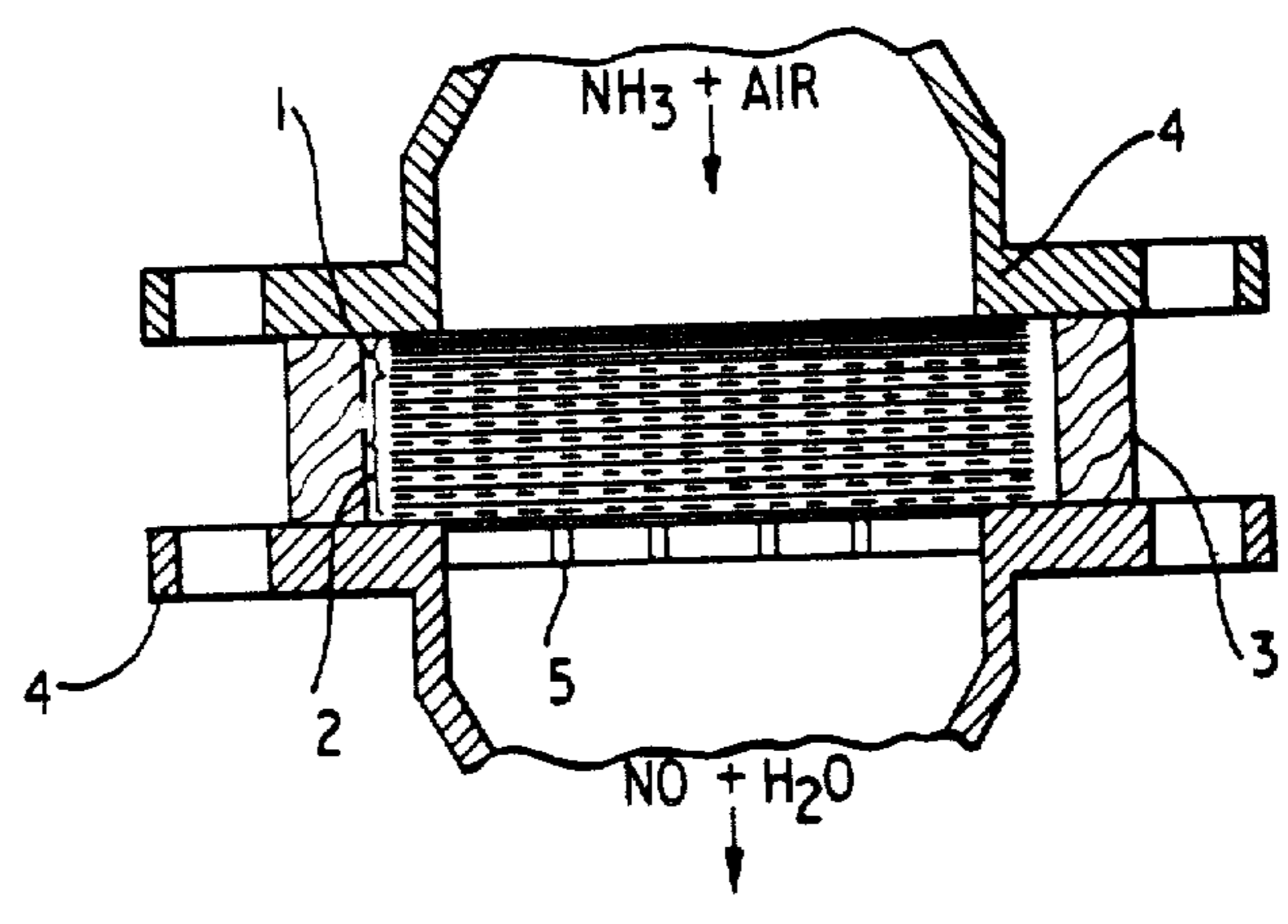
FIG. X. (PRIOR ART)
