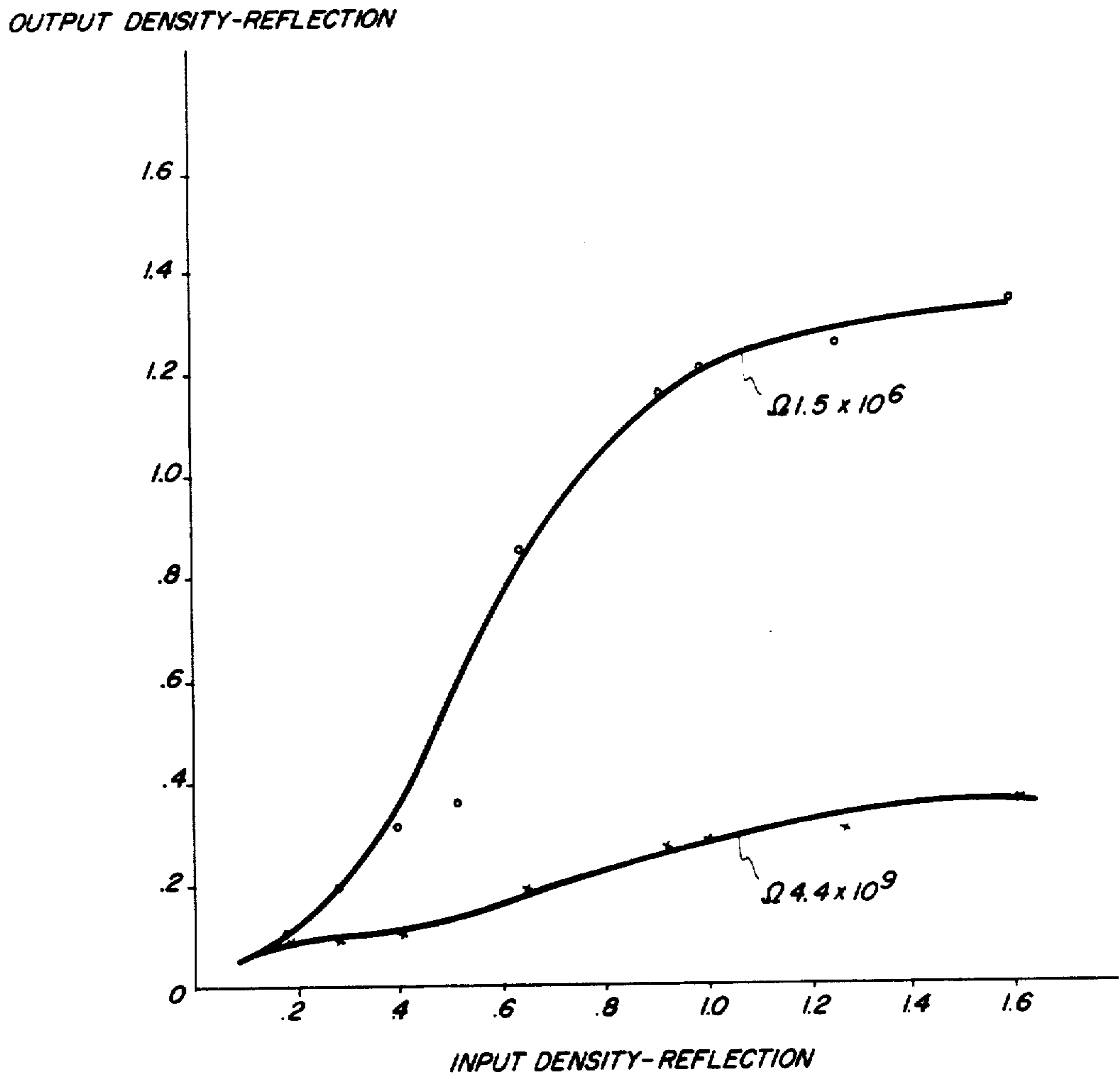
EFFECT OF DEVELOPER CONDUCTIVITY ON SYSTEM H&D
