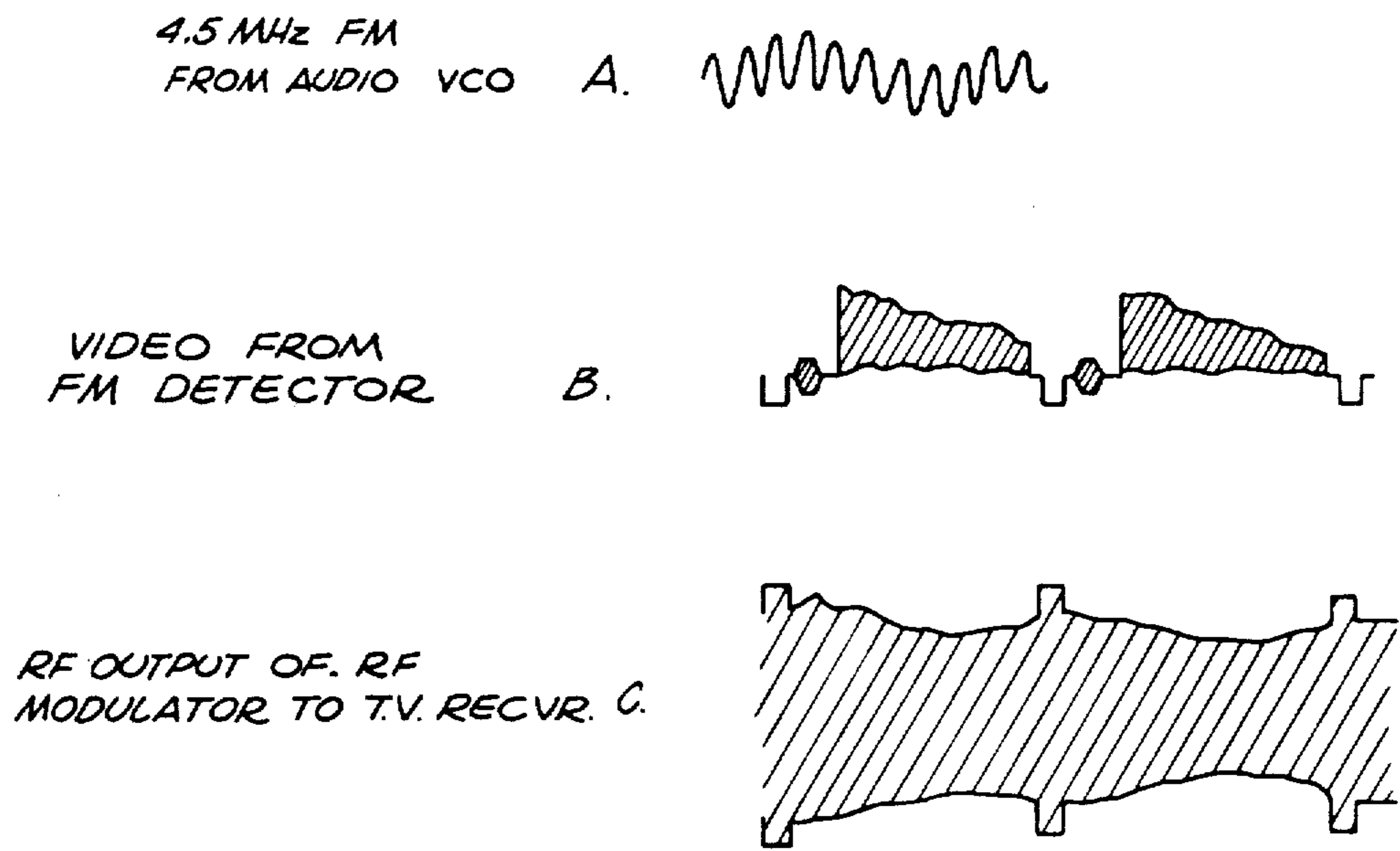
FIG. 25 RF MODULATOR
