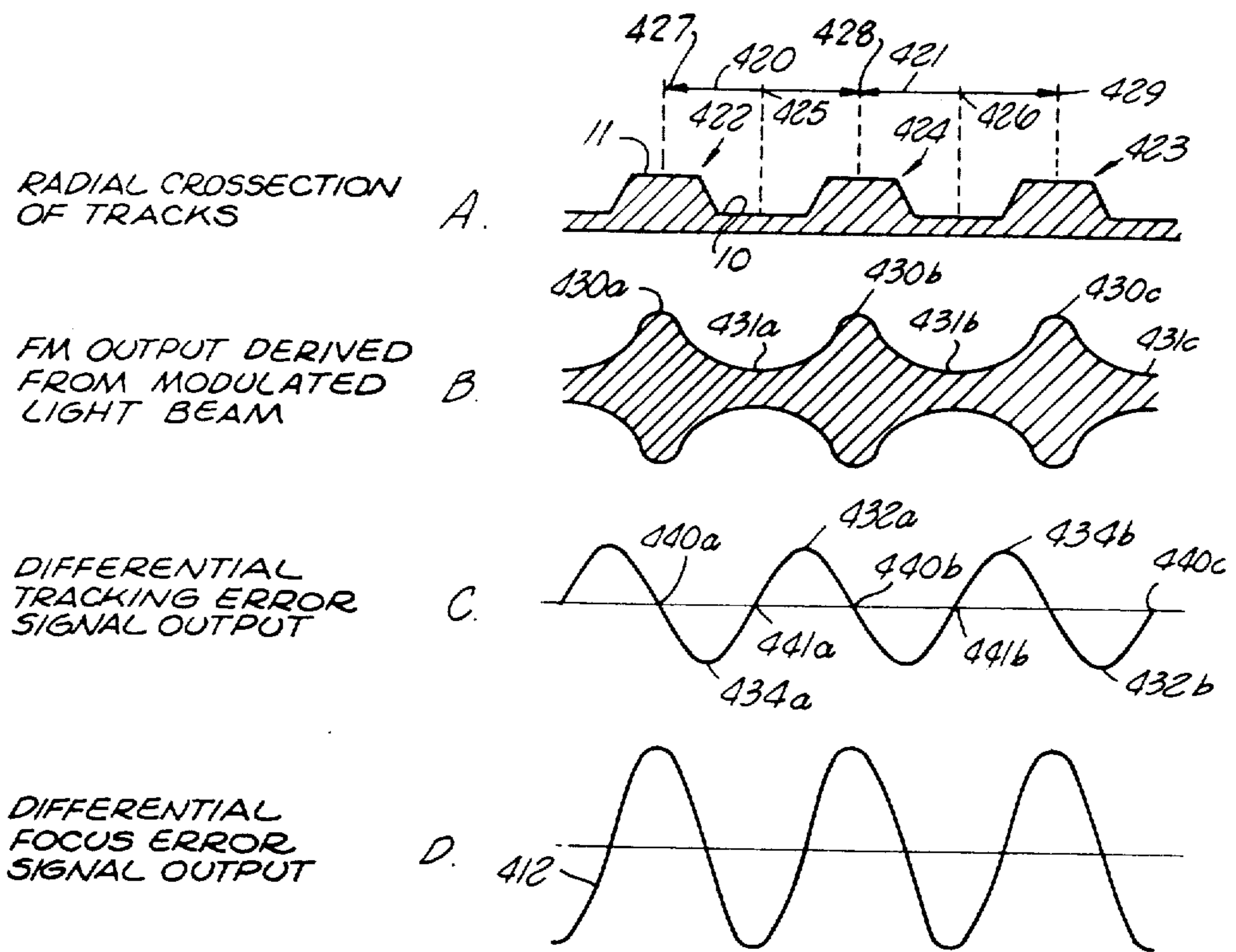
FIG. 8 SIGNAL RECOVERY
