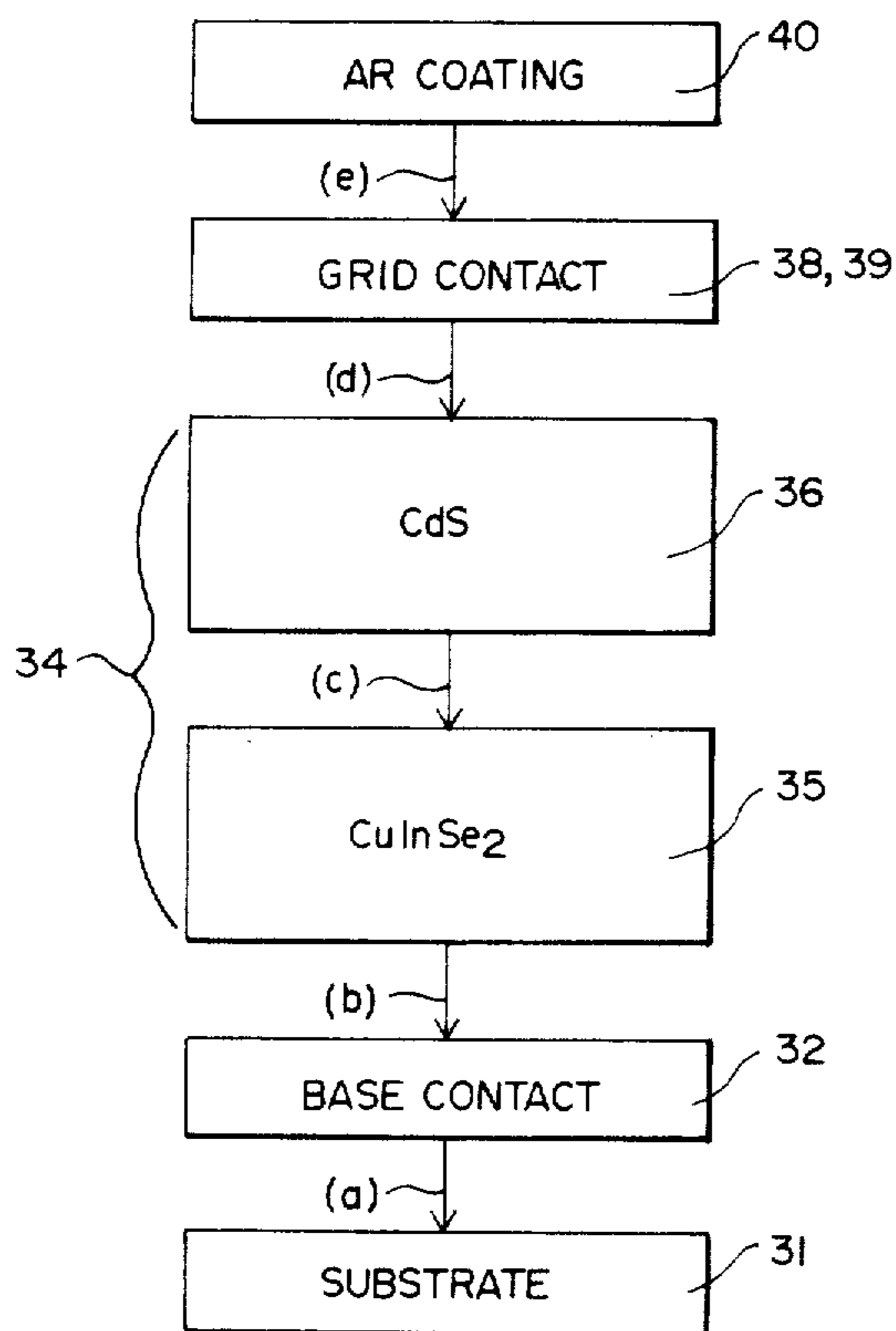
FIG. 3 PRIOR ART
