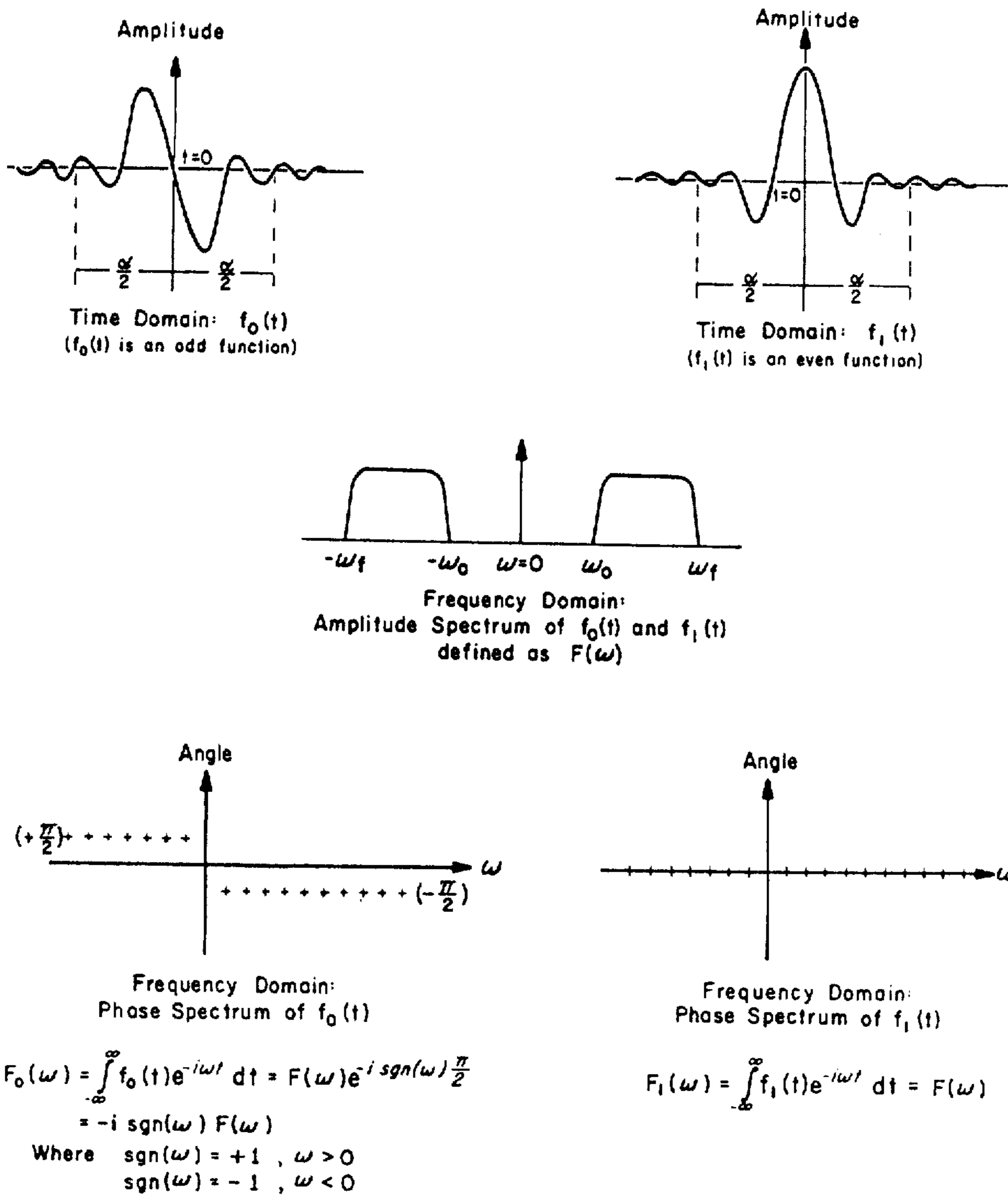
TIME DOMAIN AND COMPLEX FREQUENCY DOMAIN (IN POLAR FORM) REPRESENTATIONS OF THE FUNCTION PAIR f_0(t), f_1(t)
