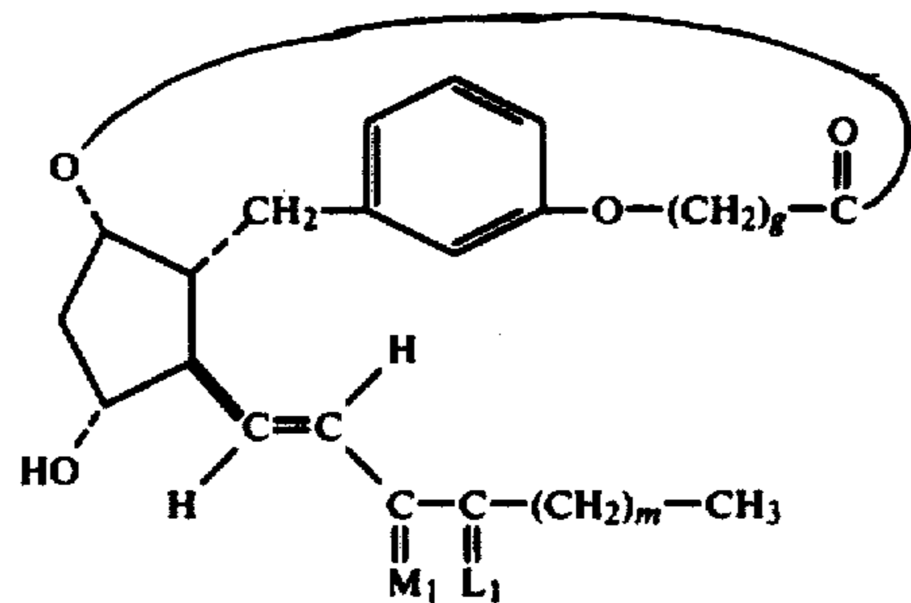
3,7-inter-m-phenylene-3-oxa-4,5,6-trinor-PGF 1α - type, 1,9-lactones
