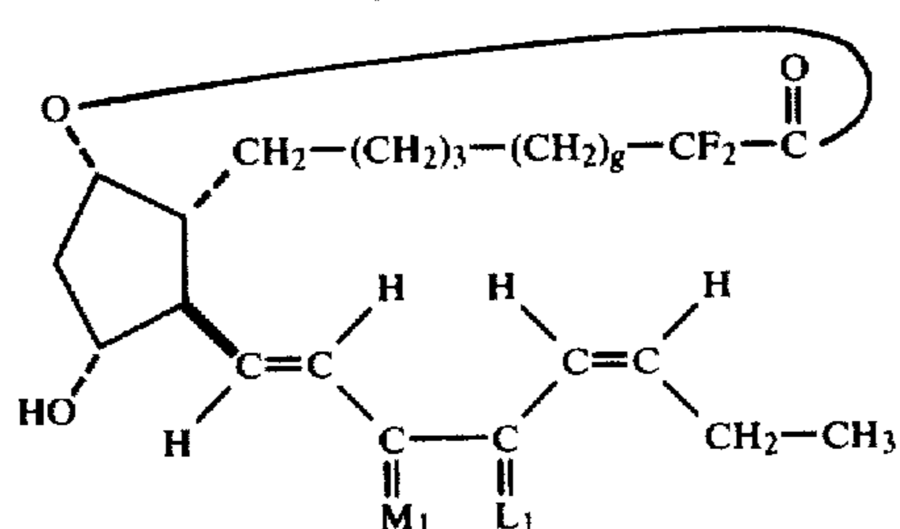
2,2-difluoro-5,6-dihydro-PGF 3α -type, 1,9-lactones
