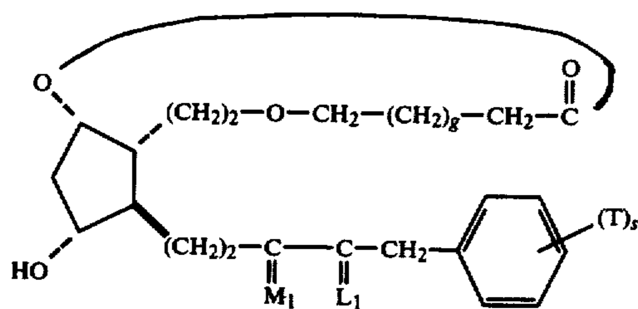
18,19,20-trinor-5-oxa-13,14-dihydro-PGF 1α - type, 1,9-lactones
