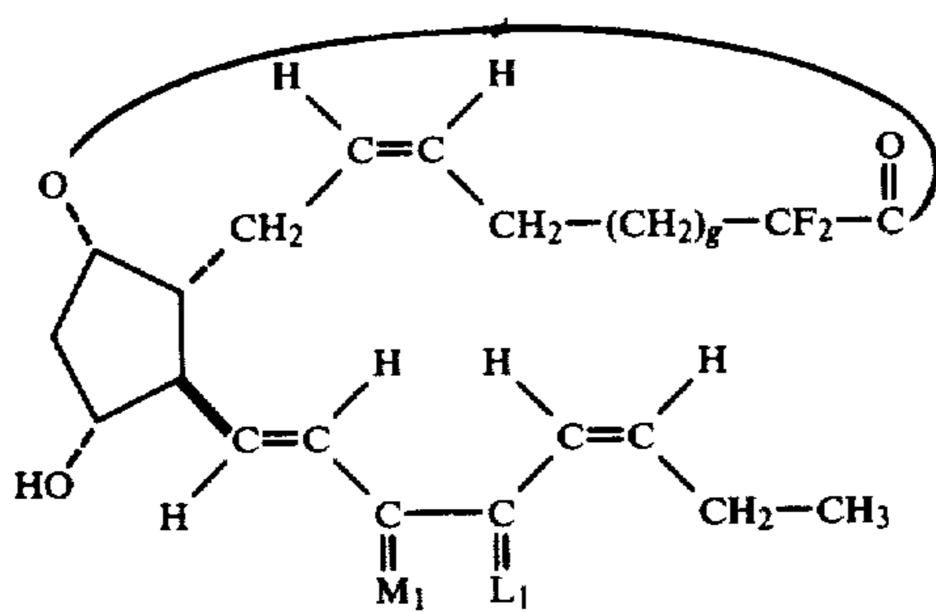
2,2-difluoro-PGF 3α -type, 1,9-lactones
