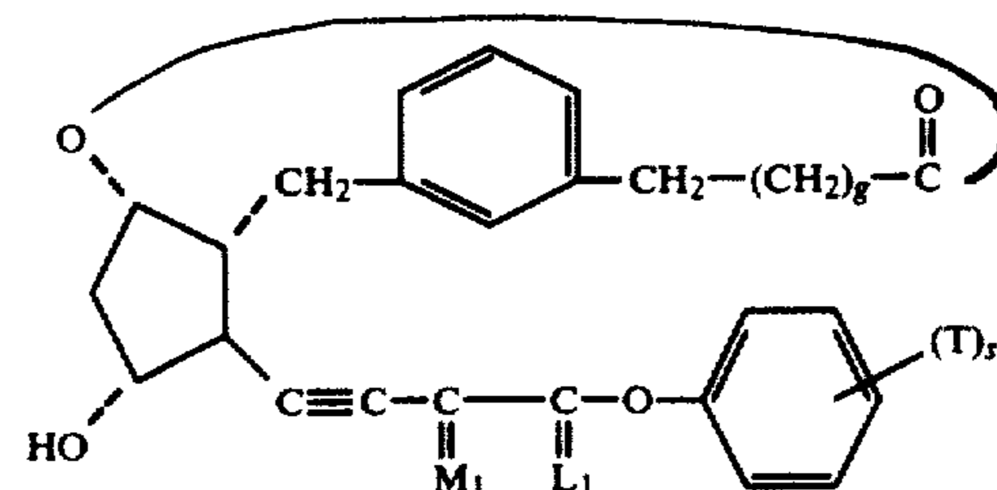
13,14-didehydro-3,7-inter-m-phenylene-4,5,6-trinor-PGF 1α -type, 1,9-lactones
