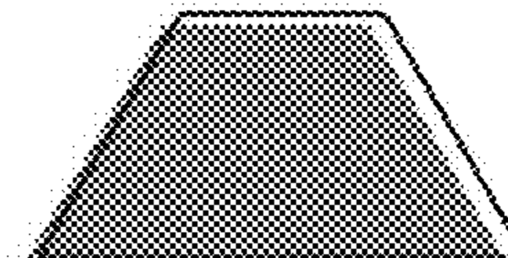
TRAPEZOID
