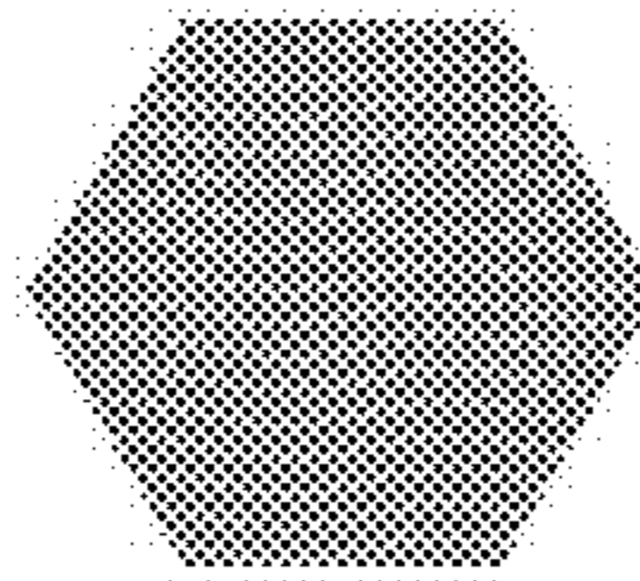
HEXAGON
