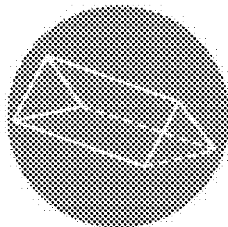
TRIANGULAR PRISM
