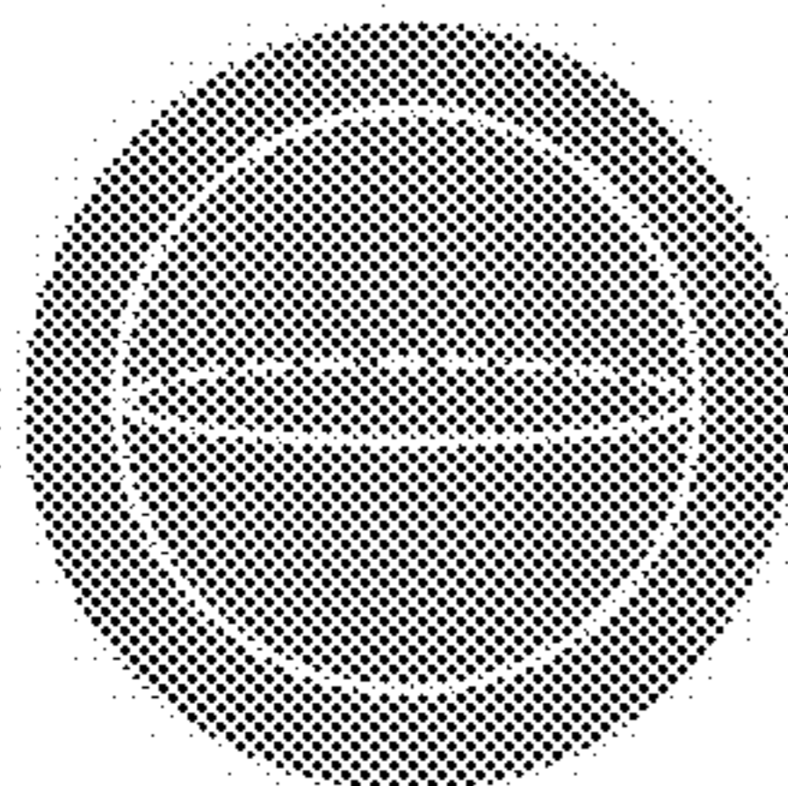
SPHERE
