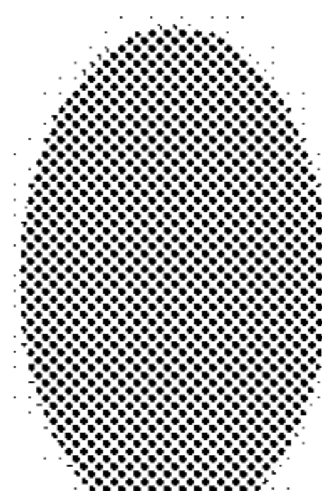
OVAL
