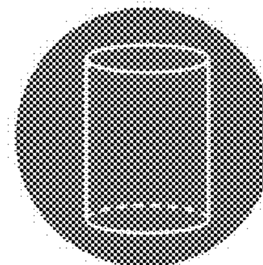
CYLINDER
