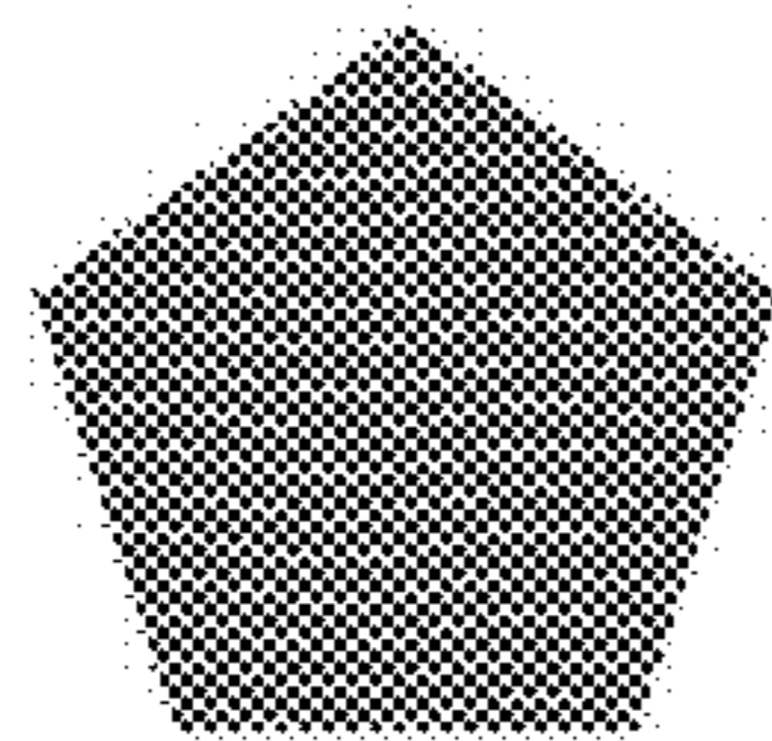
PENTAGON
