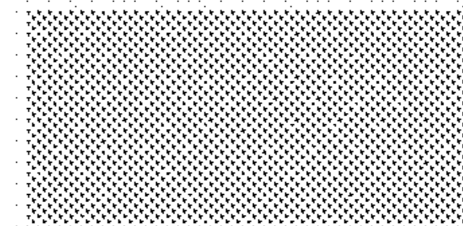
RECTANGLE
