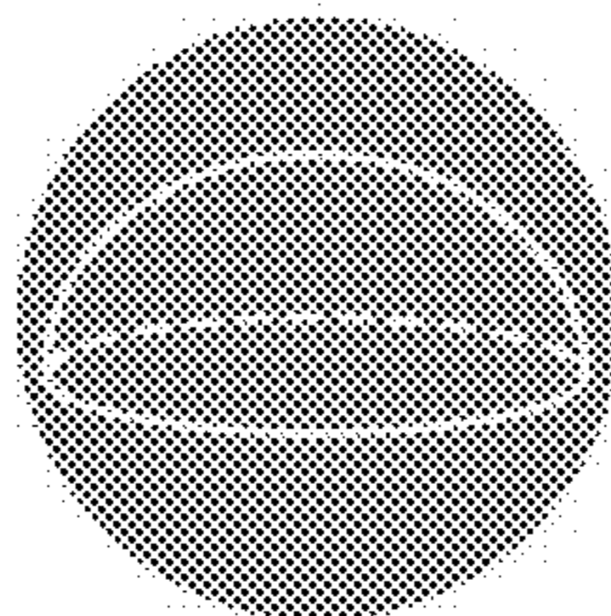
HEMISPHERE
