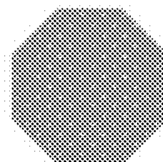
OCTAGON
