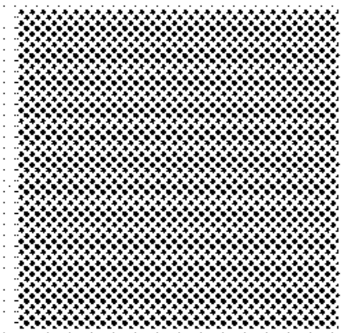
SQUARE
