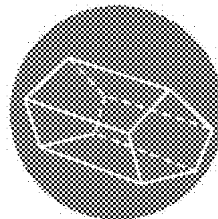
PENTAGONAL PRISM
