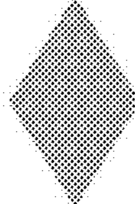
DIAMOND
