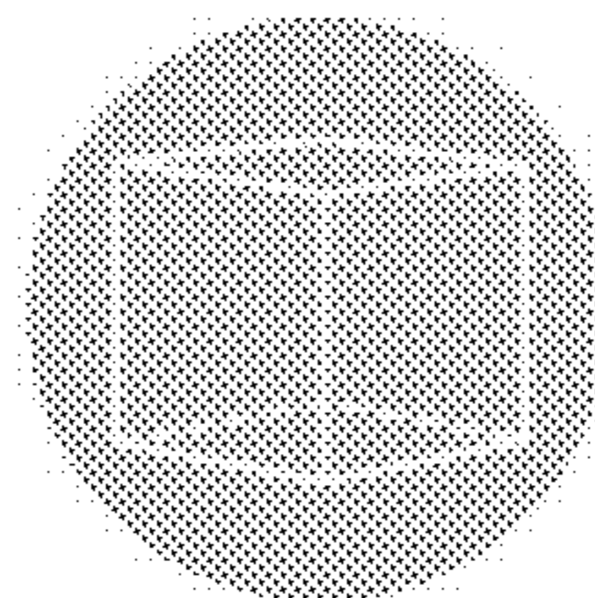
CUBE
