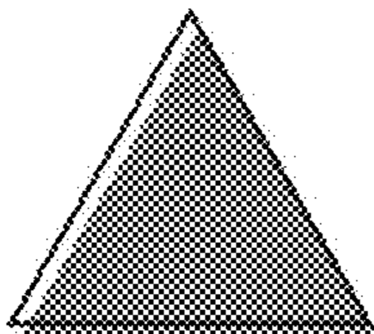
TRIANGLE
