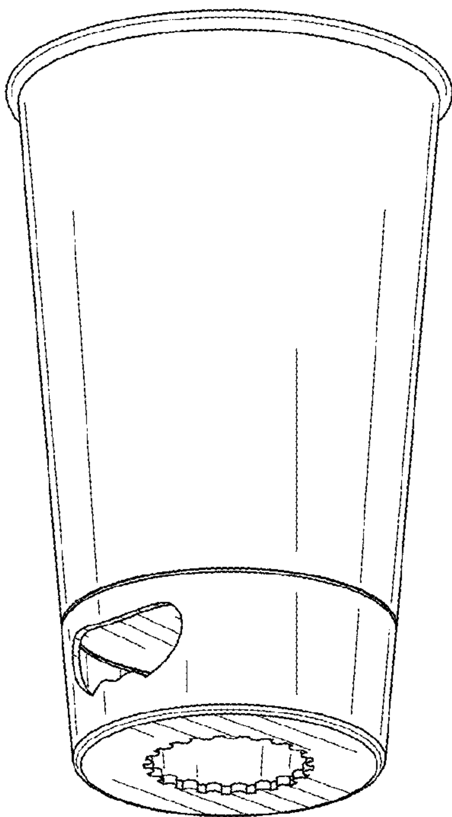
FIG.2 PERSPECTIVE VIEW
