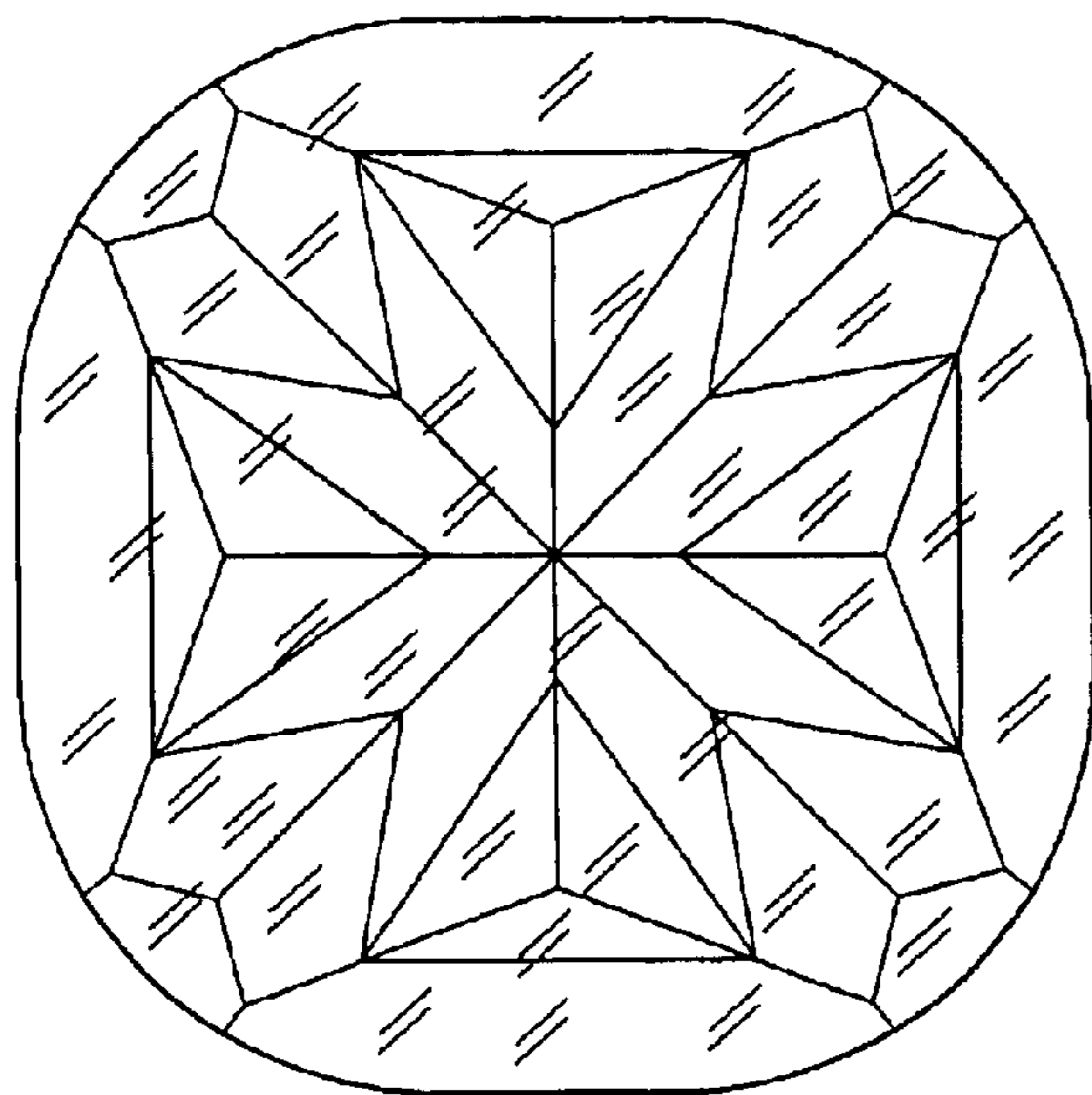
BOTTOM VIEW
