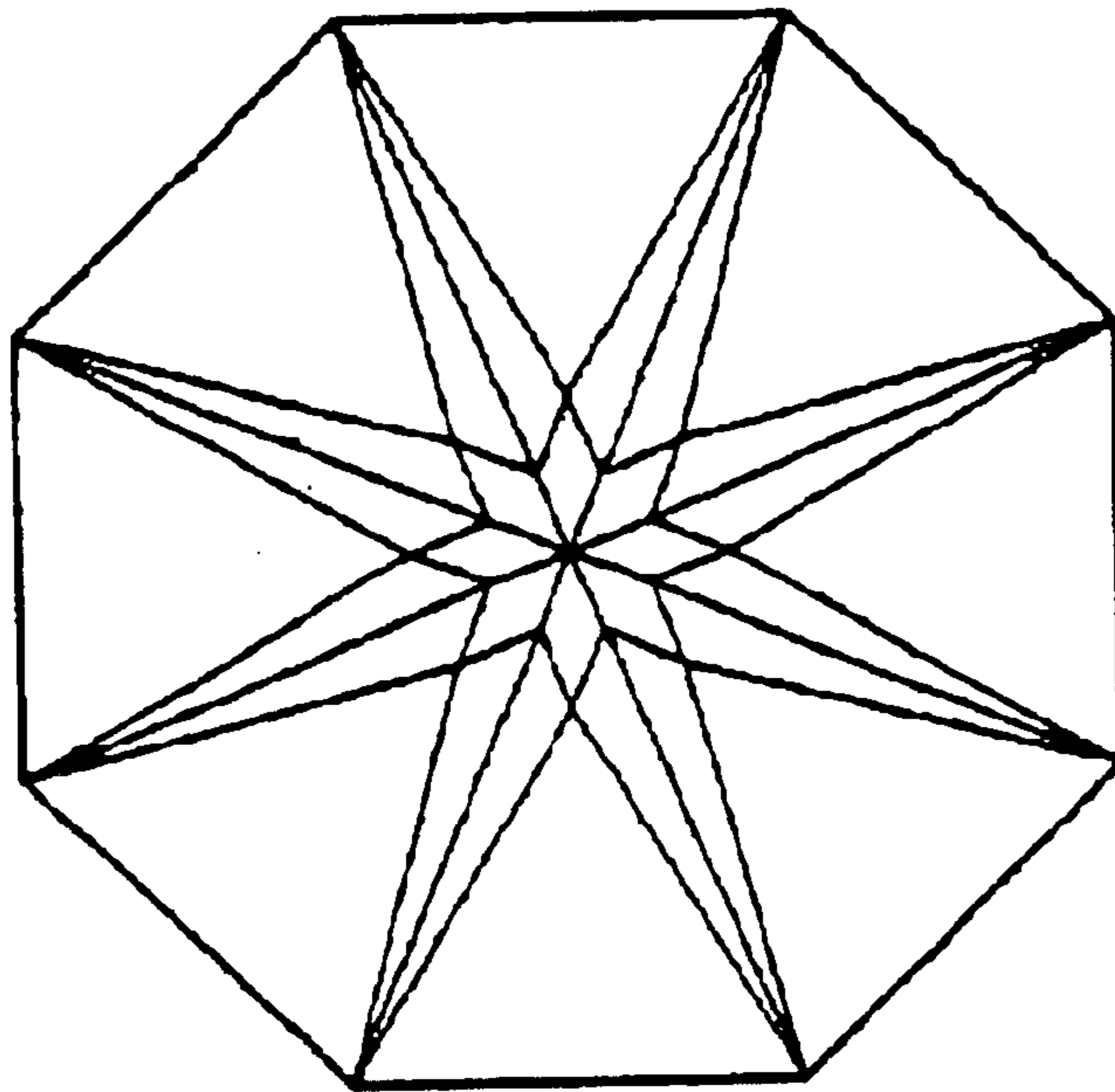
FIG. 3 BOTTOM VIEW
